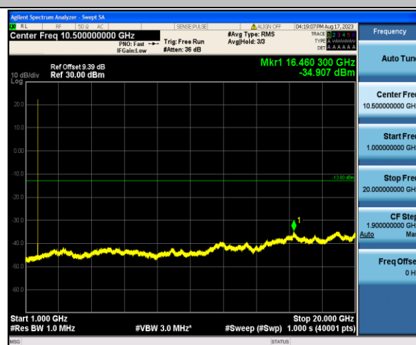
Band4_1.4MHz_16QAM_19957_1RB#0_1000~20000_1000~200
