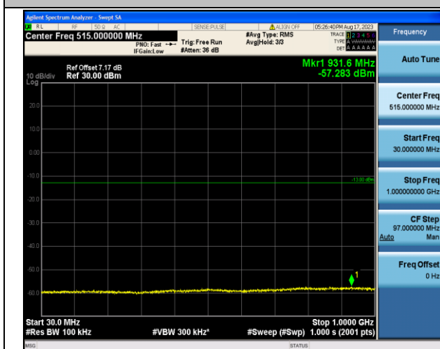
Band4_15MHz_QPSK_20325_1RB#0_30~1000_30~1000
