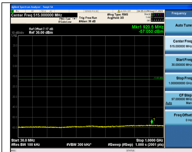
Band4_3MHz_16QAM_20175_1RB#0_30~1000_30~1000
