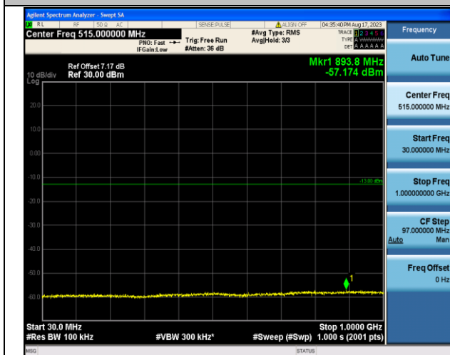
Band4_3MHz_QPSK_20385_1RB#0_30~1000_30~1000
