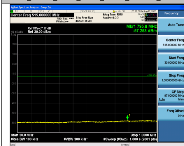
Band4_15MHz_16QAM_20325_1RB#0_30~1000_30~100
