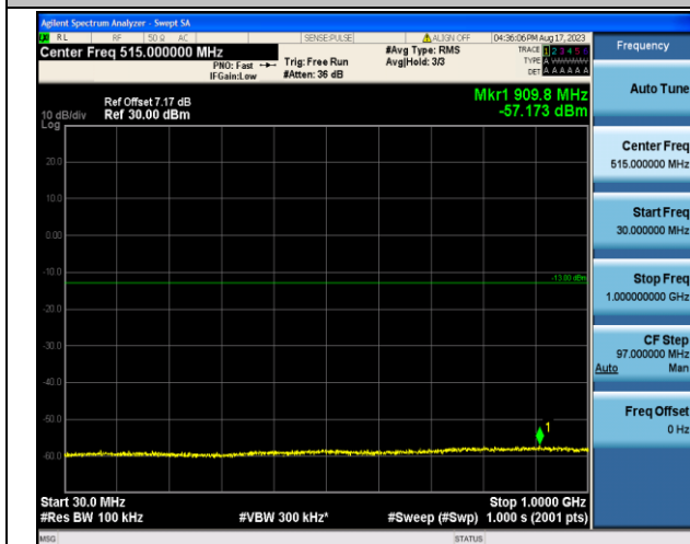
Band4_3MHz_16QAM_20385_1RB#0_30~1000_30~1000
