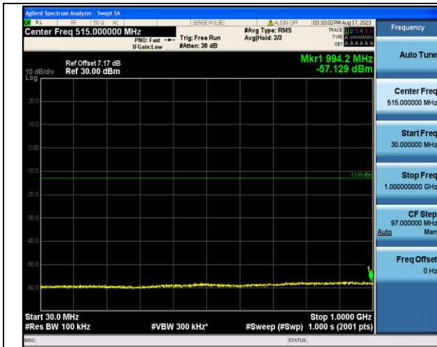
Band2_3MHz_16QAM_18900_1RB#0_30~1000_30~1000
