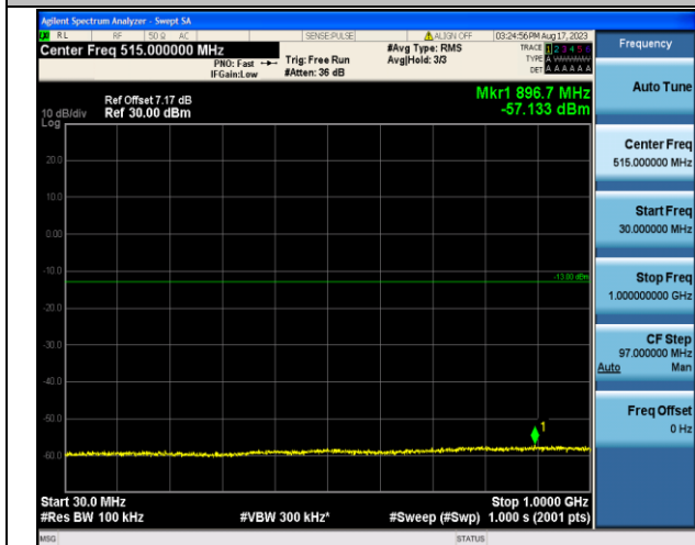
Band2_5MHz_16QAM_18625_1RB#0_30~1000_30~1000
