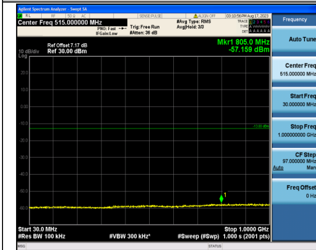
Band2_3MHz_16QAM_19185_1RB#0_30~1000_30~1000
