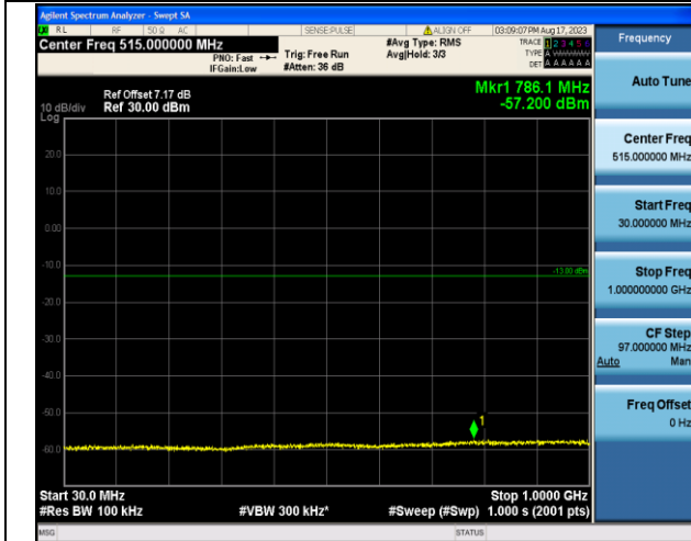
Band2_3MHz_16QAM_18615_1RB#0_30~1000_30~1000
