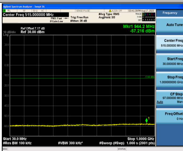
Band2_10MHz_QPSK_19150_1RB#0_30~1000_30~1000
