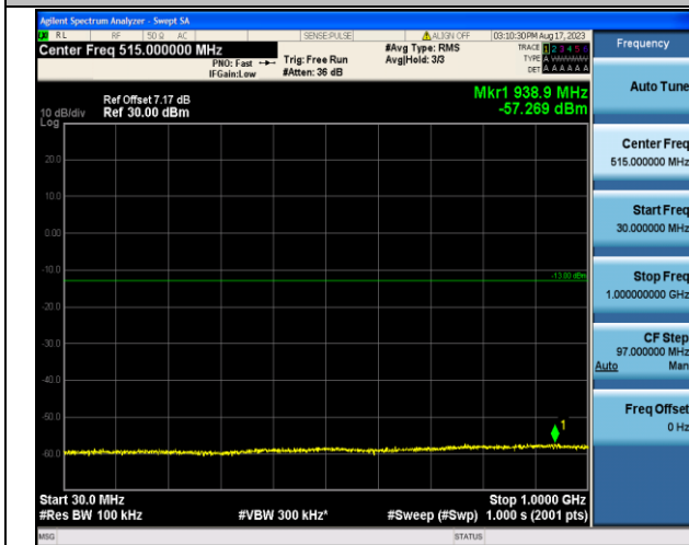
Band2_3MHz_QPSK_19185_1RB#0_30~1000_30~1000
