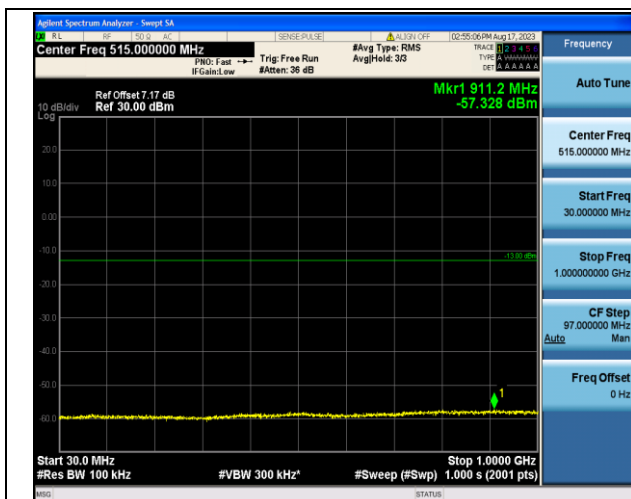
Band2_1.4MHz_16QAM_18900_1RB#0_30~1000_30~1000 00
