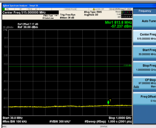
Band2_10MHz_16QAM_19150_1RB#0_30~1000_30~100
