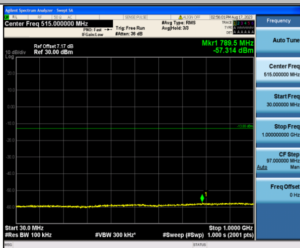
Band2_1.4MHz_16QAM_19193_1RB#0_30~1000_30~1000 00
