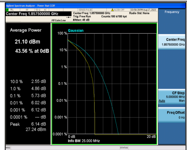
Band2-15MHz-QPSK-18675-75RB#0-PASS
