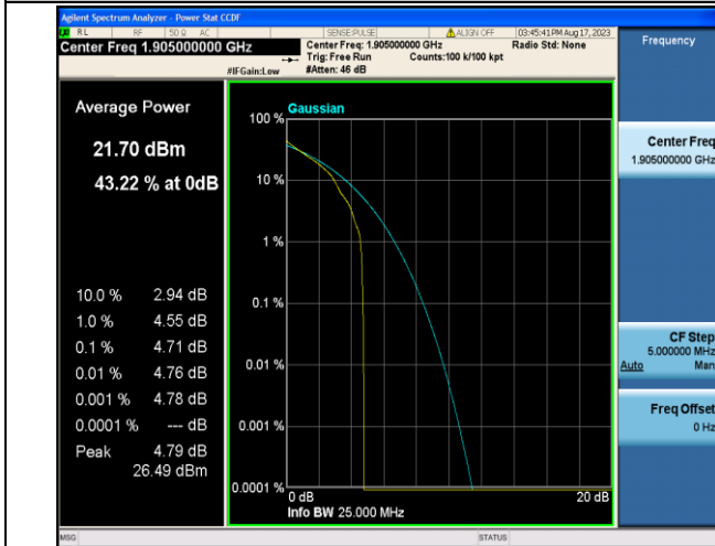
Band2-10MHz-QPSK-19150-1RB#0-PASS
