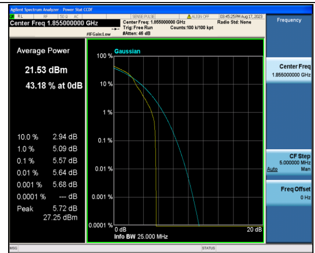
Band2-10MHz-16QAM-18650-1RB#0-PASS
