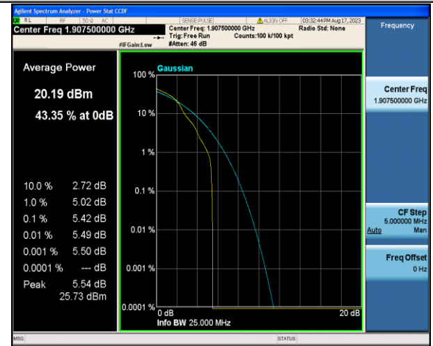
Band2-5MHz-16QAM-19175-1RB#0-PASS
