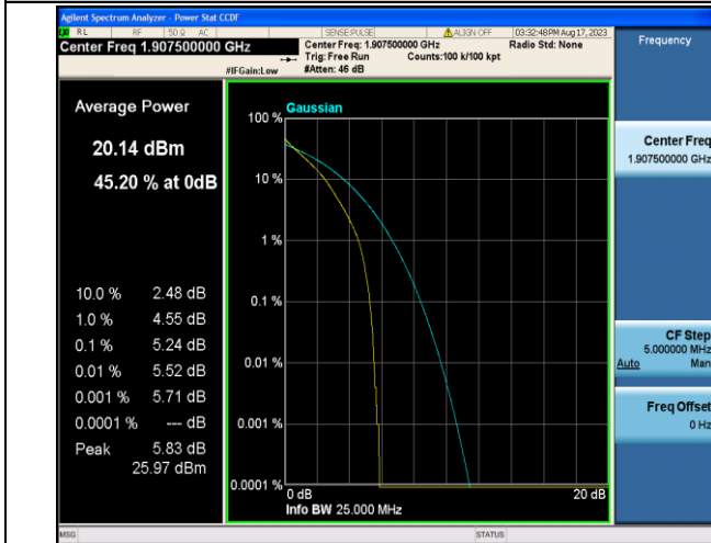
Band2-5MHz-QPSK-19175-25RB#0-PASS
