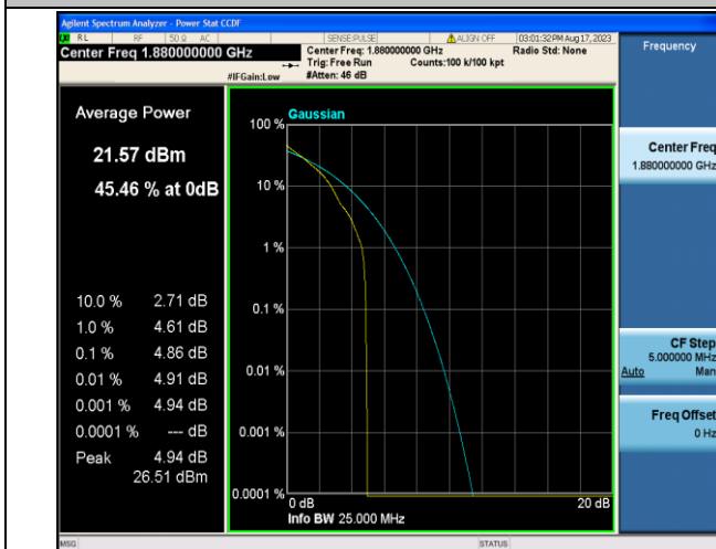
Band2-1.4MHz-QPSK-18900-1RB#0-PASS
