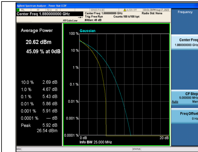
Band2-1.4MHz-QPSK-18900-6RB#0-PASS
