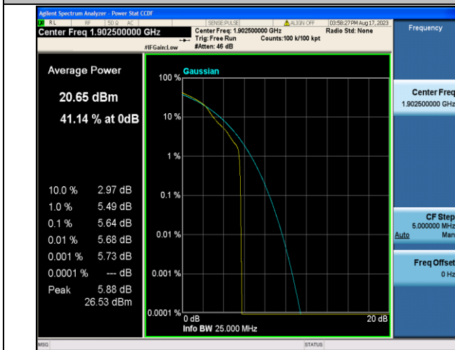
Band2-15MHz-16QAM-19125-1RB#0-PASS
