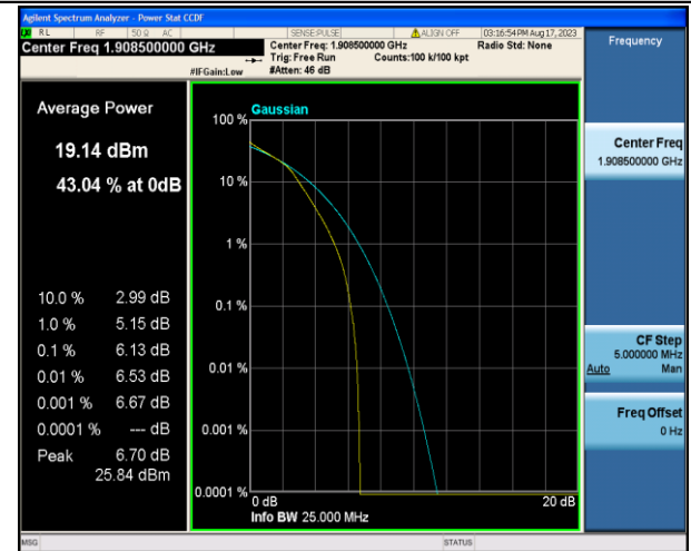
Band2-3MHz-16QAM-19185-15RB#0-PASS
