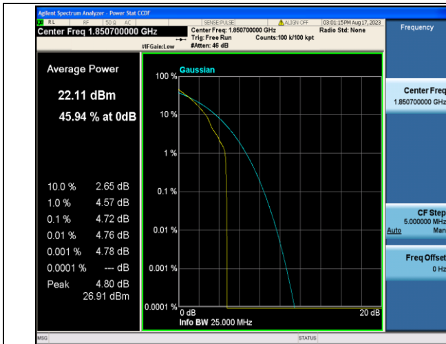
Band2-1.4MHz-QPSK-18607-1RB#0-PASS
