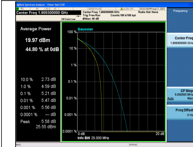
Band2-1.4MHz-QPSK-19193-6RB#0-PASS
