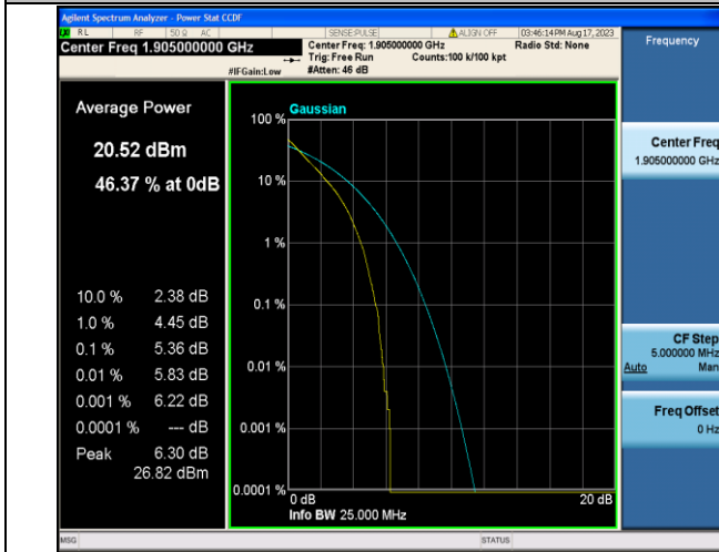
Band2-10MHz-QPSK-19150-50RB#0-PASS
