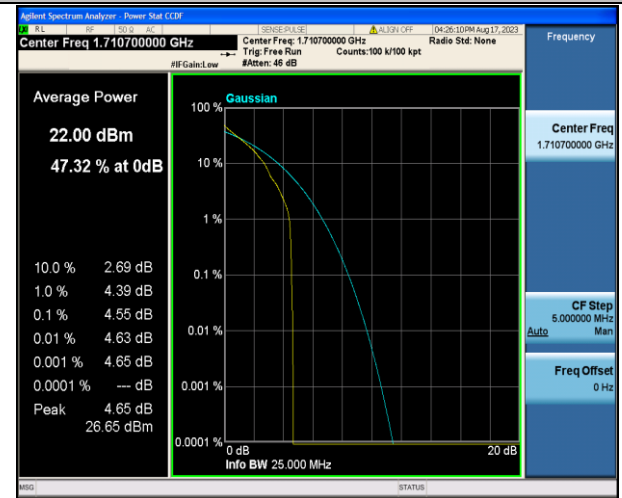
Band4-1.4MHz-QPSK-19957-1RB#0-PASS
