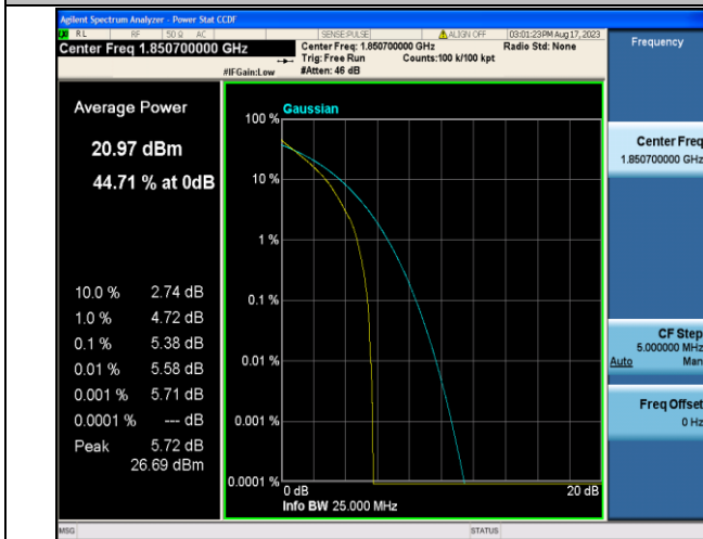
Band2-1.4MHz-QPSK-18607-6RB#0-PASS
