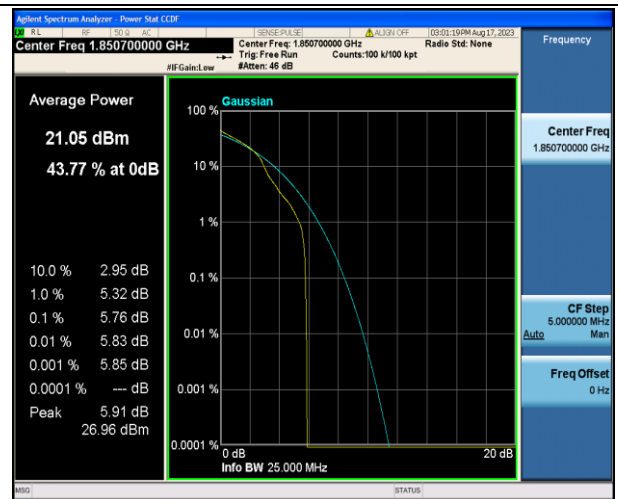
Band2-1.4MHz-16QAM-18607-1RB#0-PASS
