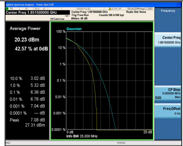
Band2-3MHz-16QAM-18615-15RB#0-PASS
