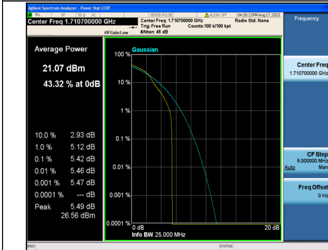
Band4-1.4MHz-16QAM-19957-1RB#0-PASS
