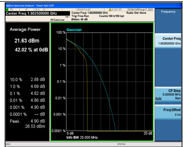
Band2-15MHz-QPSK-19125-1RB#0-PASS
