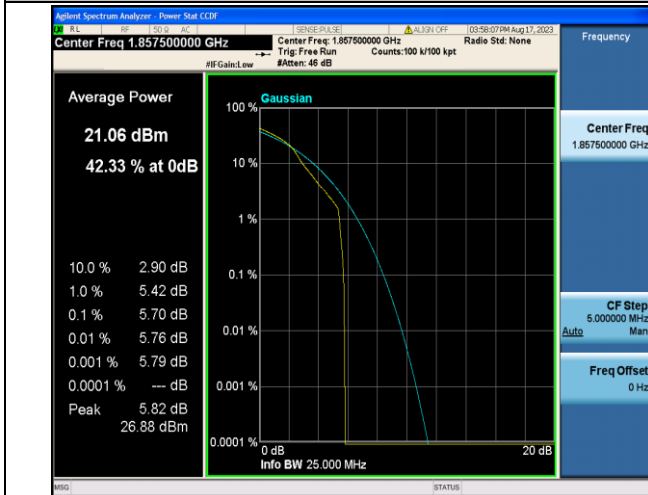
Band2-15MHz-16QAM-18675-1RB#0-PASS
