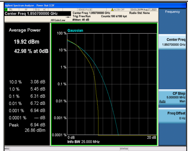
Band2-1.4MHz-16QAM-18607-6RB#0-PASS
