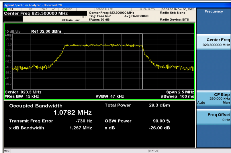
Band26-1.4MHz-16QAM-26783-6RB#0-1.0782
