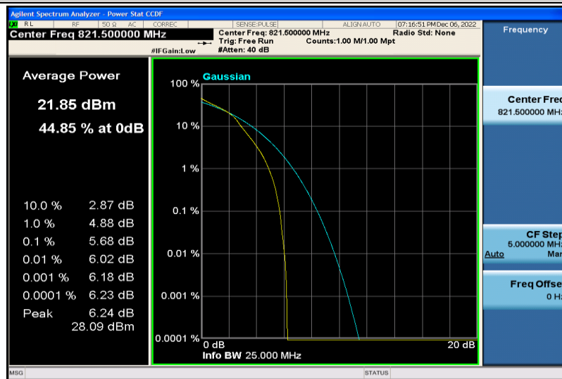
Band26-15MHz-16QAM-26765-25RB#0
