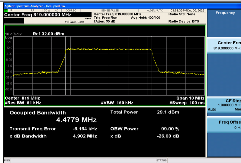
Band26-5MHz-QPSK-26740-25RB#0-4.4779
