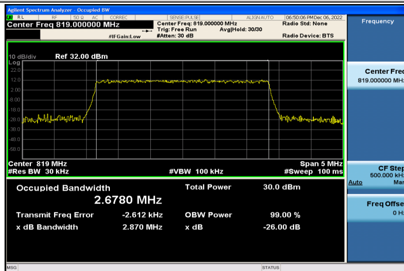
Band26-3MHz-16QAM-26740-15RB#0-2.6780
