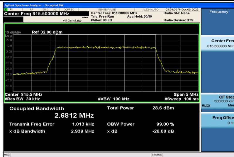
Band26-3MHz-QPSK-26705-15RB#0-2.6812
