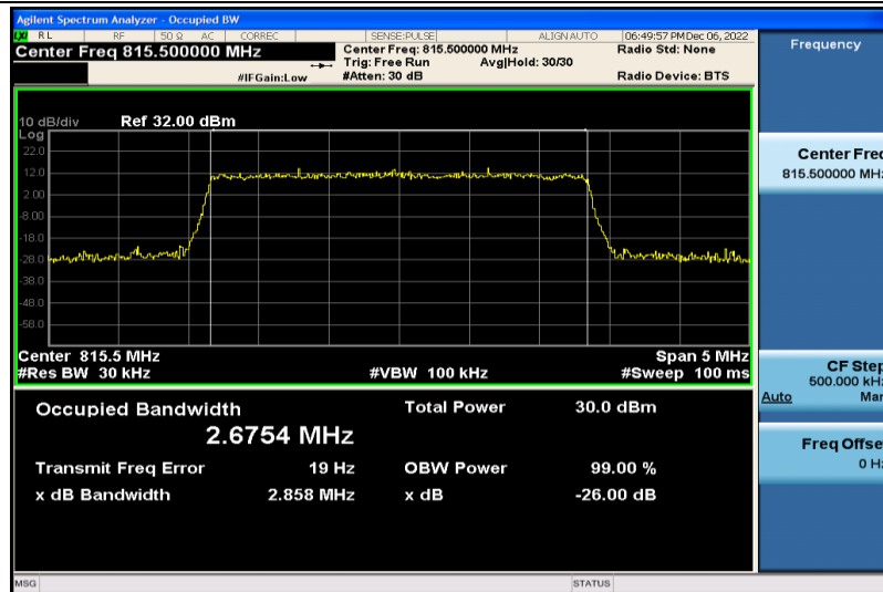
Band26-3MHz-16QAM-26705-15RB#0-2.6754
