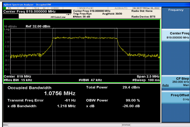
Band26-1.4MHz-16QAM-26740-6RB#0-1.0756
