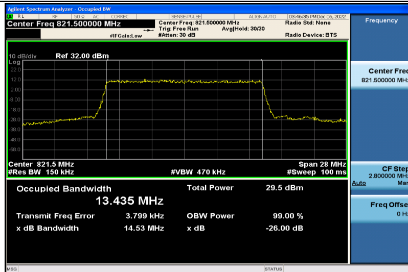
Band26-15MHz-QPSK-26765-75RB#0-13.435
