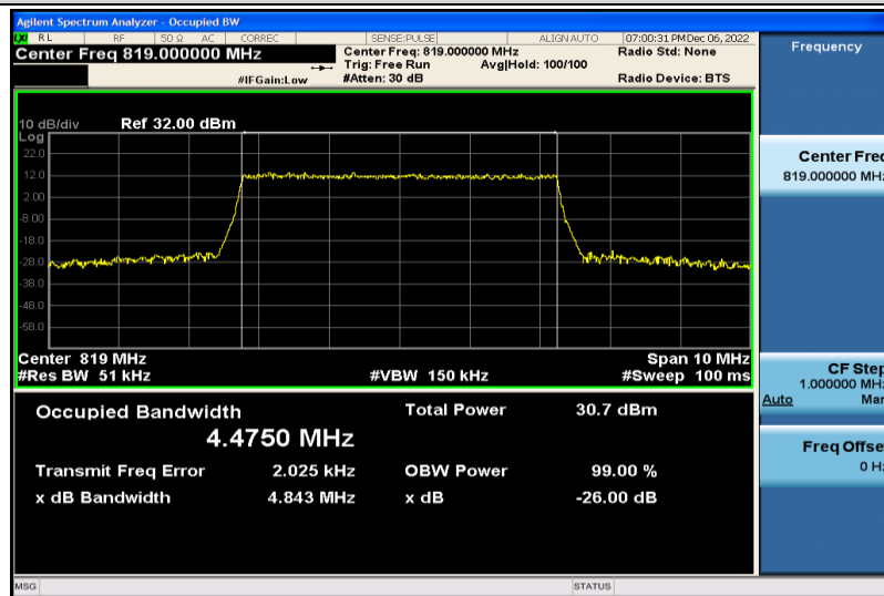
Band26-5MHz-16QAM-26740-25RB#0-4.4750
