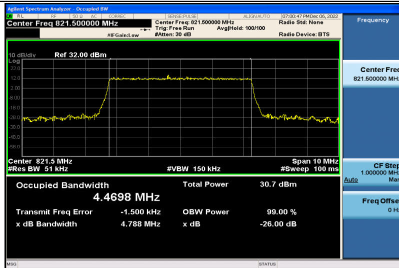
Band26-5MHz-16QAM-26765-25RB#0-4.4698
