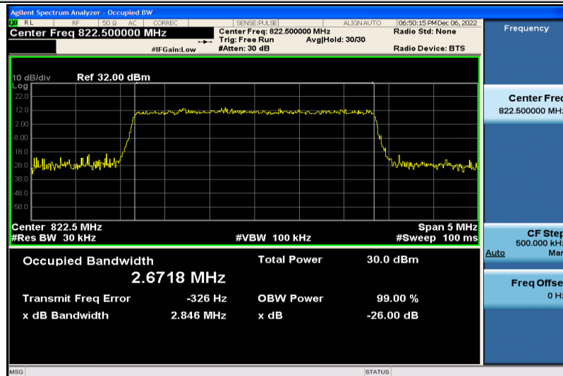
Band26-3MHz-16QAM-26775-15RB#0-2.6718
