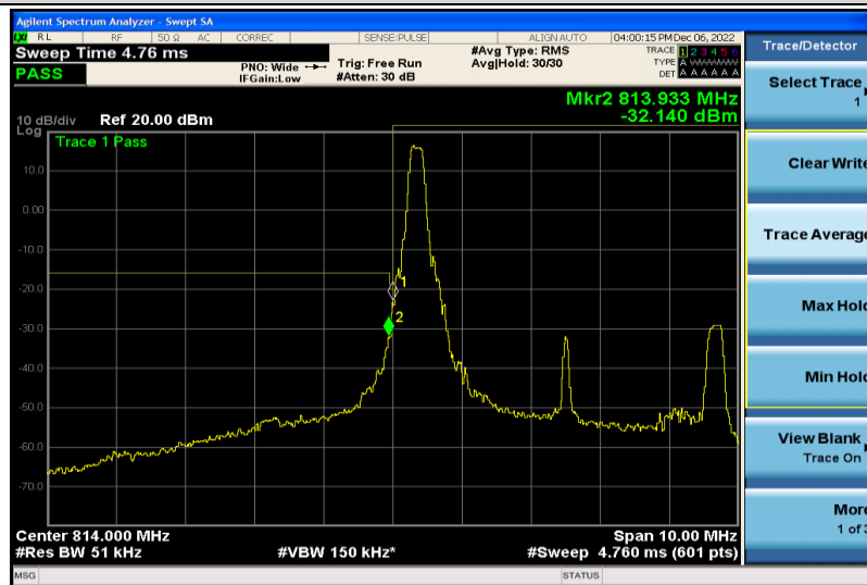
Band26-5MHz-QPSK-26715-1RB#0
