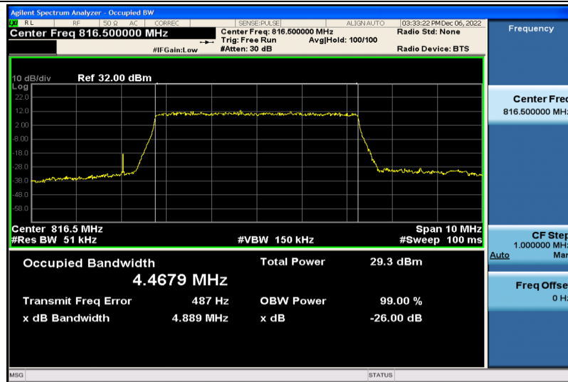
Band26-5MHz-QPSK-26715-25RB#0-4.4679
