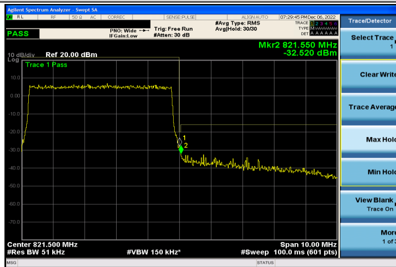
Band26-5MHz-16QAM-26740-25RB#0
