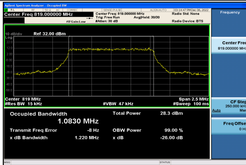
Band26-1.4MHz-QPSK-26740-6RB#0-1.0830
