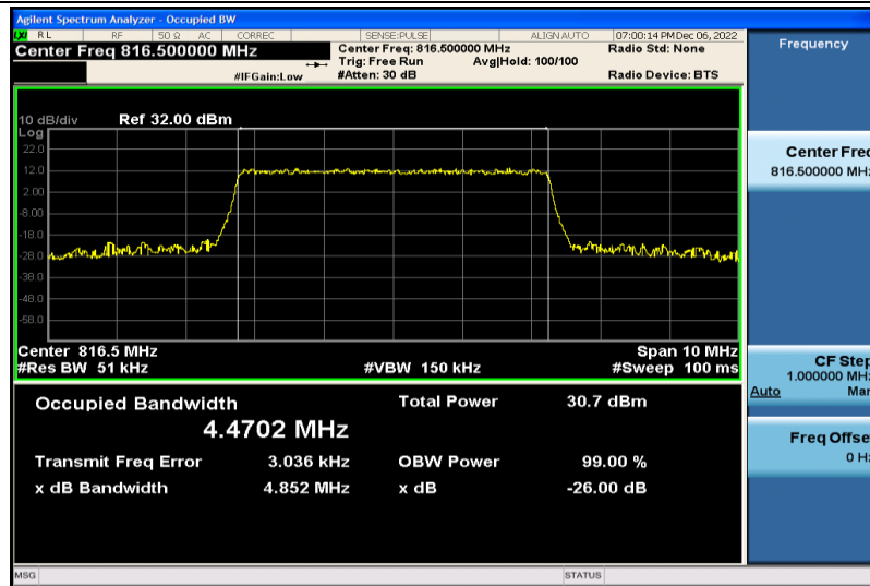
Band26-5MHz-16QAM-26715-25RB#0-4.4702
