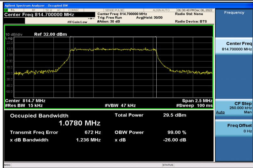
Band26-1.4MHz-16QAM-26697-6RB#0-1.0780
