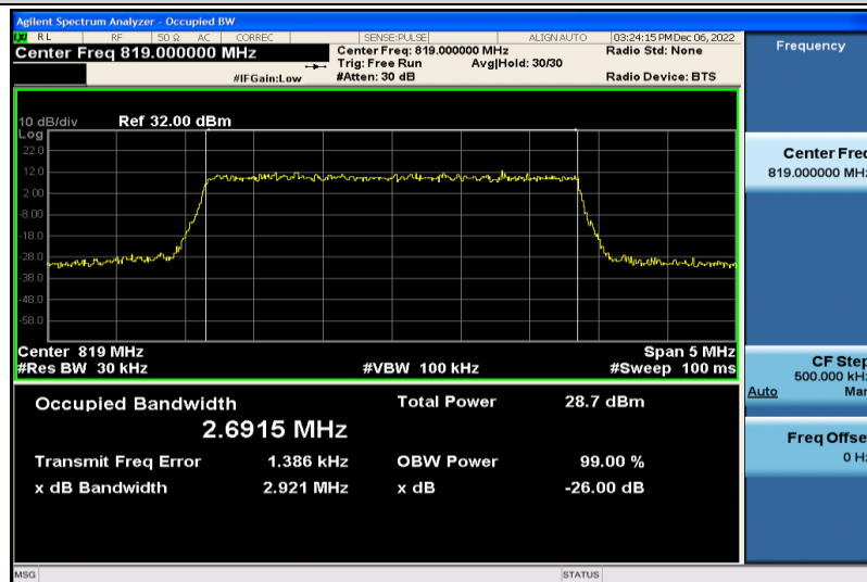
Band26-3MHz-QPSK-26740-15RB#0-2.6915
