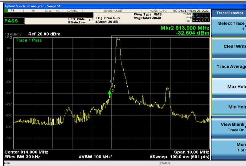
Band26-3MHz-16QAM-26705-1RB#0
