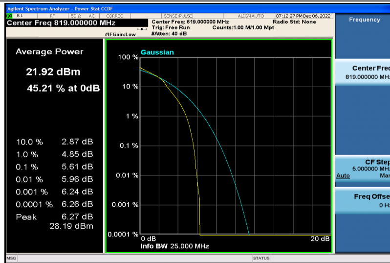
Band26-10MHz-16QAM-26740-25RB#0
