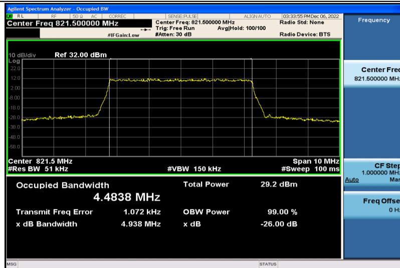
Band26-5MHz-QPSK-26765-25RB#0-4.4838
