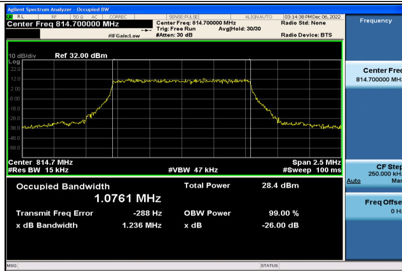
Band26-1.4MHz-QPSK-26697-6RB#0-1.0761
