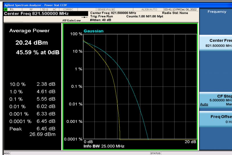
Band26-5MHz-QPSK-26765-25RB#0
