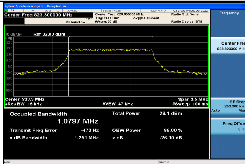
Band26-1.4MHz-QPSK-26783-6RB#0-1.0797
