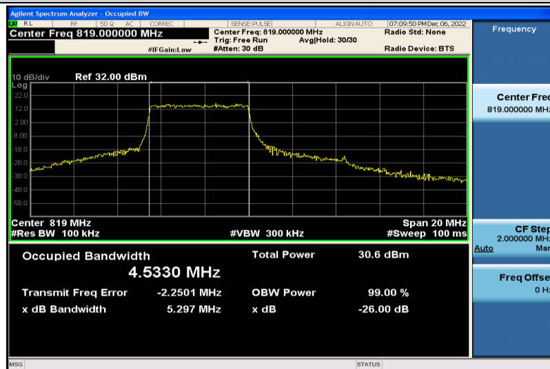
Band26-10MHz-16QAM-26740-25RB#0-4.5330
