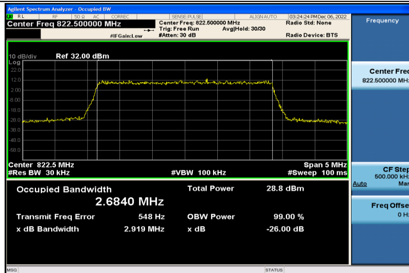
Band26-3MHz-QPSK-26775-15RB#0-2.6840
