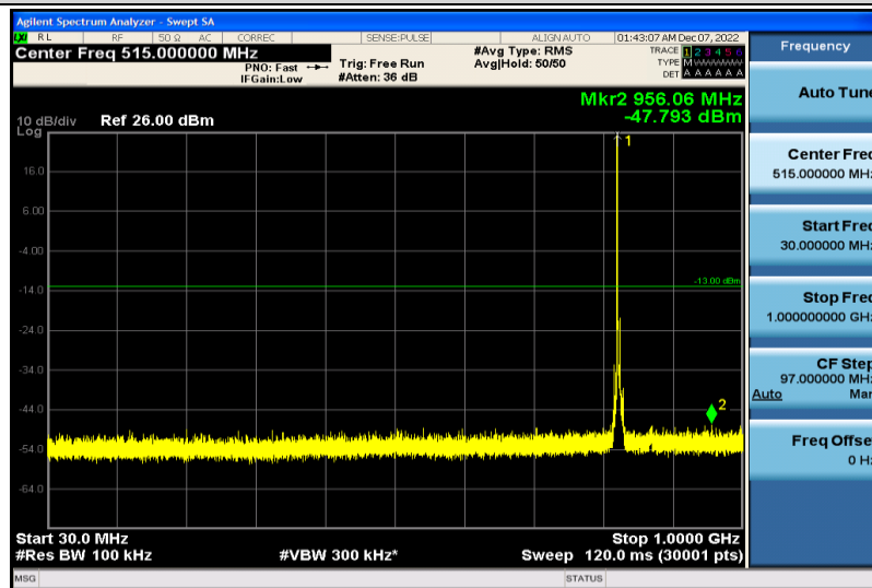
Band26-5MHz-16QAM-26815-1RB#0-30~1000MHz
