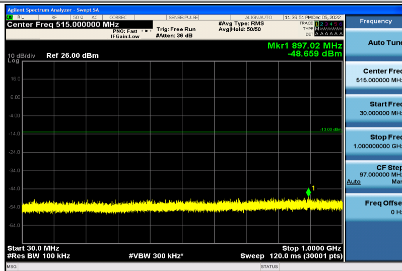
Band25-10MHz-QPSK-26090-1RB#0-30~1000MHz
