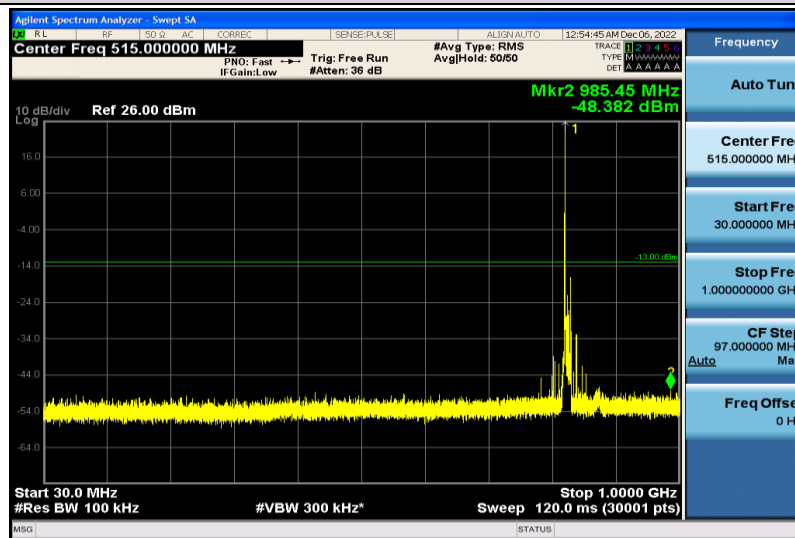
Band26-10MHz-QPSK-26840-1RB#0-30~1000MHz
