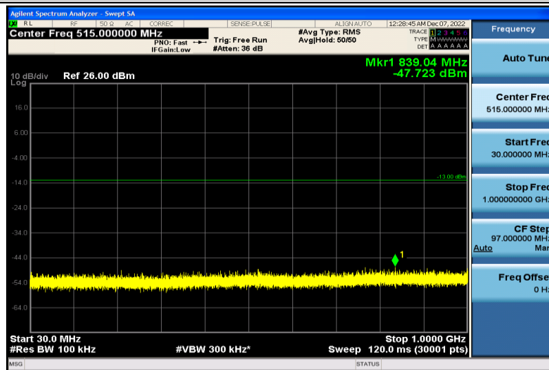
Band25-5MHz-16QAM-26065-1RB#0-30~1000MHz
