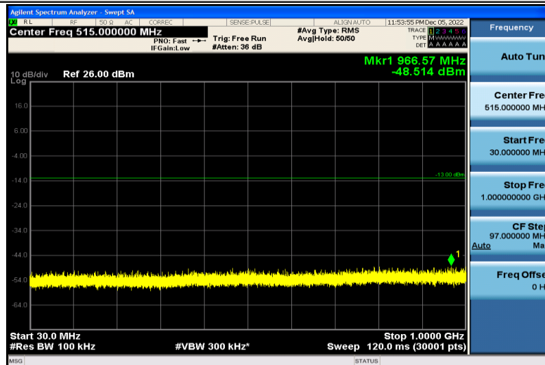
Band25-15MHz-QPSK-26615-1RB#0-30~1000MHz
