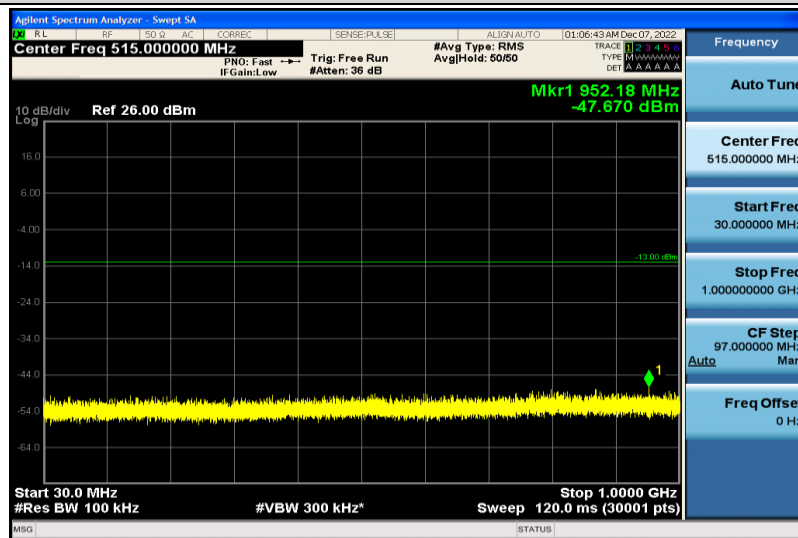
Band25-20MHz-16QAM-26140-1RB#0-30~1000MHz
