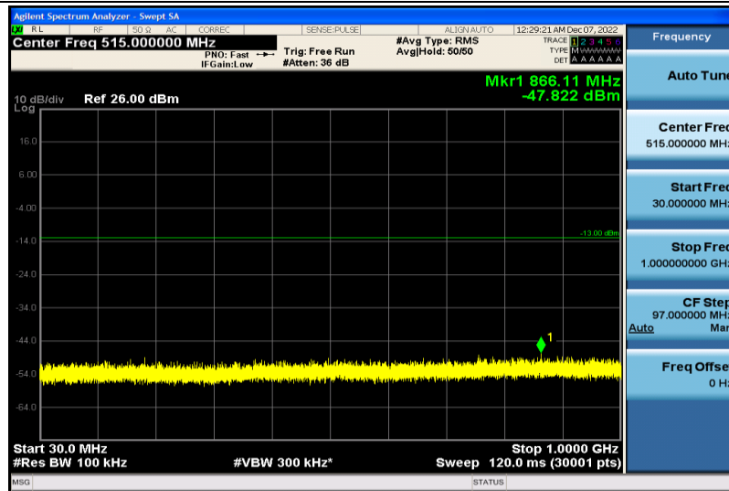
Band25-5MHz-16QAM-26365-1RB#0-30~1000MHz
