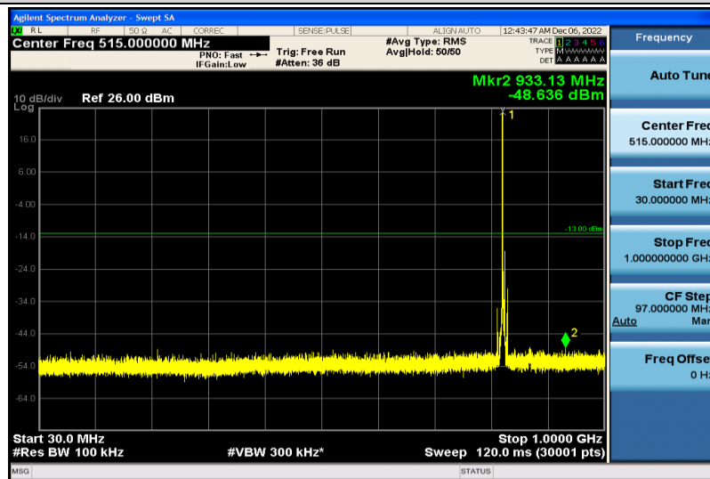
Band26-5MHz-QPSK-26815-1RB#0-30~1000MHz
