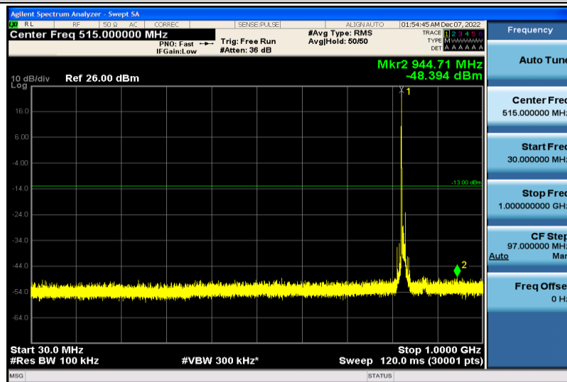
Band26-10MHz-16QAM-26840-1RB#0-30~1000MHz
