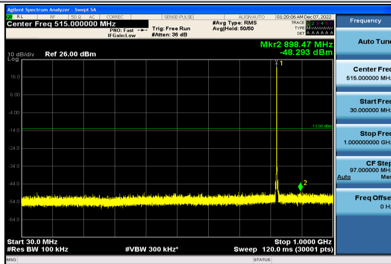
Band26-1.4MHz-16QAM-26797-1RB#0-30~1000MHz
