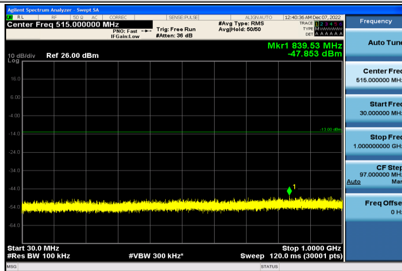
Band25-10MHz-16QAM-26090-1RB#0-30~1000MHz
