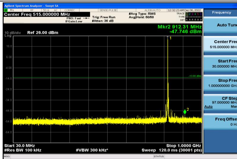
Band26-3MHz-QPSK-26805-1RB#0-30~1000MHz
