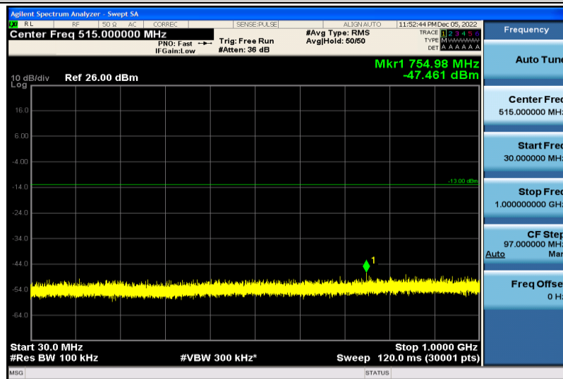
Band25-15MHz-QPSK-26115-1RB#0-30~1000MHz
