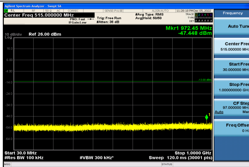
Band25-5MHz-QPSK-26065-1RB#0-30~1000MHz
