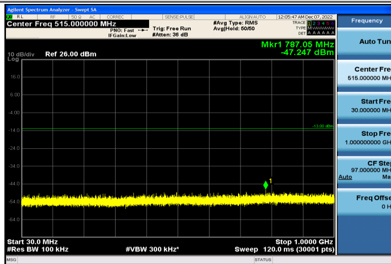
Band25-1.4MHz-16QAM-26047-1RB#0-30~1000MHz
