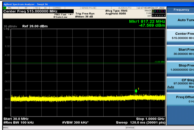
Band25-3MHz-16QAM-26365-1RB#0-30~1000MHz
