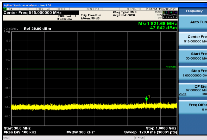
Band25-3MHz-QPSK-26055-1RB#0-30~1000MHz
