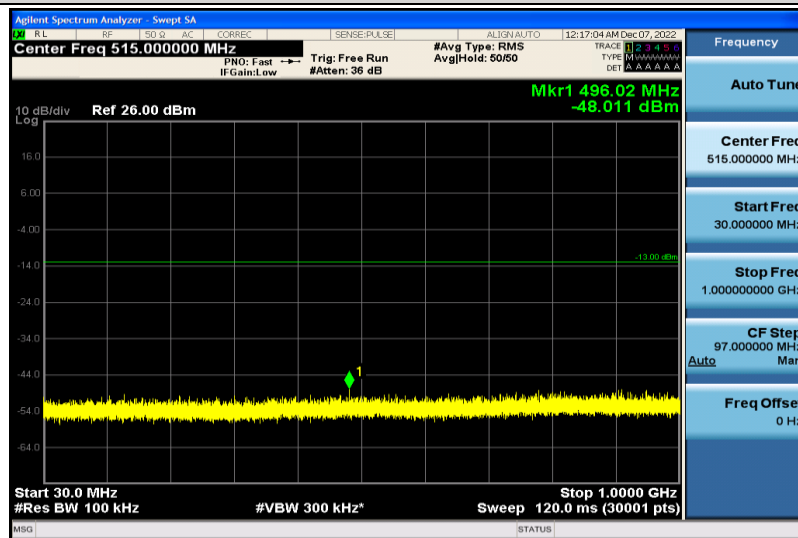
Band25-3MHz-16QAM-26055-1RB#0-30~1000MHz
