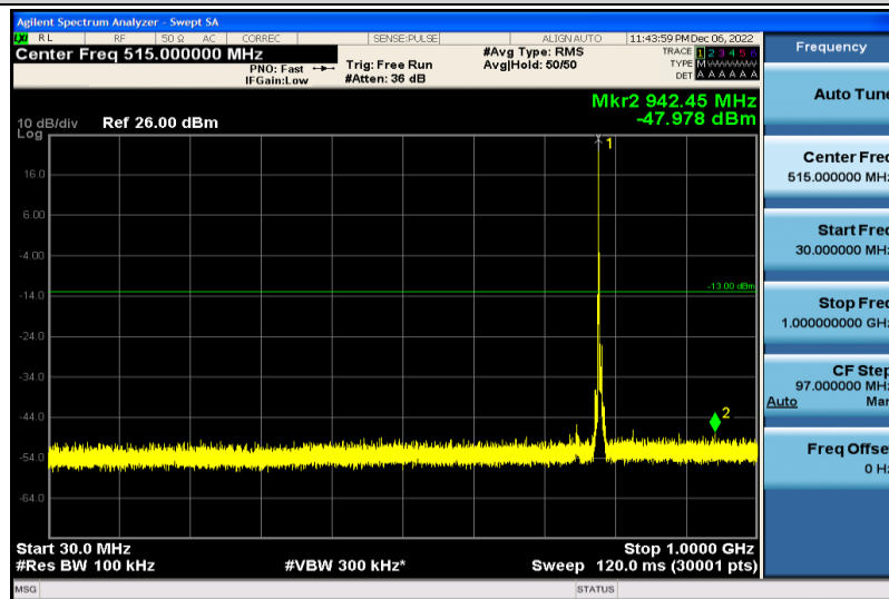
Band13-5MHz-16QAM-23255-1RB#0-30~1000MHz
