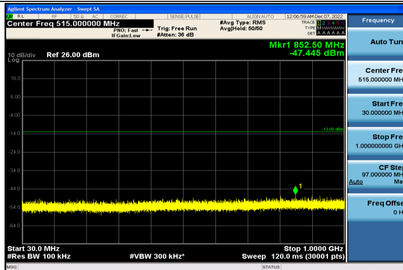
Band25-1.4MHz-16QAM-26683-1RB#0-30~1000MHz
