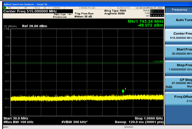
Band25-3MHz-16QAM-26675-1RB#0-30~1000MHz
