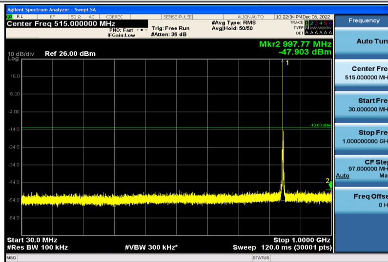
Band5-3MHz-16QAM-20635-1RB#0-30~1000MHz
