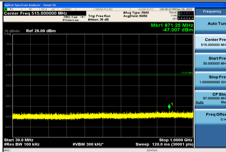
Band4-15MHz-16QAM-20175-1RB#0-30~1000MHz
