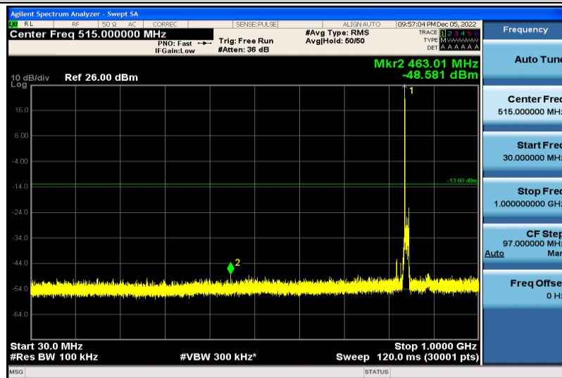
Band5-10MHz-QPSK-20600-1RB#0-30~1000MHz
