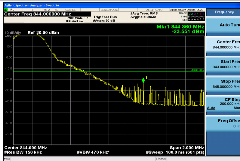
Band26-15MHz-QPSK-26915-1RB#74
