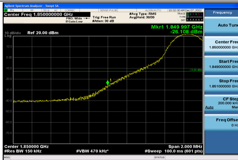
Band25-15MHz-16QAM-26115-1RB#0
