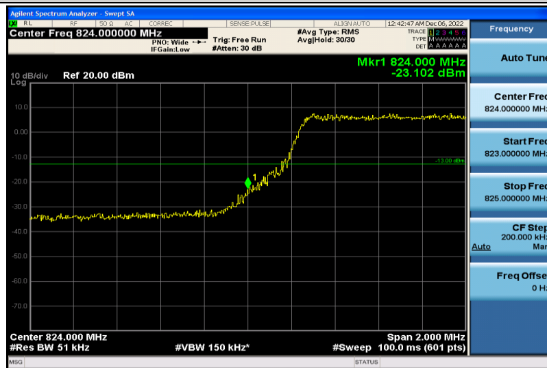
Band26-5MHz-QPSK-26815-25RB#0
