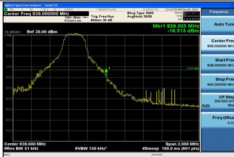
Band26-5MHz-QPSK-26915-1RB#24
