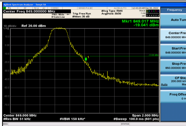
Band26-5MHz-QPSK-27015-1RB#24
