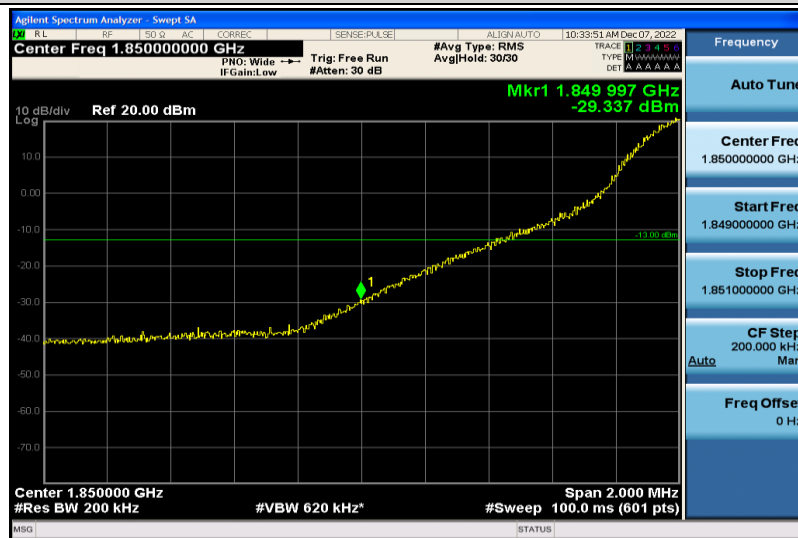
Band25-20MHz-16QAM-26140-1RB#0
