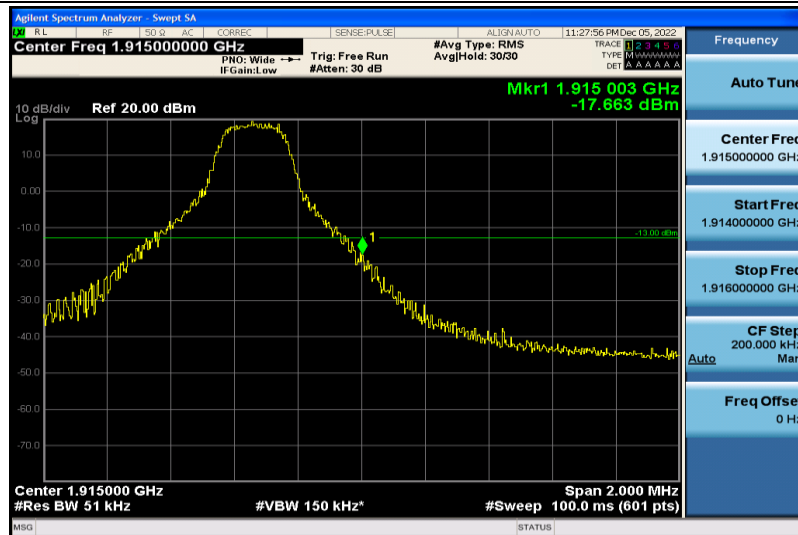
Band25-5MHz-QPSK-26665-1RB#24
