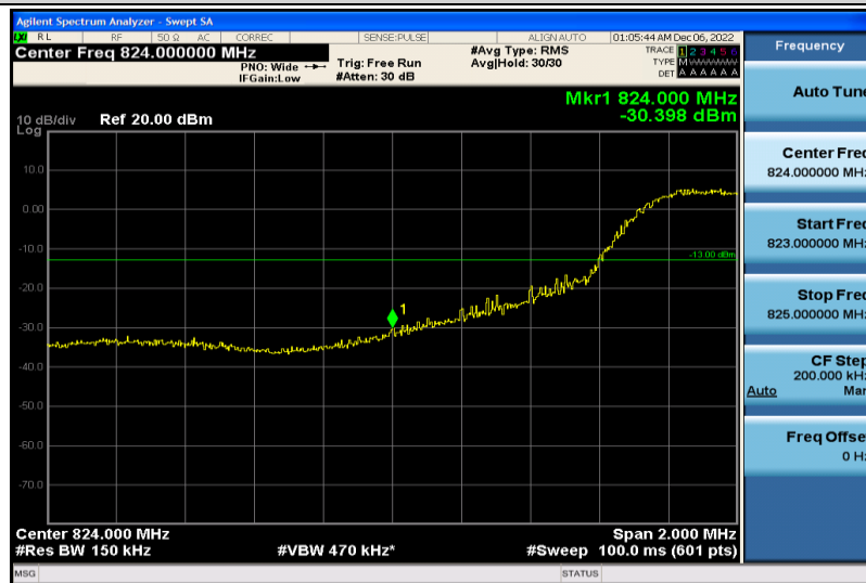
Band26-15MHz-QPSK-26865-75RB#0
