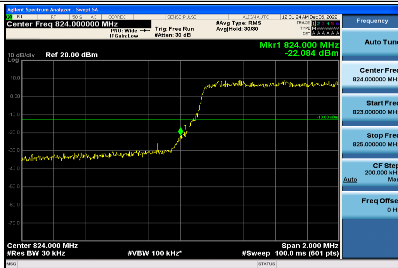
Band26-3MHz-QPSK-26805-15RB#0
