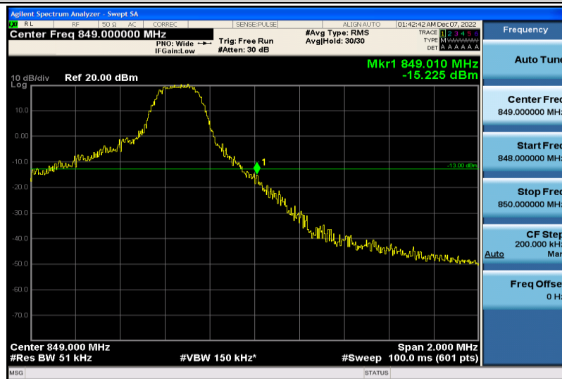
Band26-5MHz-16QAM-27015-1RB#24
