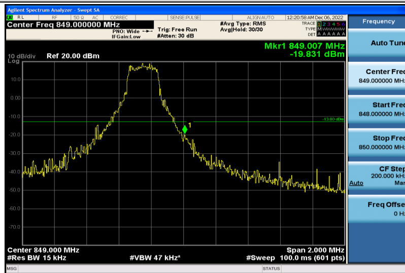
Band26-1.4MHz-QPSK-27033-1RB#5
