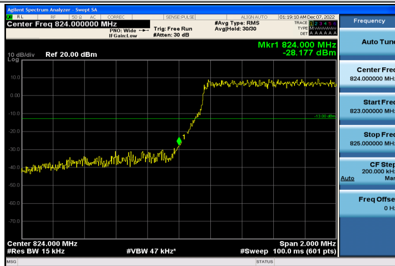
Band26-1.4MHz-16QAM-26797-6RB#0
