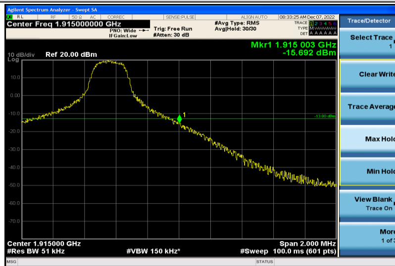
Band25-5MHz-16QAM-26665-1RB#24
