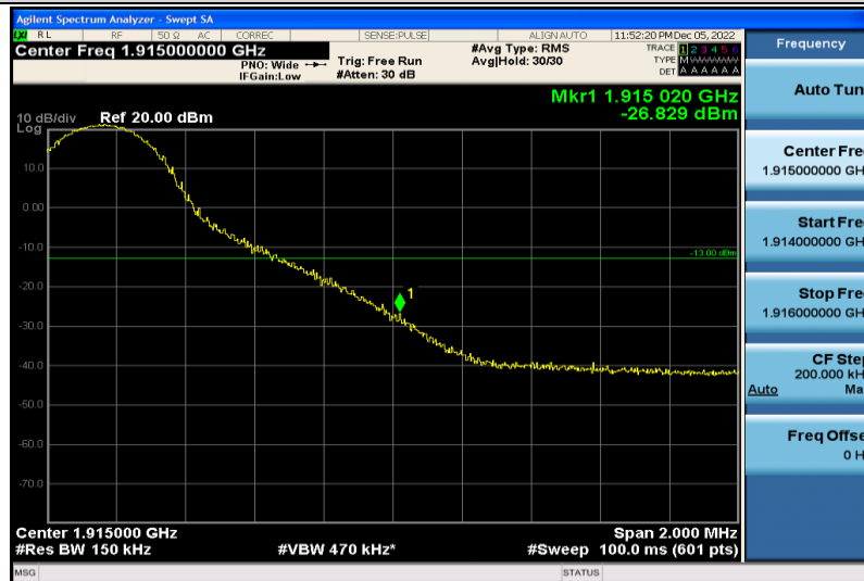
Band25-15MHz-QPSK-26615-1RB#74
