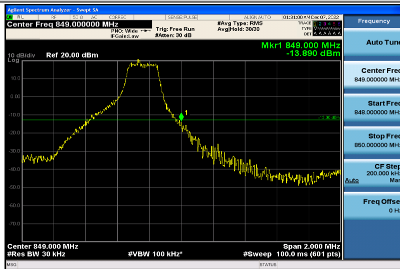
Band26-3MHz-16QAM-27025-1RB#14
