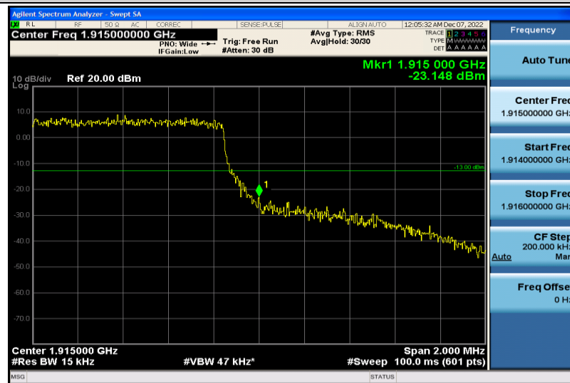
Band25-1.4MHz-16QAM-26683-6RB#0
