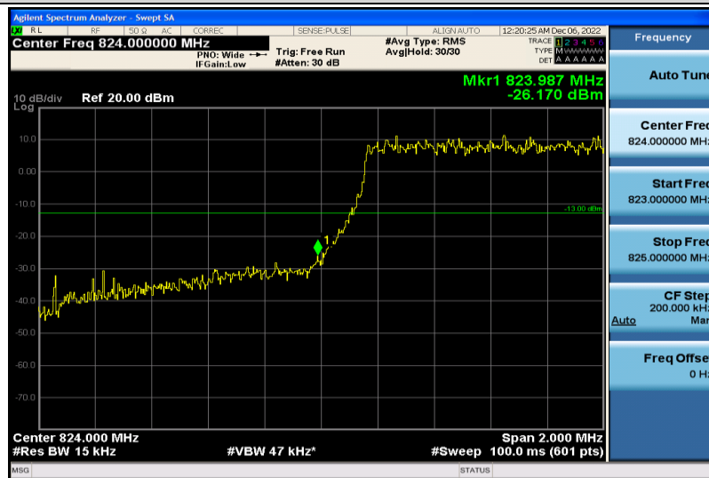
Band26-1.4MHz-QPSK-26797-6RB#0
