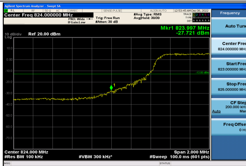
Band26-10MHz-QPSK-26840-50RB#0
