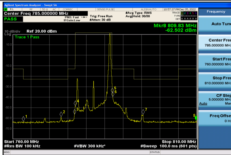
Band13-10MHz-QPSK-23230-1RB#49
