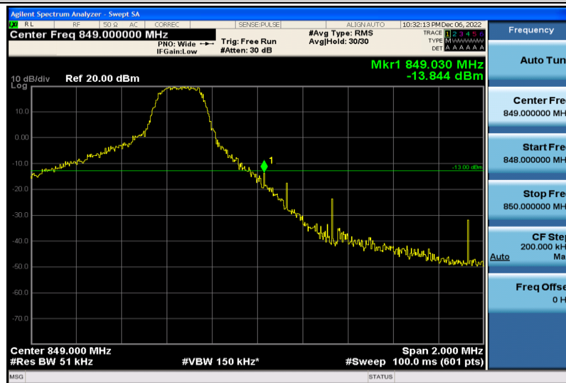
Band5-5MHz-16QAM-20625-1RB#24
