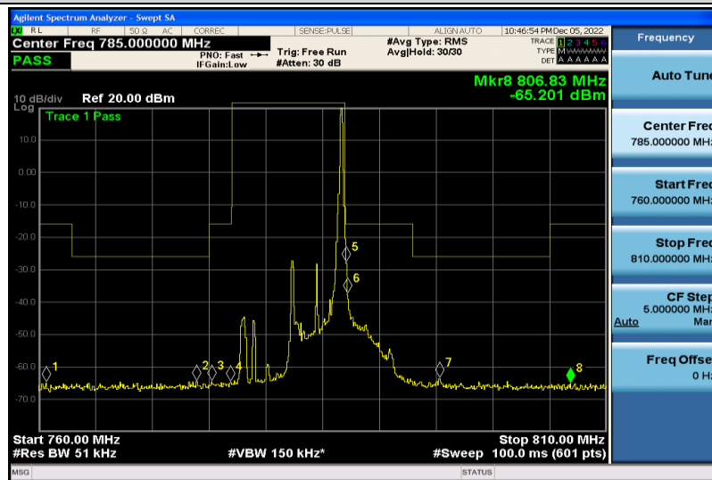
Band13-5MHz-QPSK-23255-1RB#24
