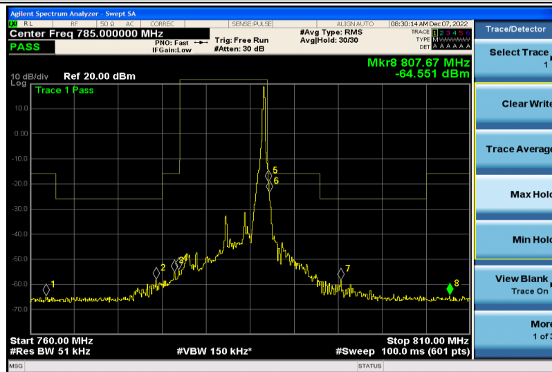
Band13-5MHz-16QAM-23255-1RB#24
