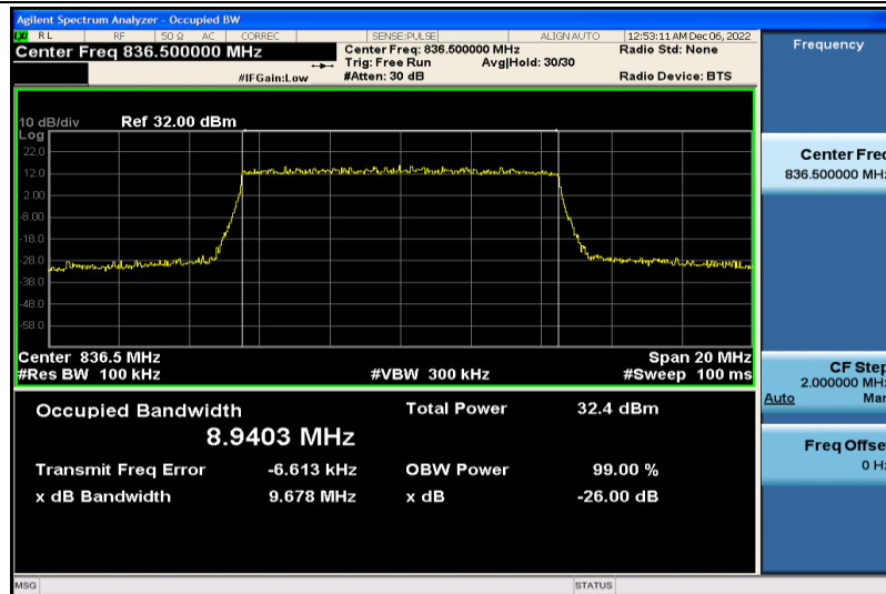
Band26-10MHz-QPSK-26915-50RB#0-8.9403
