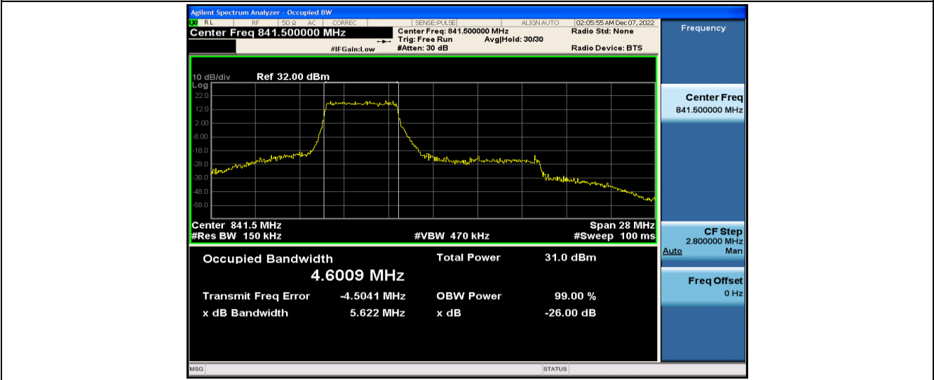
Band26-15MHz-16QAM-26965-25RB#0-4.6009
