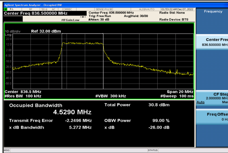
Band26-10MHz-16QAM-26915-25RB#0-4.5290
