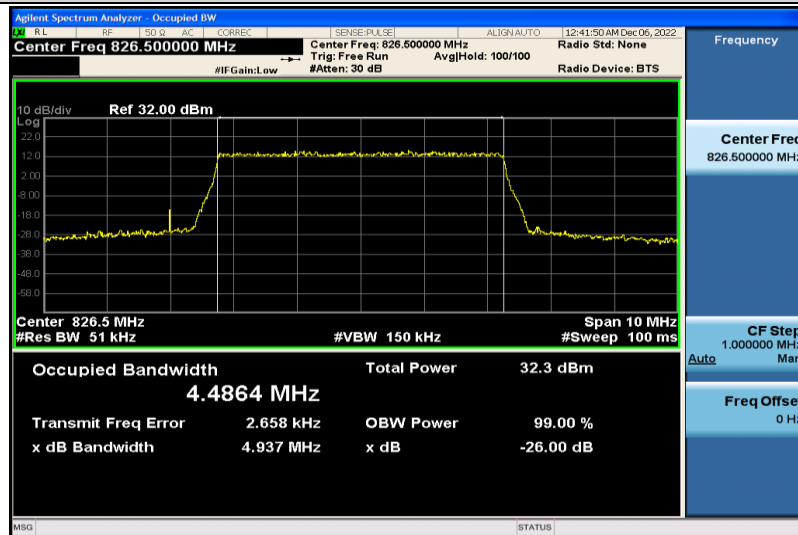
Band26-5MHz-QPSK-26815-25RB#0-4.4864
