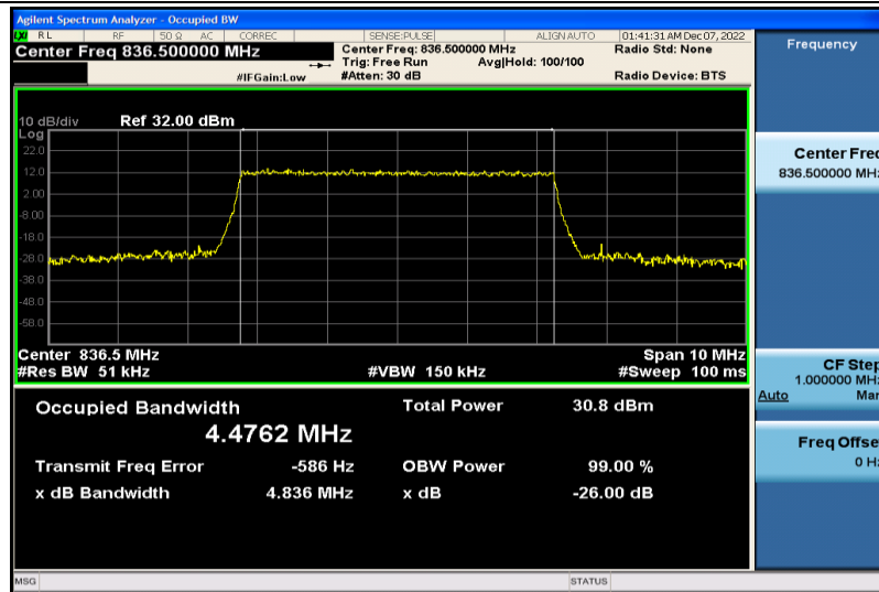
Band26-5MHz-16QAM-26915-25RB#0-4.4762
