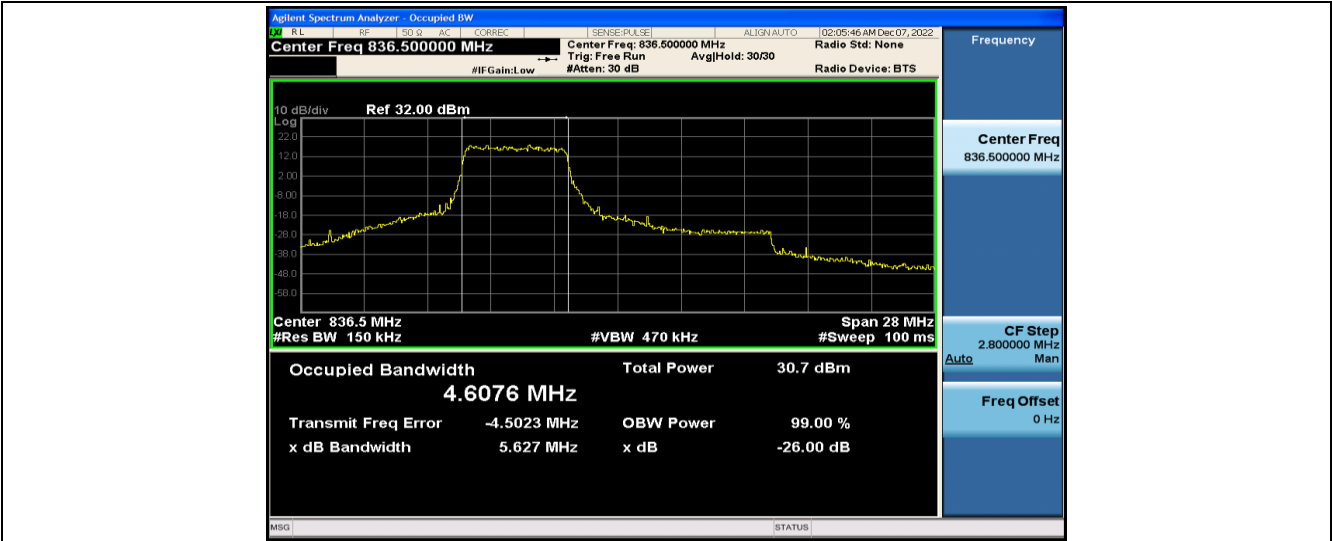
Band26-15MHz-16QAM-26915-25RB#0-4.6076
