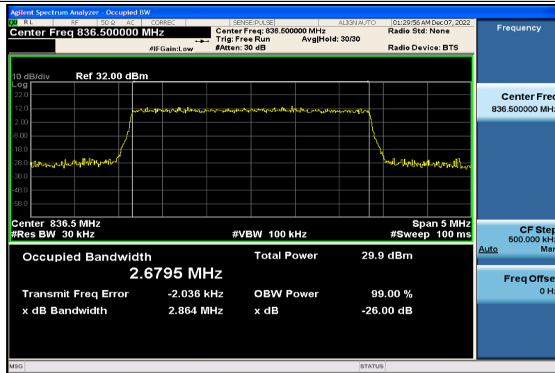
Band26-3MHz-16QAM-26915-15RB#0-2.6795
