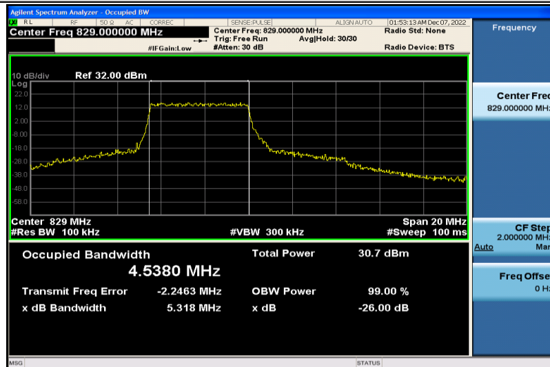
Band26-10MHz-16QAM-26840-25RB#0-4.5380
