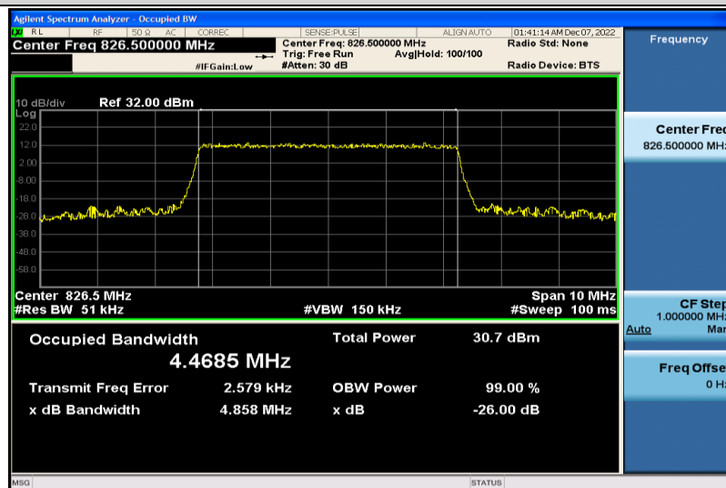
Band26-5MHz-16QAM-26815-25RB#0-4.4685
