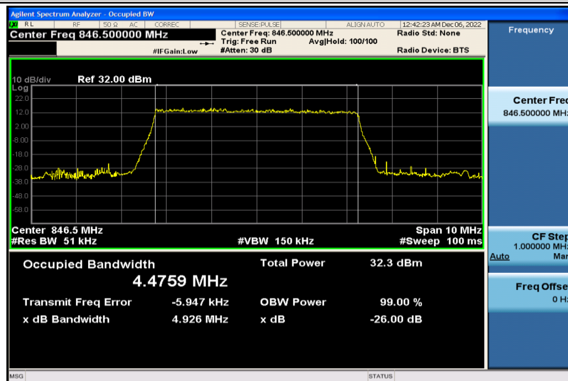
Band26-5MHz-QPSK-27015-25RB#0-4.4759
