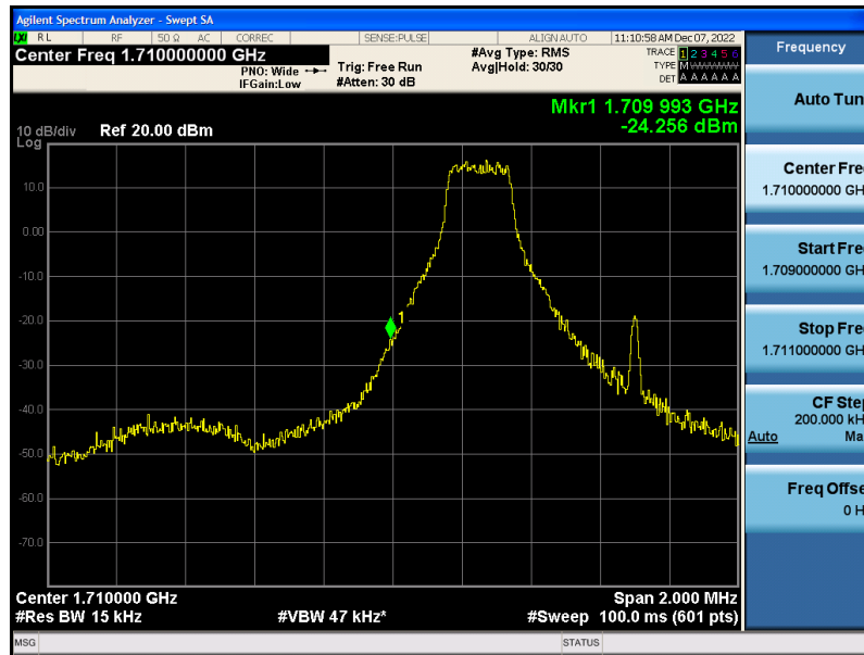
Band4-1.4MHz-QPSK-19957-1RB#0
