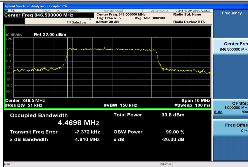
Band26-5MHz-16QAM-27015-25RB#0-4.4698
