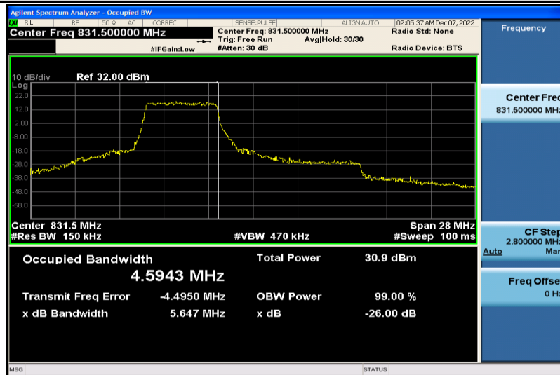
Band26-15MHz-16QAM-26865-25RB#0-4.5943
