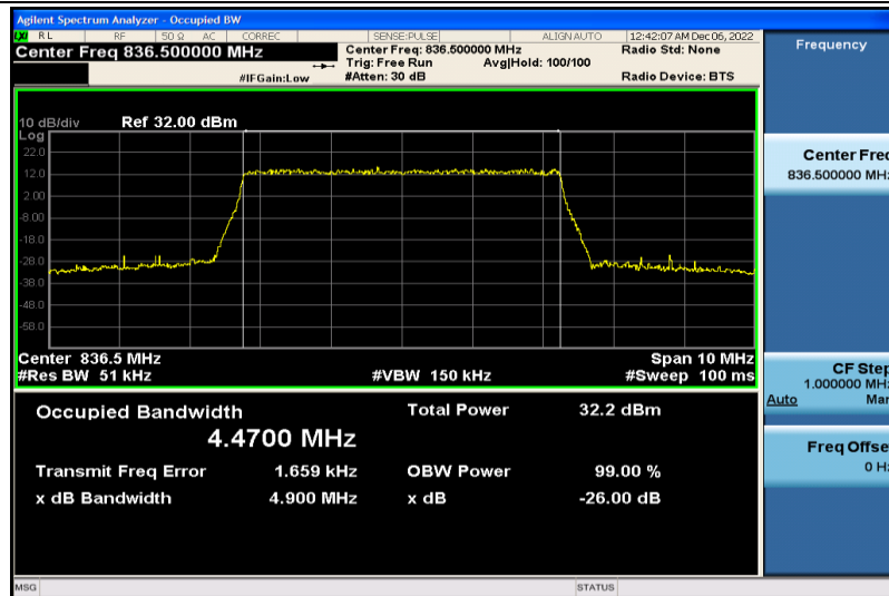
Band26-5MHz-QPSK-26915-25RB#0-4.4700
