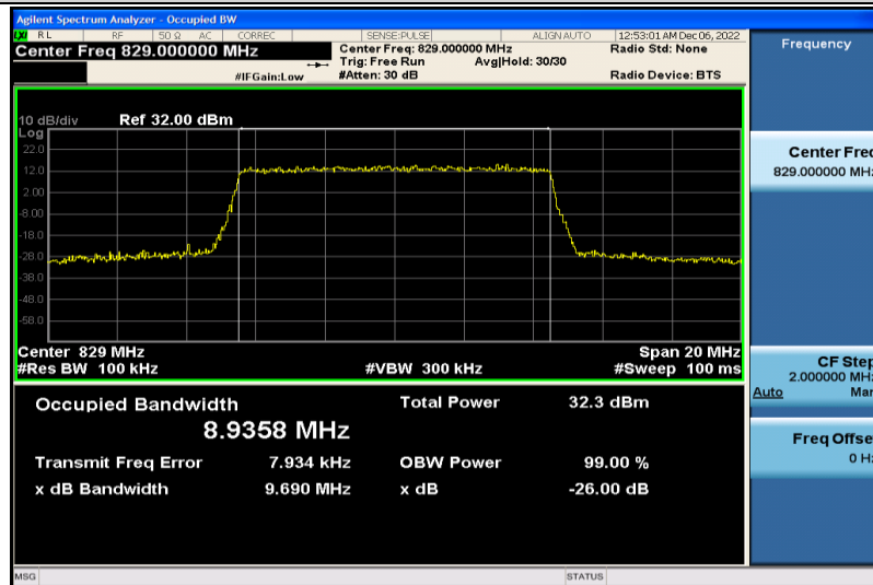
Band26-10MHz-QPSK-26840-50RB#0-8.9358
