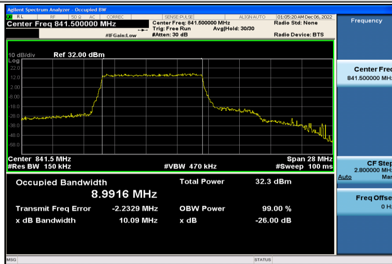
Band26-15MHz-QPSK-26965-75RB#0-8.9916
