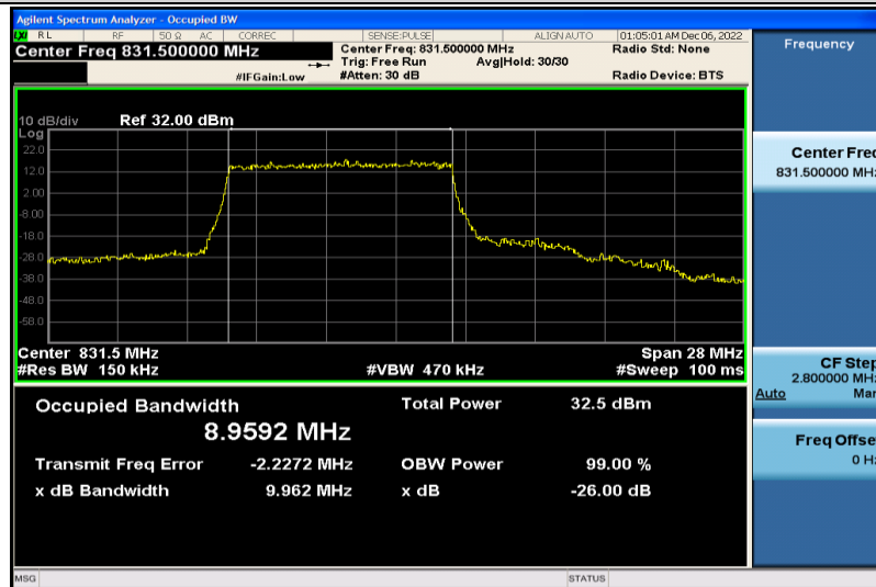
Band26-15MHz-QPSK-26865-75RB#0-8.9592
