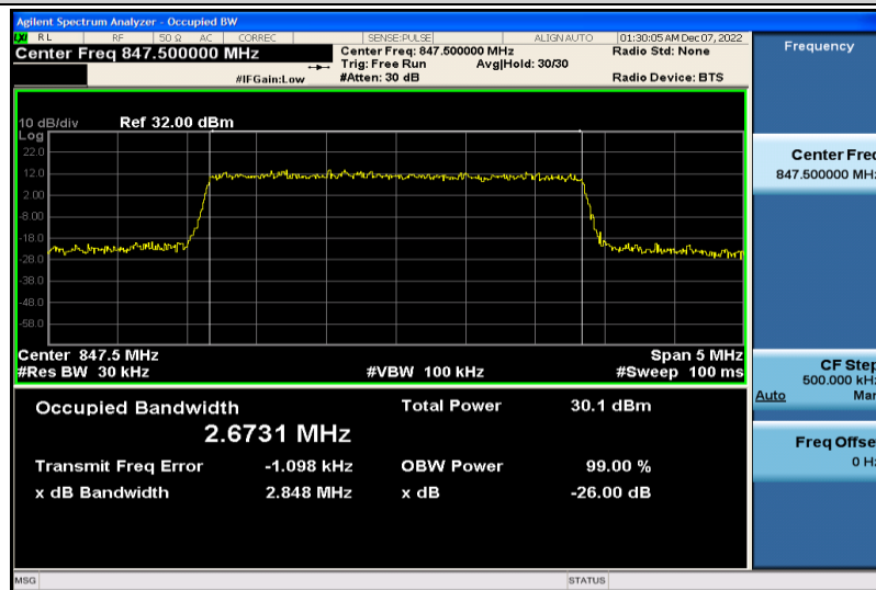
Band26-3MHz-16QAM-27025-15RB#0-2.6731
