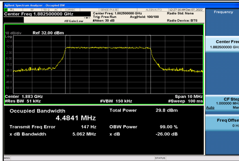
Band25-5MHz-16QAM-26365-25RB#0-4.4841
