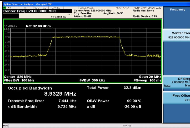
Band5-10MHz-QPSK-20450-50RB#0-8.9329
