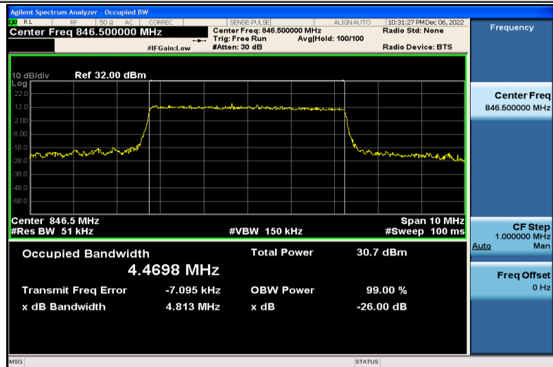
Band5-5MHz-16QAM-20625-25RB#0-4.4698
