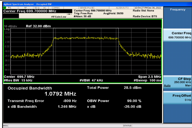
Band12-1.4MHz-16QAM-23017-6RB#0-1.0792
