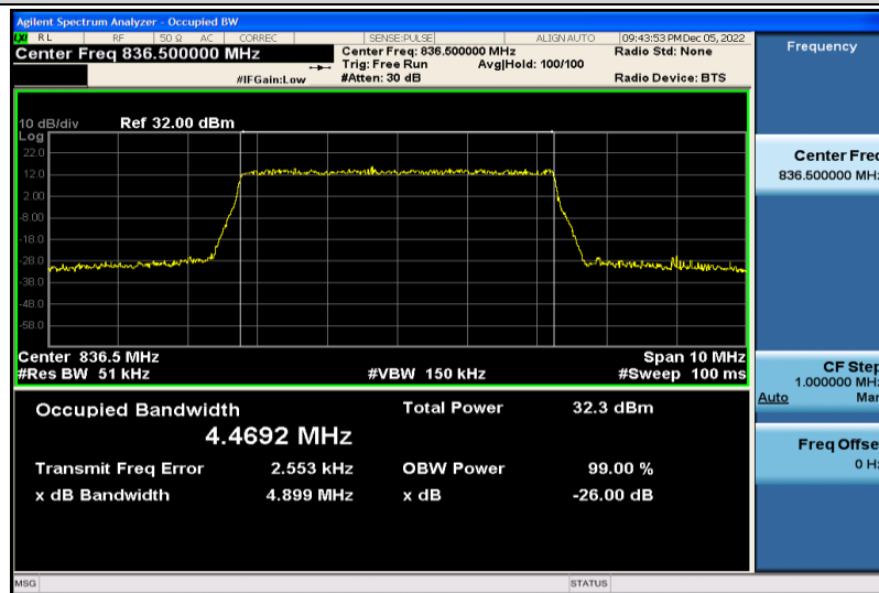
Band5-5MHz-QPSK-20525-25RB#0-4.4692
