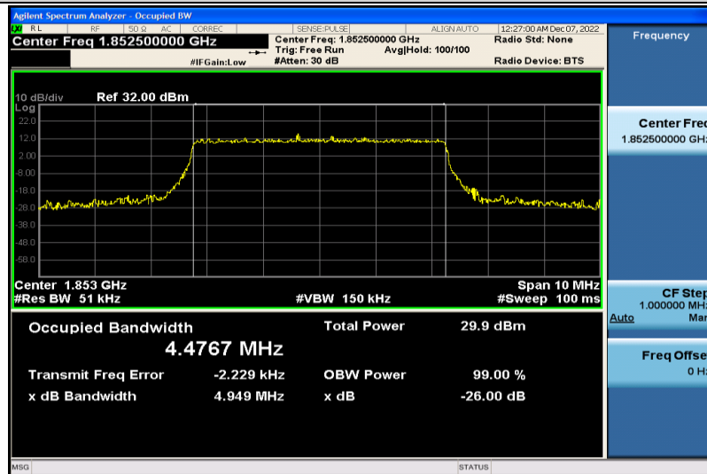
Band25-5MHz-16QAM-26065-25RB#0-4.4767
