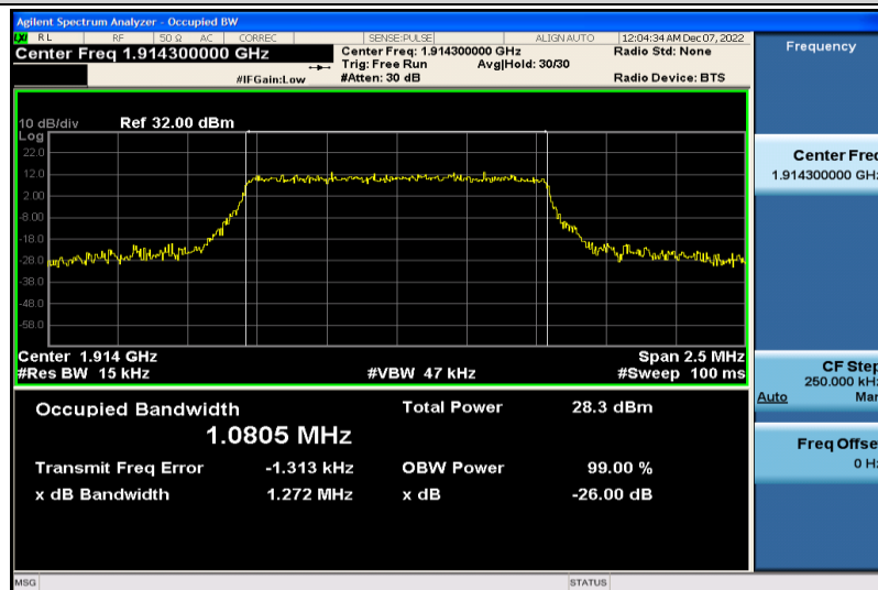
Band25-1.4MHz-16QAM-26683-6RB#0-1.0805
