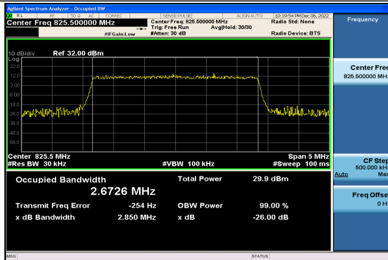
Band5-3MHz-16QAM-20415-15RB#0-2.6726
