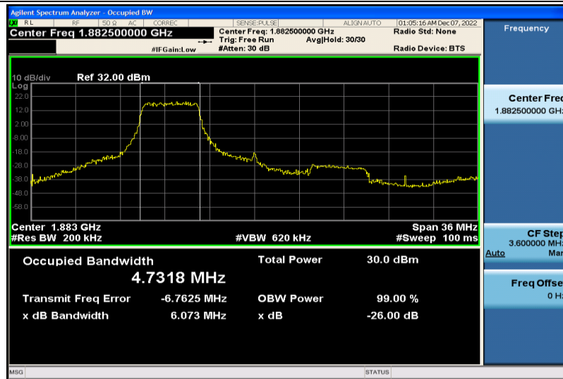
Band25-20MHz-16QAM-26365-25RB#0-4.7318
