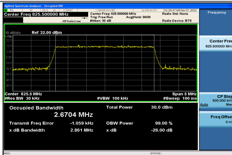
Band26-3MHz-16QAM-26805-15RB#0-2.6704
