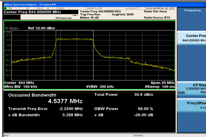
Band5-10MHz-16QAM-20600-25RB#0-4.5377
