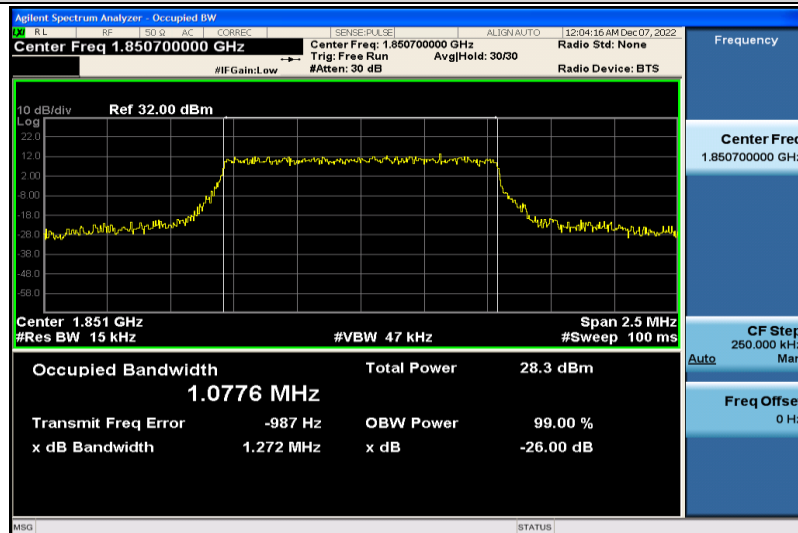
Band25-1.4MHz-16QAM-26047-6RB#0-1.0776
