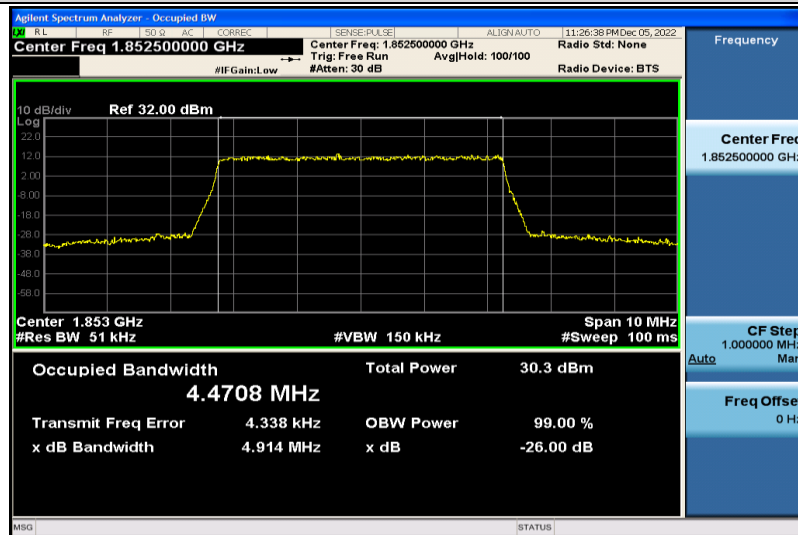
Band25-5MHz-QPSK-26065-25RB#0-4.4708
