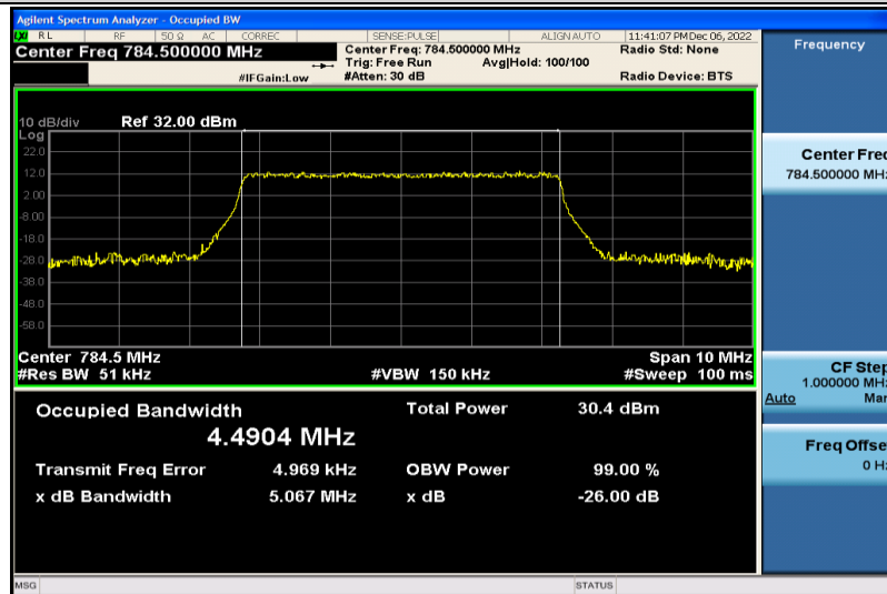
Band13-5MHz-16QAM-23255-25RB#0-4.4904
