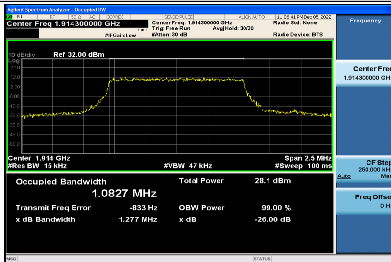
Band25-1.4MHz-QPSK-26683-6RB#0-1.0827
