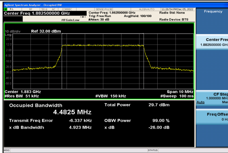
Band25-5MHz-QPSK-26365-25RB#0-4.4825
