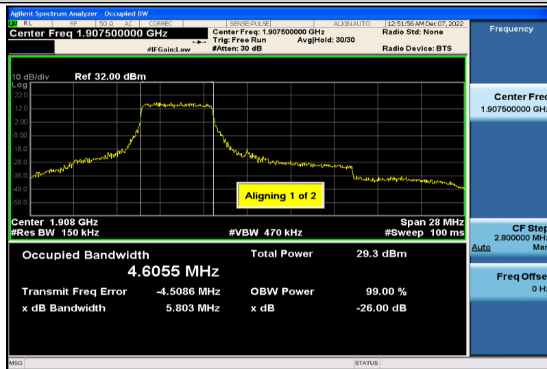
Band25-15MHz-16QAM-26615-25RB#0-4.6055
