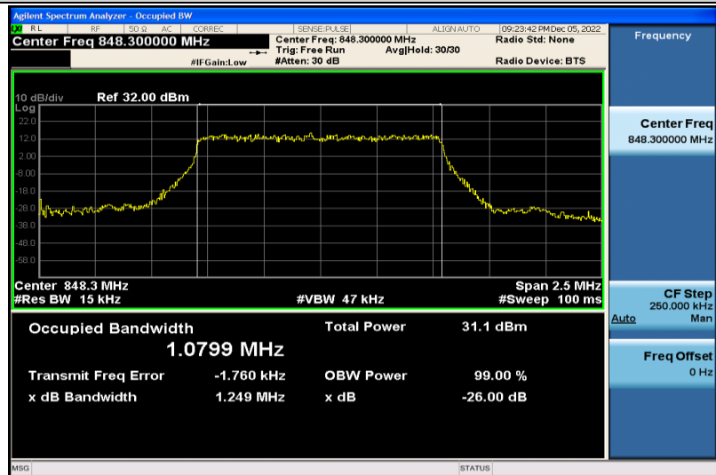
Band5-1.4MHz-QPSK-20643-6RB#0-1.0799
