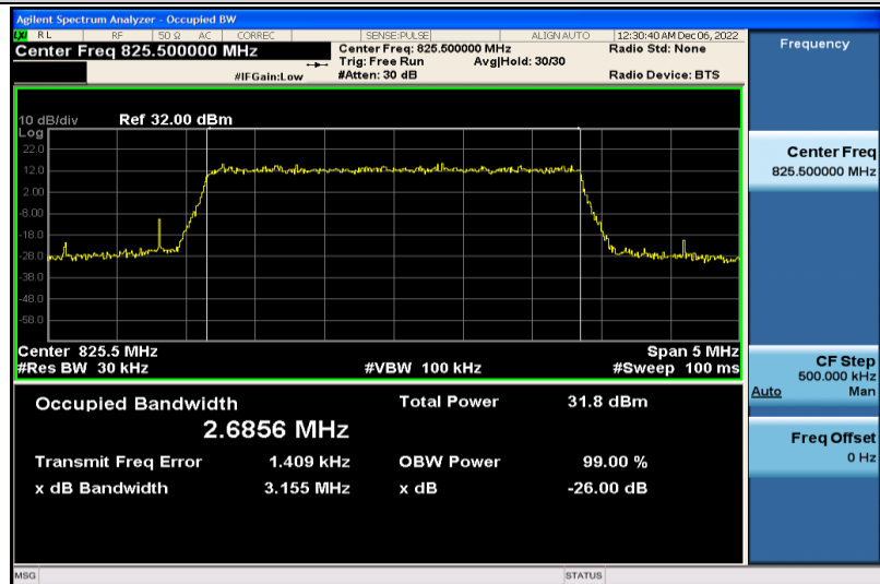
Band26-3MHz-QPSK-26805-15RB#0-2.6856
