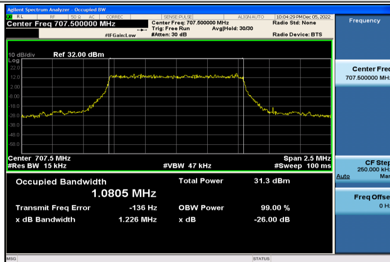
Band12-1.4MHz-QPSK-23095-6RB#0-1.0805
