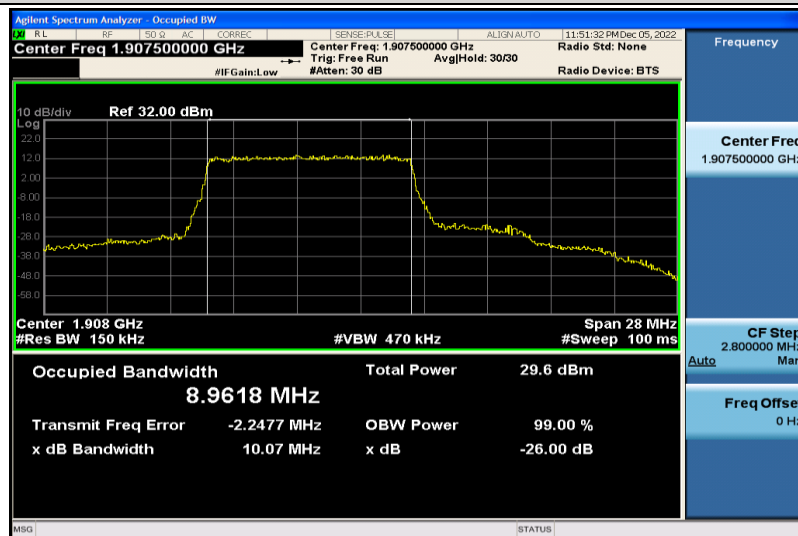
Band25-15MHz-QPSK-26615-75RB#0-8.9618
