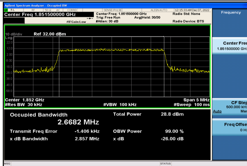
Band25-3MHz-16QAM-26055-15RB#0-2.6682
