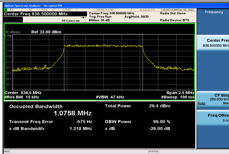
Band5-1.4MHz-16QAM-20525-6RB#0-1.0758
