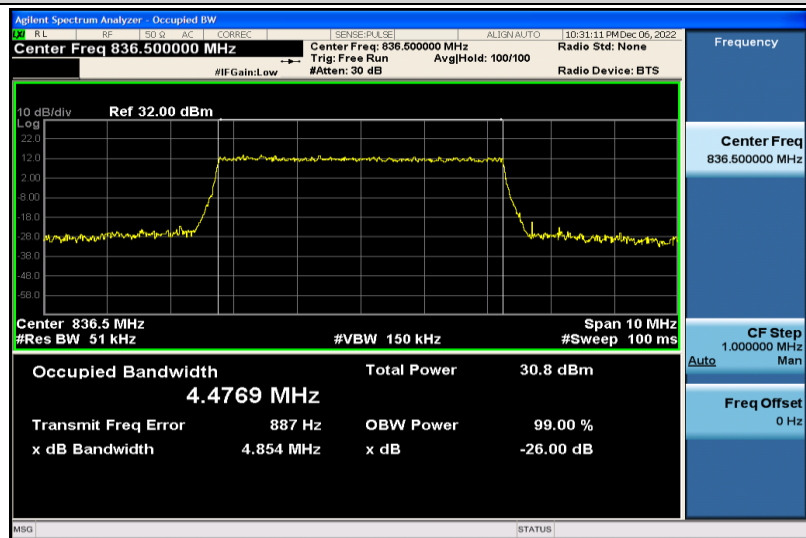
Band5-5MHz-16QAM-20525-25RB#0-4.4769
