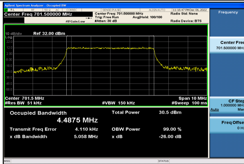
Band12-5MHz-16QAM-23035-25RB#0-4.4875
