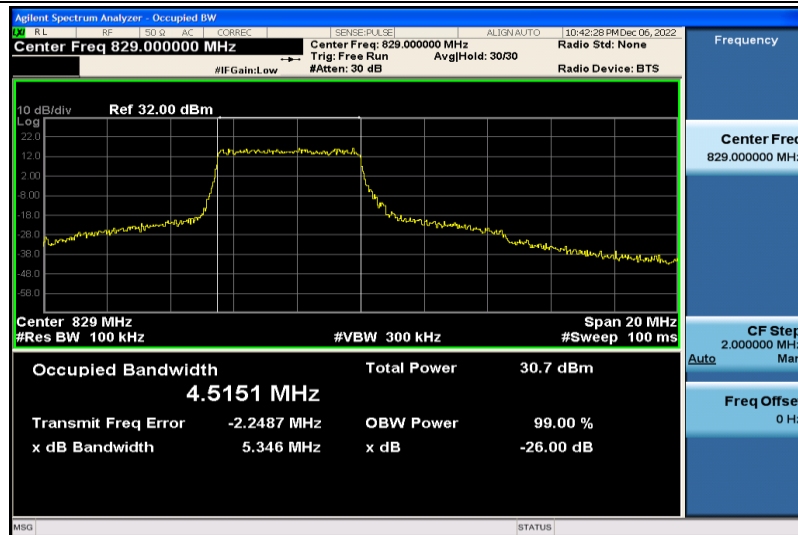
Band5-10MHz-16QAM-20450-25RB#0-4.5151
