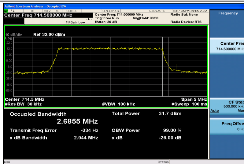
Band12-3MHz-QPSK-23165-15RB#0-2.6855
