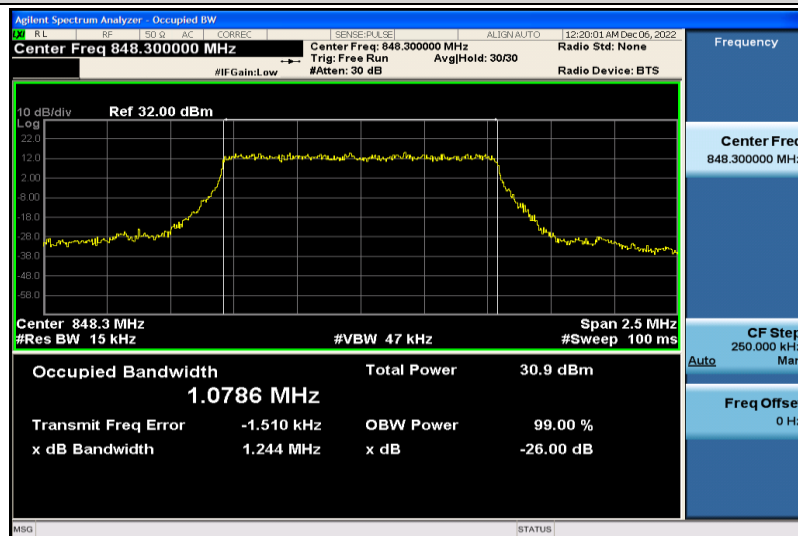
Band26-1.4MHz-QPSK-27033-6RB#0-1.0786
