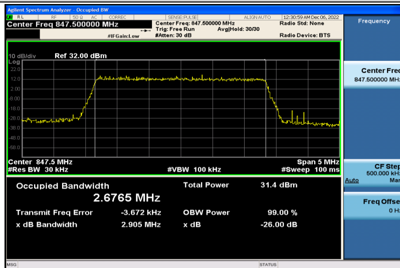
Band26-3MHz-QPSK-27025-15RB#0-2.6765
