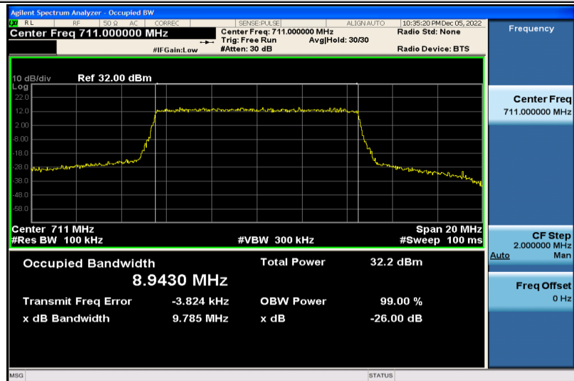
Band12-10MHz-QPSK-23130-50RB#0-8.9430
