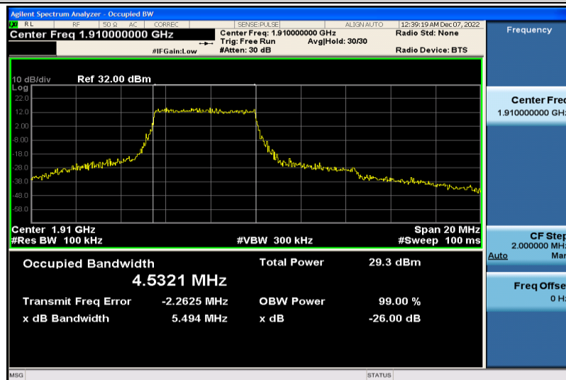
Band25-10MHz-16QAM-26640-25RB#0-4.5321
