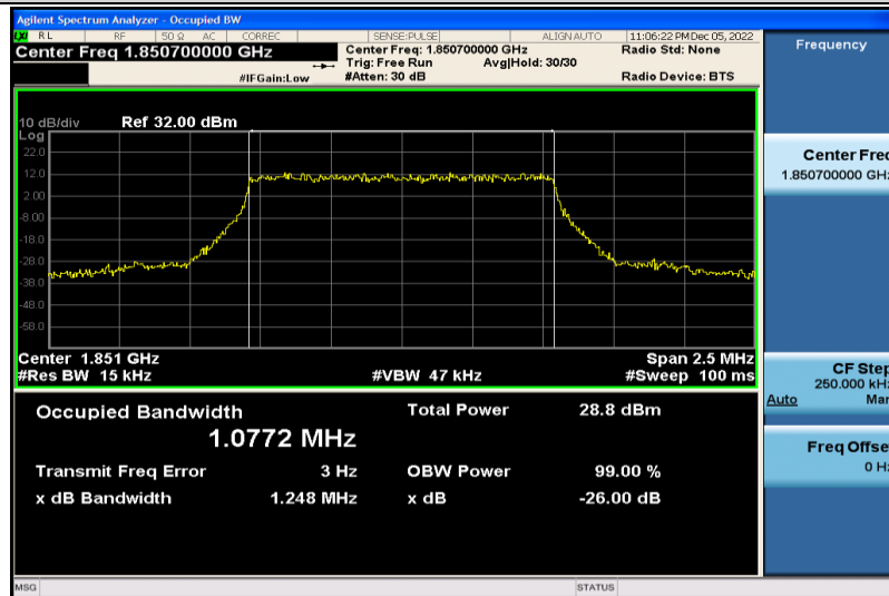
Band25-1.4MHz-QPSK-26047-6RB#0-1.0772
