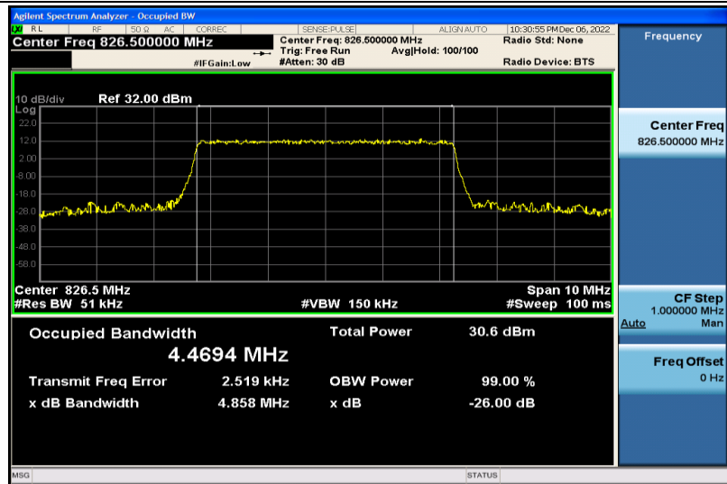
Band5-5MHz-16QAM-20425-25RB#0-4.4694
