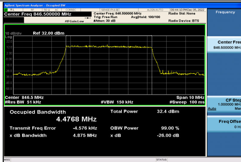
Band5-5MHz-QPSK-20625-25RB#0-4.4768
