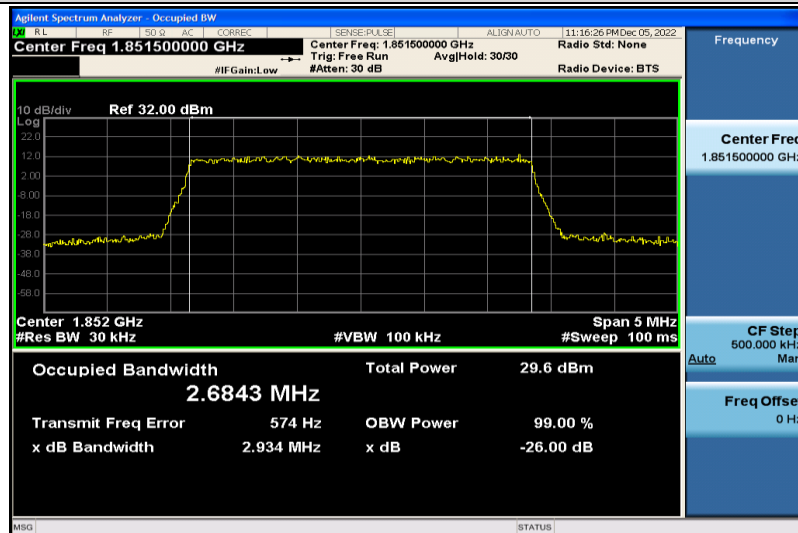
Band25-3MHz-QPSK-26055-15RB#0-2.6843
