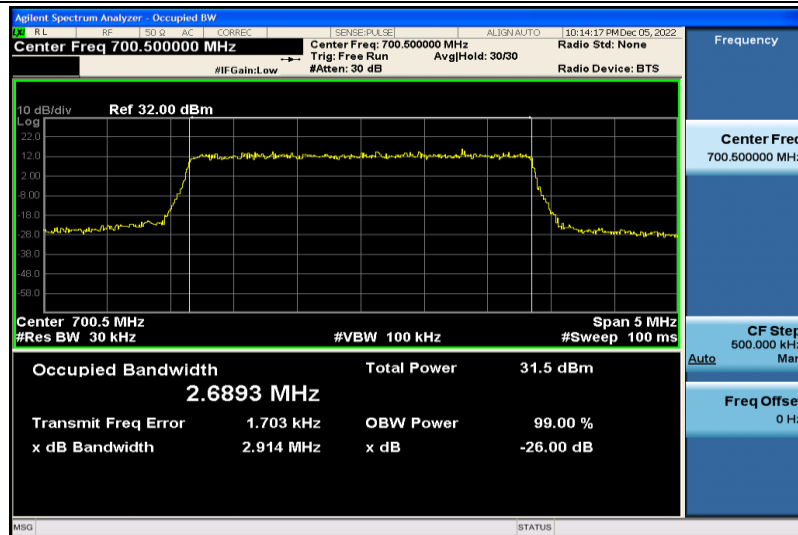
Band12-3MHz-QPSK-23025-15RB#0-2.6893
