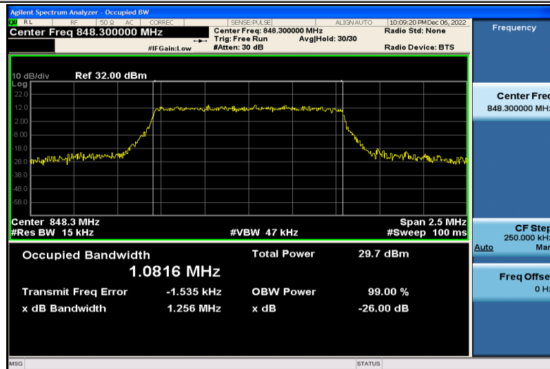
Band5-1.4MHz-16QAM-20643-6RB#0-1.0816
