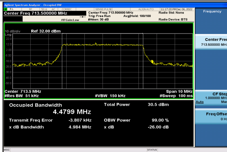
Band12-5MHz-16QAM-23155-25RB#0-4.4799
