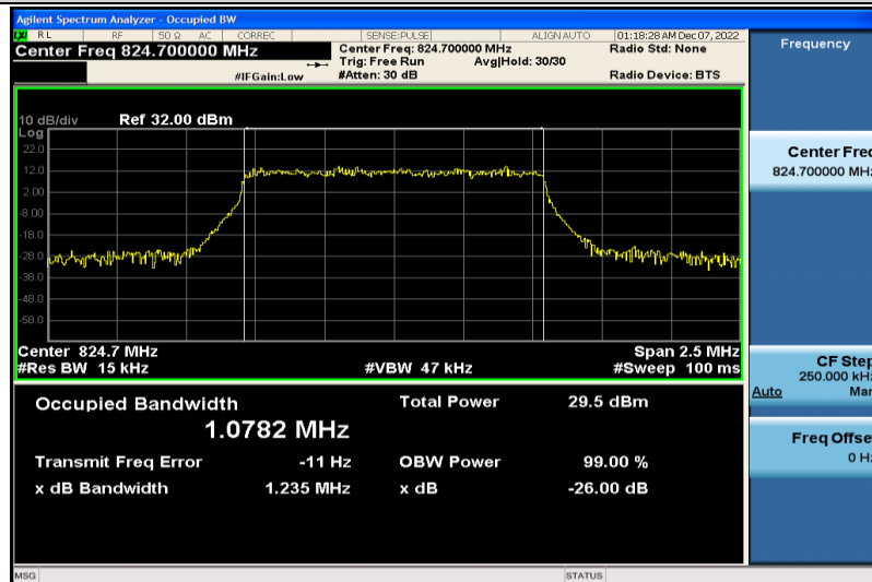
Band26-1.4MHz-16QAM-26797-6RB#0-1.0782
