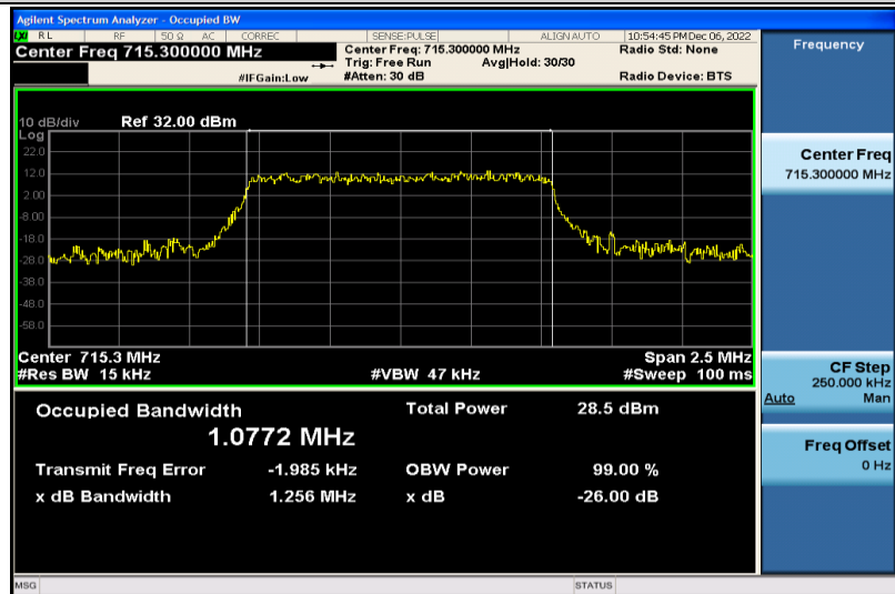
Band12-1.4MHz-16QAM-23173-6RB#0-1.0772
