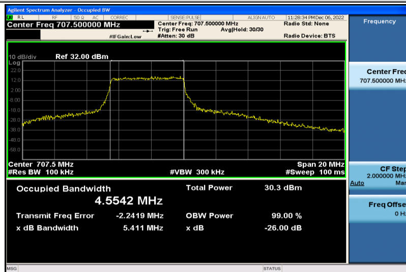
Band12-10MHz-16QAM-23095-25RB#0-4.5542
