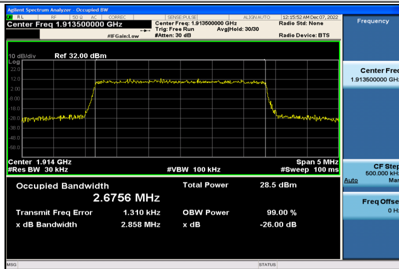
Band25-3MHz-16QAM-26675-15RB#0-2.6756
