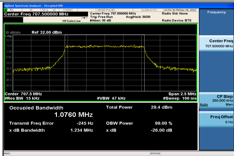
Band12-1.4MHz-16QAM-23095-6RB#0-1.0760
