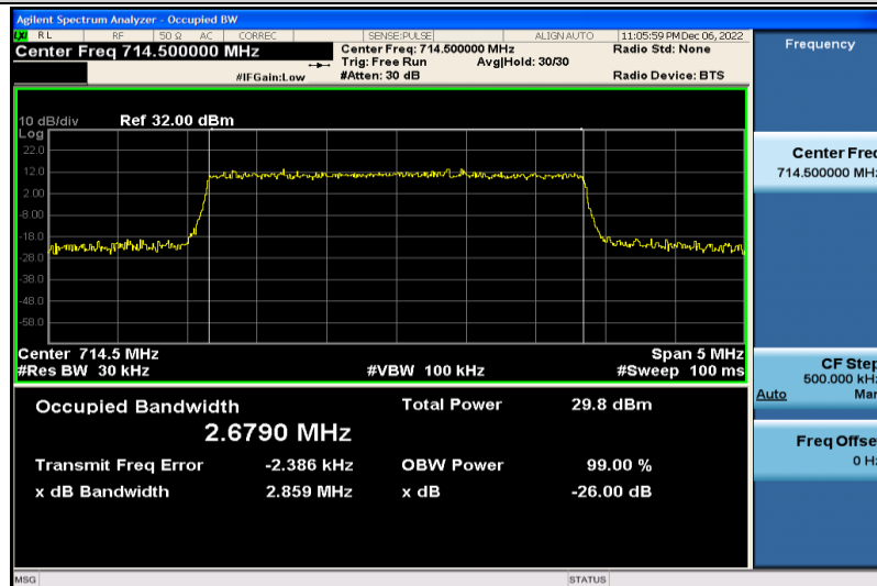
Band12-3MHz-16QAM-23165-15RB#0-2.6790
