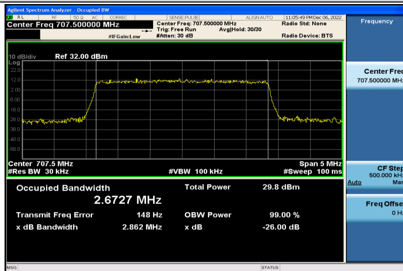
Band12-3MHz-16QAM-23095-15RB#0-2.6727
