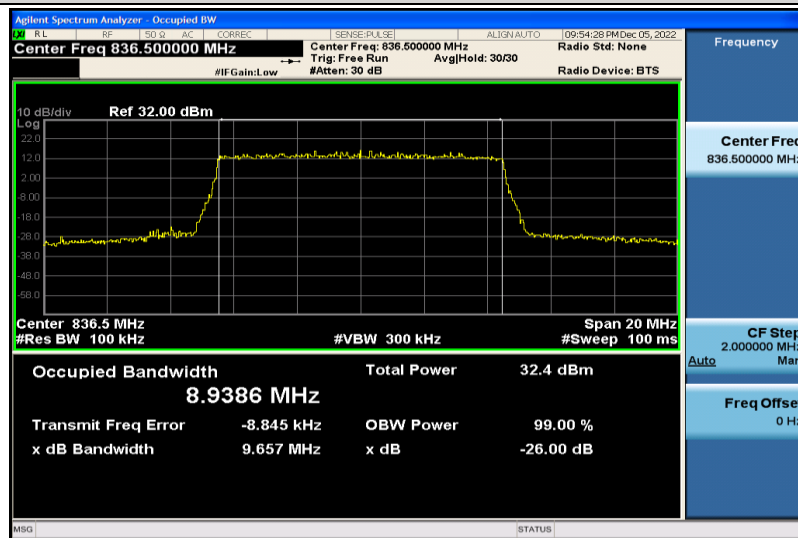
Band5-10MHz-QPSK-20525-50RB#0-8.9386
