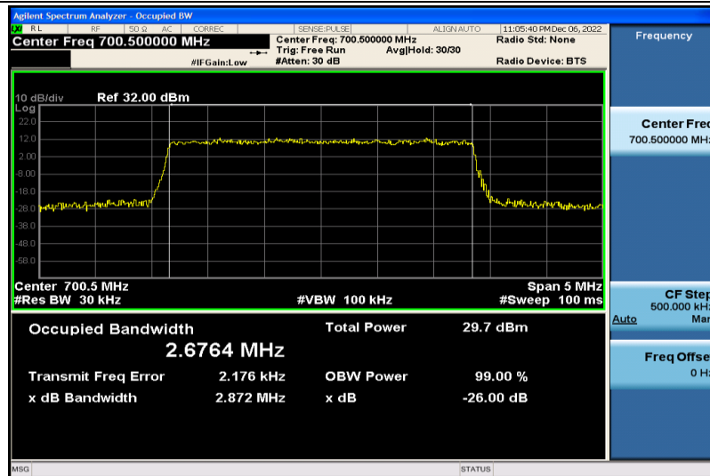
Band12-3MHz-16QAM-23025-15RB#0-2.6764
