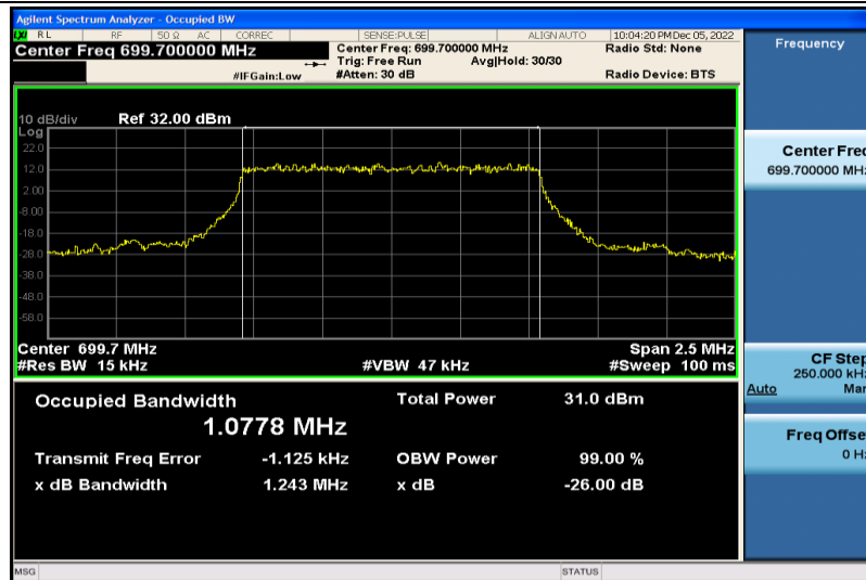
Band12-1.4MHz-QPSK-23017-6RB#0-1.0778
