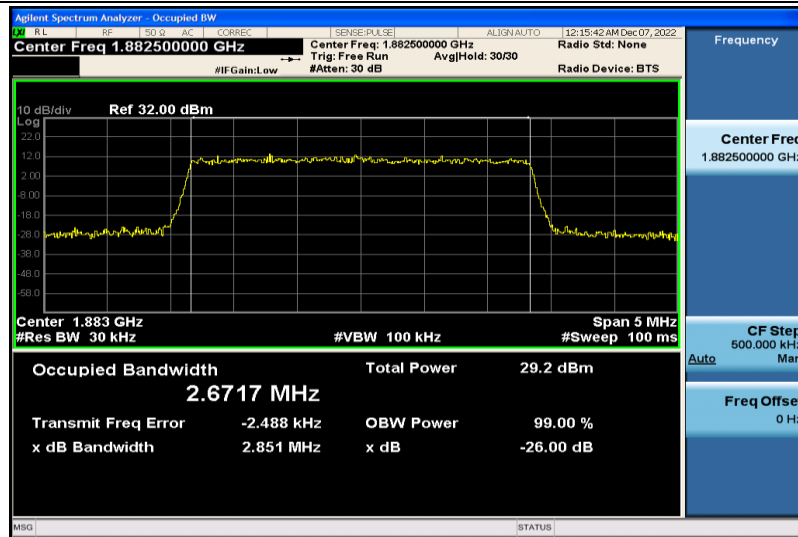
Band25-3MHz-16QAM-26365-15RB#0-2.6717
