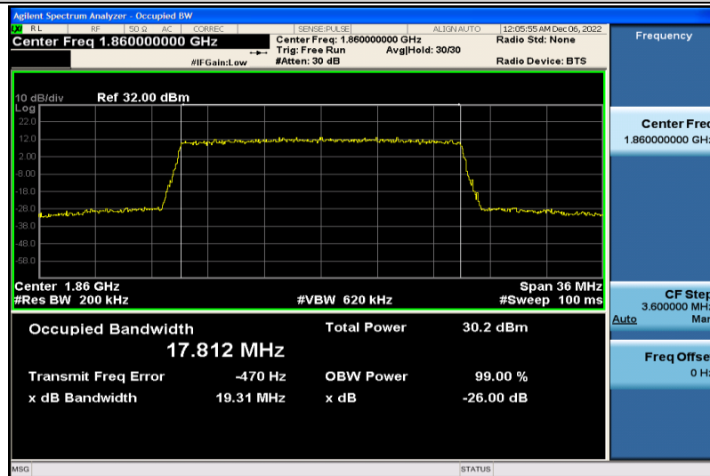
Band25-20MHz-QPSK-26140-100RB#0-17.812
