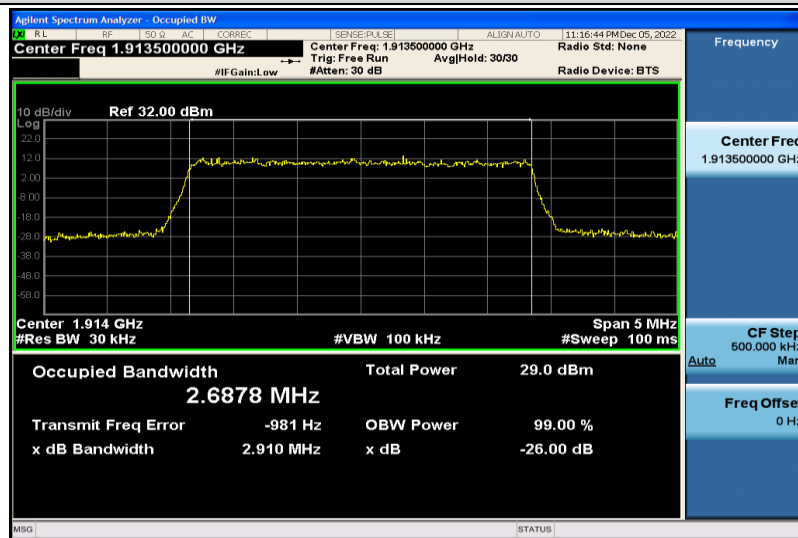
Band25-3MHz-QPSK-26675-15RB#0-2.6878
