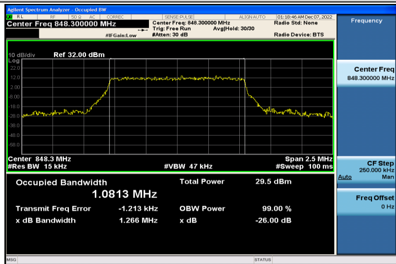
Band26-1.4MHz-16QAM-27033-6RB#0-1.0813
