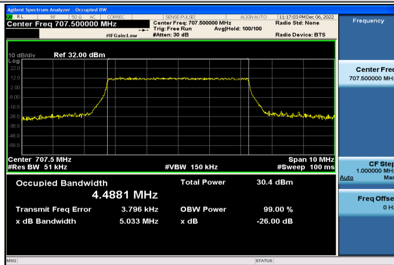
Band12-5MHz-16QAM-23095-25RB#0-4.4881
