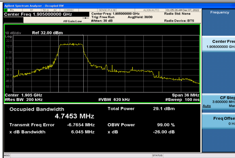
Band25-20MHz-16QAM-26590-25RB#0-4.7453
