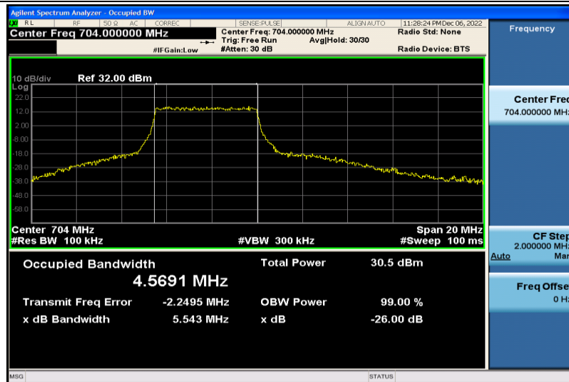
Band12-10MHz-16QAM-23060-25RB#0-4.5691
