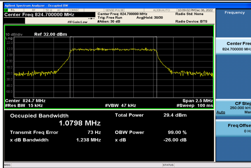
Band5-1.4MHz-16QAM-20407-6RB#0-1.0798
