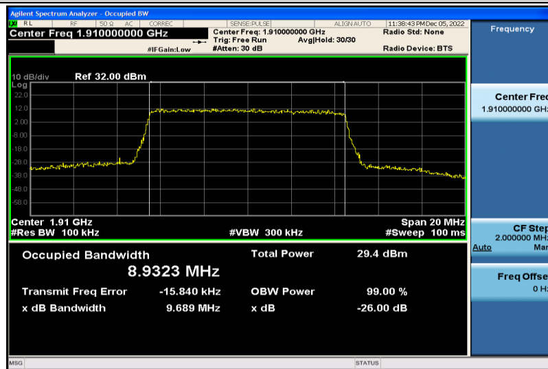
Band25-10MHz-QPSK-26640-50RB#0-8.9323
