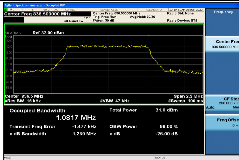
Band26-1.4MHz-QPSK-26915-6RB#0-1.0817
