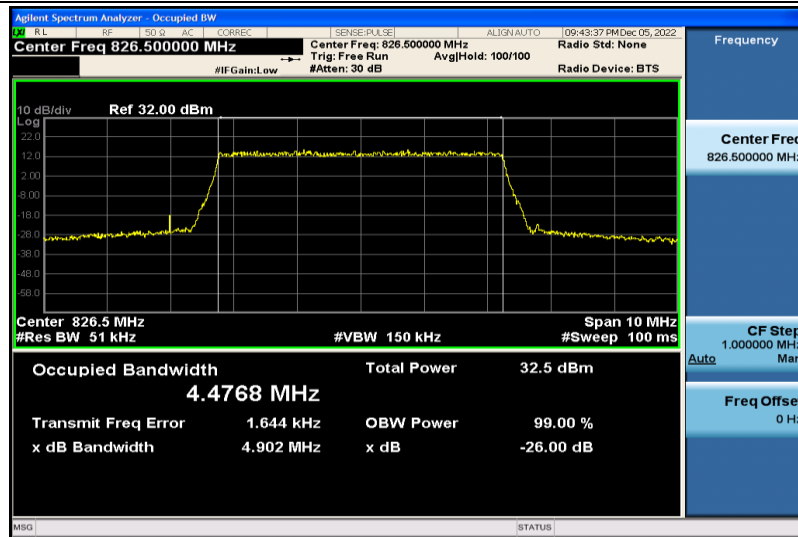
Band5-5MHz-QPSK-20425-25RB#0-4.4768
