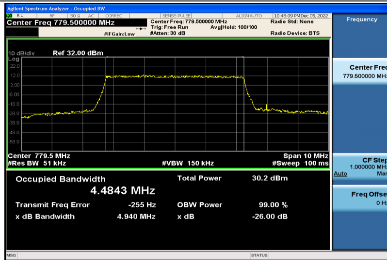
Band13-5MHz-QPSK-23205-25RB#0-4.4843
