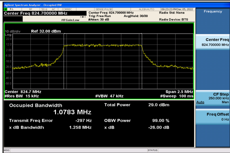
Band5-1.4MHz-QPSK-20407-6RB#0-1.0783
