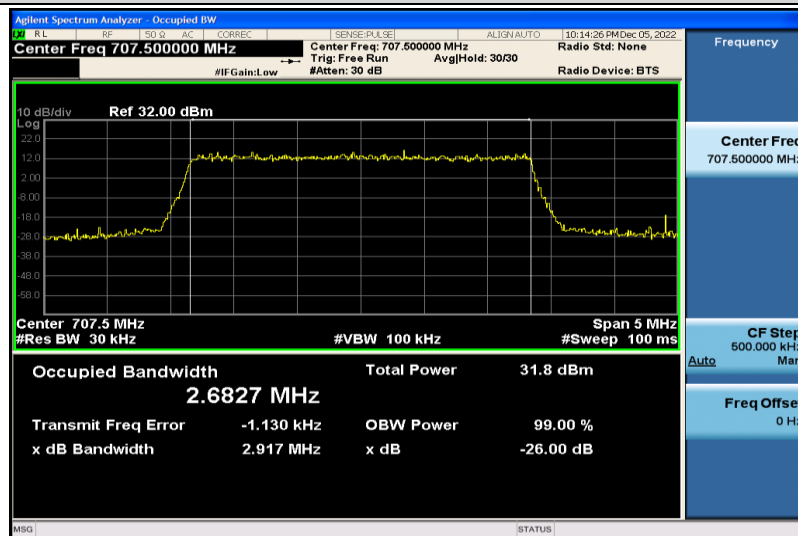
Band12-3MHz-QPSK-23095-15RB#0-2.6827
