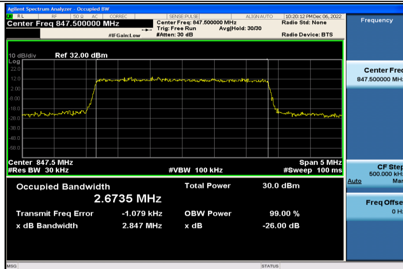
Band5-3MHz-16QAM-20635-15RB#0-2.6735
