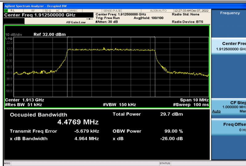
Band25-5MHz-16QAM-26665-25RB#0-4.4769
