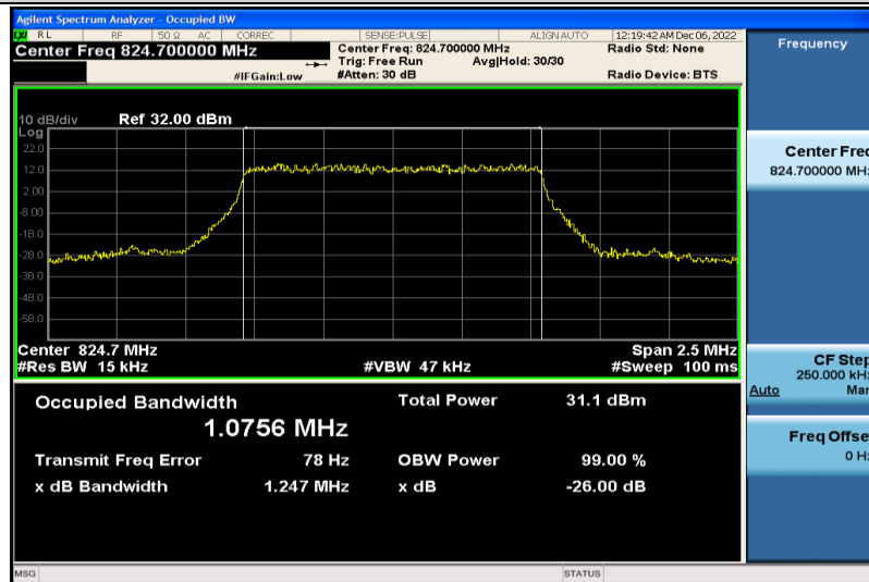
Band26-1.4MHz-QPSK-26797-6RB#0-1.0756
