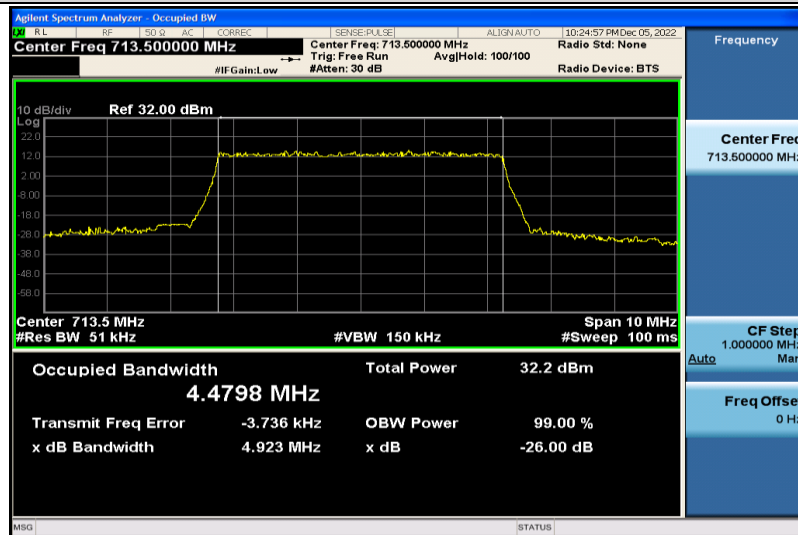
Band12-5MHz-QPSK-23155-25RB#0-4.4798
