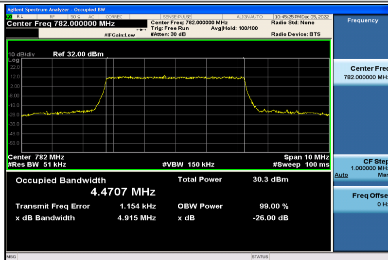
Band13-5MHz-QPSK-23230-25RB#0-4.4707
