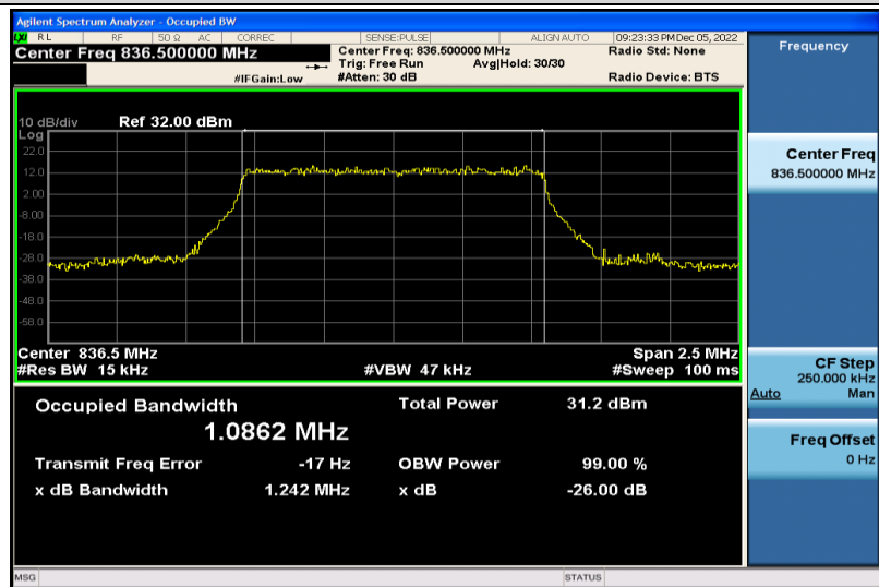
Band5-1.4MHz-QPSK-20525-6RB#0-1.0862
