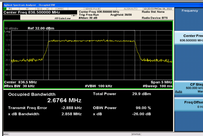
Band5-3MHz-16QAM-20525-15RB#0-2.6764
