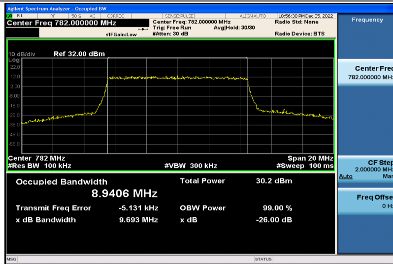
Band13-10MHz-QPSK-23230-50RB#0-8.9406
