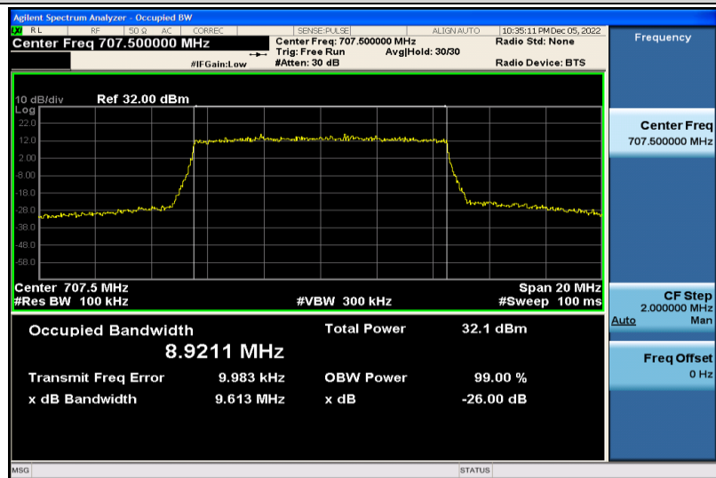
Band12-10MHz-QPSK-23095-50RB#0-8.9211
