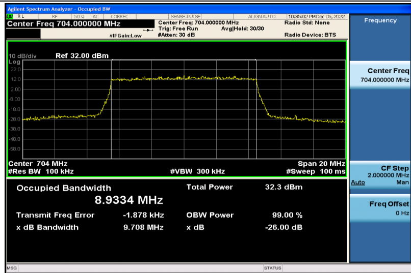
Band12-10MHz-QPSK-23060-50RB#0-8.9334
