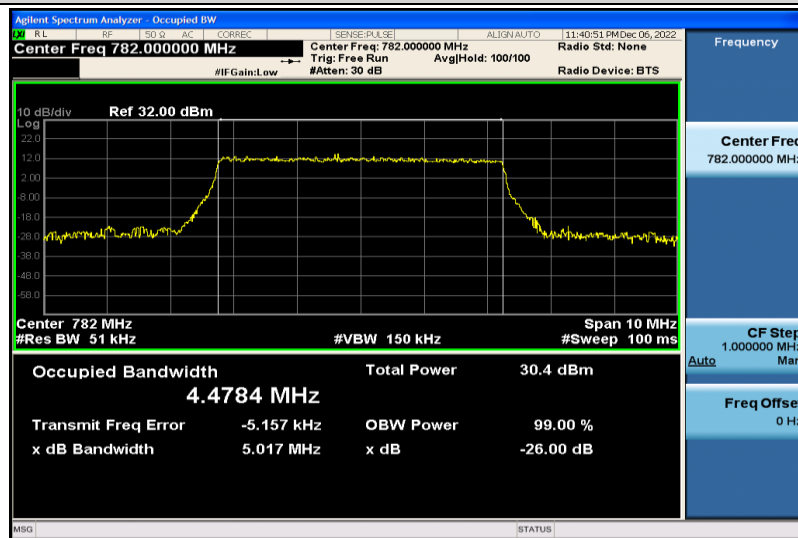
Band13-5MHz-16QAM-23230-25RB#0-4.4784
