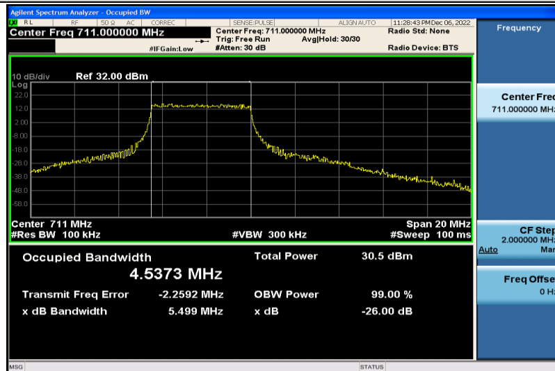
Band12-10MHz-16QAM-23130-25RB#0-4.5373
