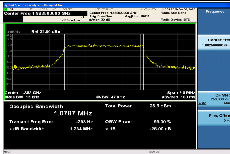
Band25-1.4MHz-16QAM-26365-6RB#0-1.0787
