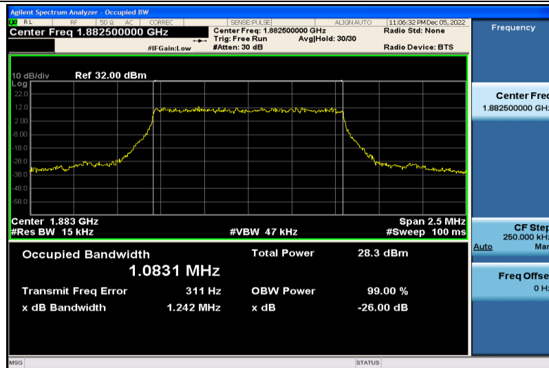
Band25-1.4MHz-QPSK-26365-6RB#0-1.0831
