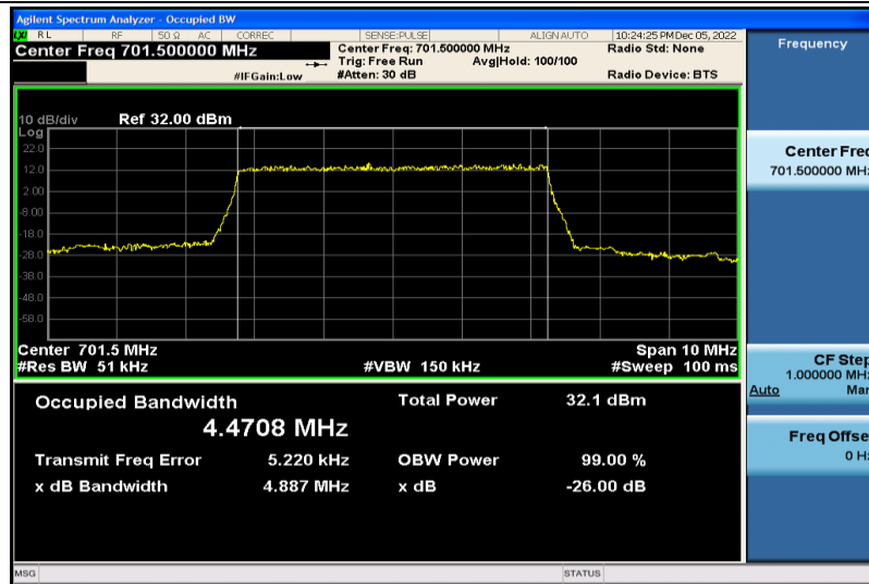
Band12-5MHz-QPSK-23035-25RB#0-4.4708
