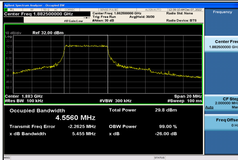
Band25-10MHz-16QAM-26365-25RB#0-4.5560
