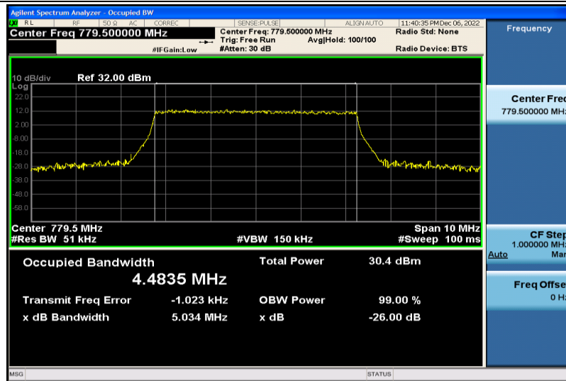
Band13-5MHz-16QAM-23205-25RB#0-4.4835
