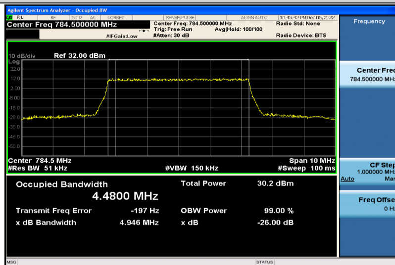
Band13-5MHz-QPSK-23255-25RB#0-4.4800
