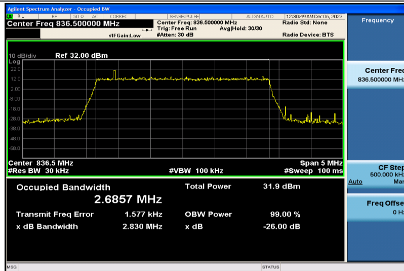
Band26-3MHz-QPSK-26915-15RB#0-2.6857
