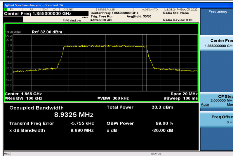
Band25-10MHz-QPSK-26090-50RB#0-8.9325
