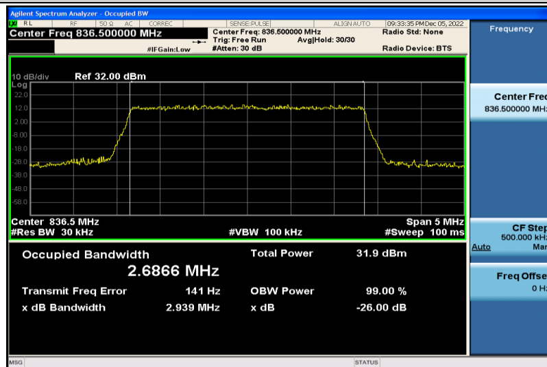
Band5-3MHz-QPSK-20525-15RB#0-2.6866
