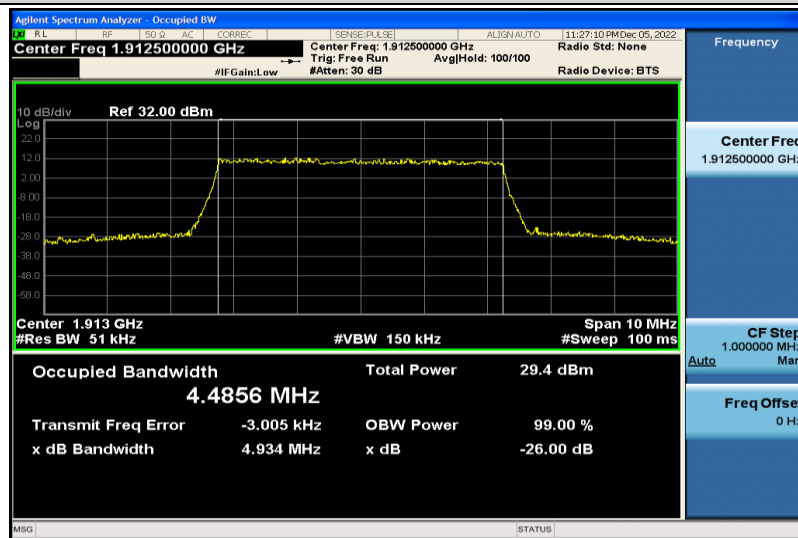
Band25-5MHz-QPSK-26665-25RB#0-4.4856
