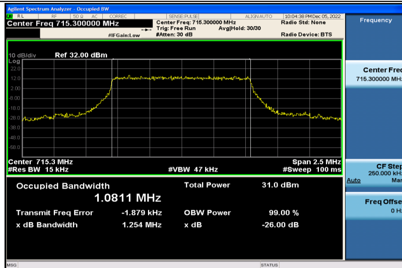
Band12-1.4MHz-QPSK-23173-6RB#0-1.0811
