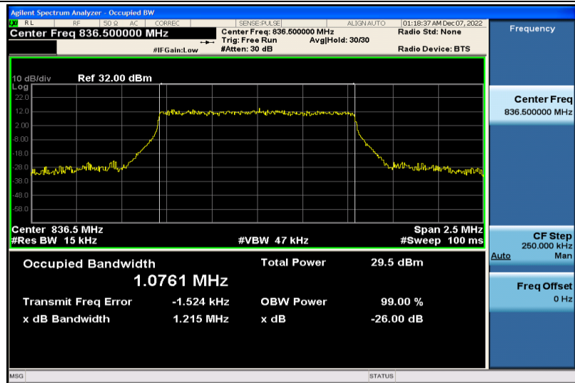
Band26-1.4MHz-16QAM-26915-6RB#0-1.0761
