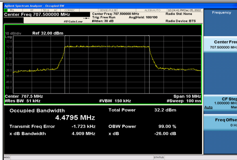
Band12-5MHz-QPSK-23095-25RB#0-4.4795
