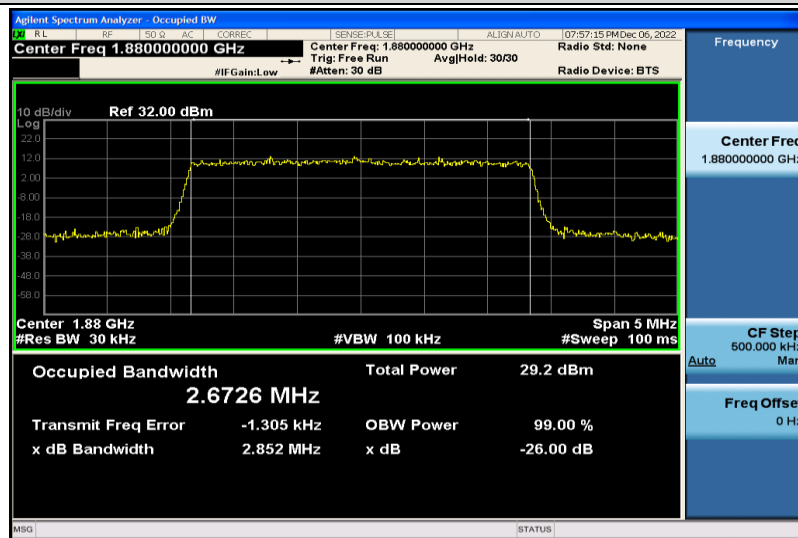
Band2-3MHz-16QAM-18900-15RB#0-2.6726
