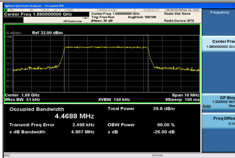
Band2-5MHz-16QAM-18900-25RB#0-4.4688
