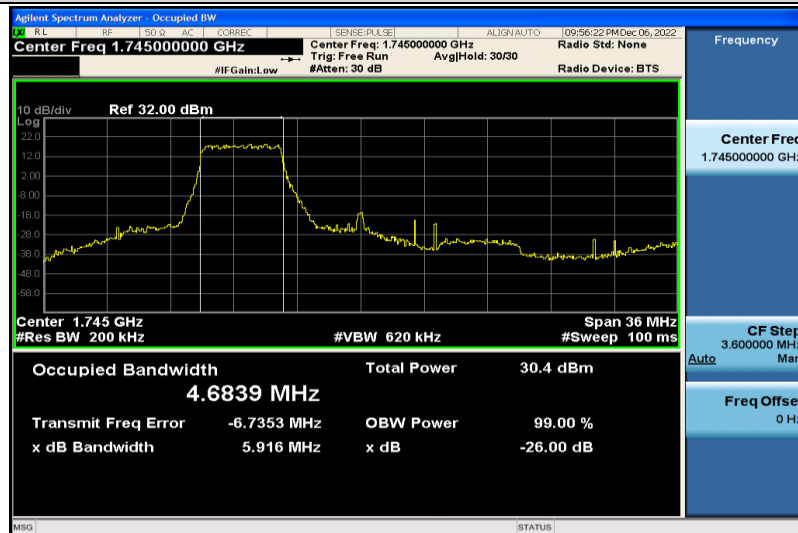
Band4-20MHz-16QAM-20300-25RB#0-4.6839
