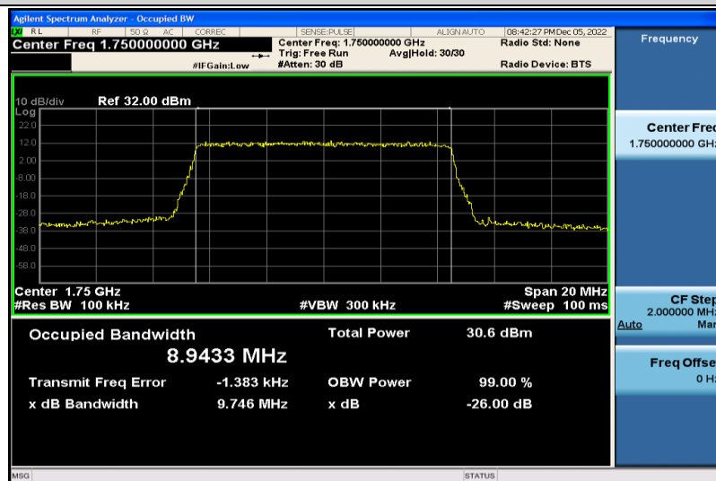
Band4-10MHz-QPSK-20350-50RB#0-8.9433
