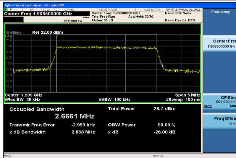
Band2-3MHz-16QAM-19185-15RB#0-2.6661
