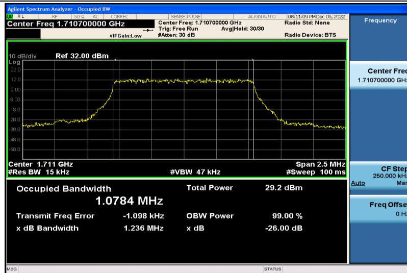
Band4-1.4MHz-QPSK-19957-6RB#0-1.0784
