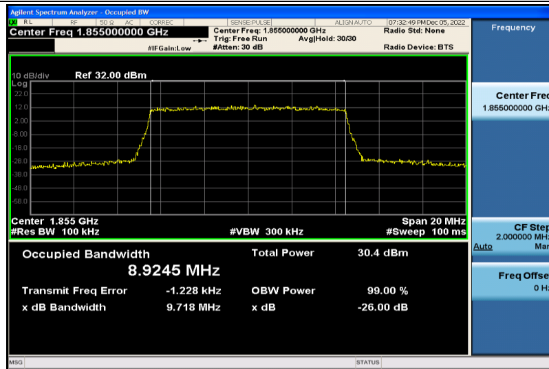
Band2-10MHz-QPSK-18650-50RB#0-8.9245
