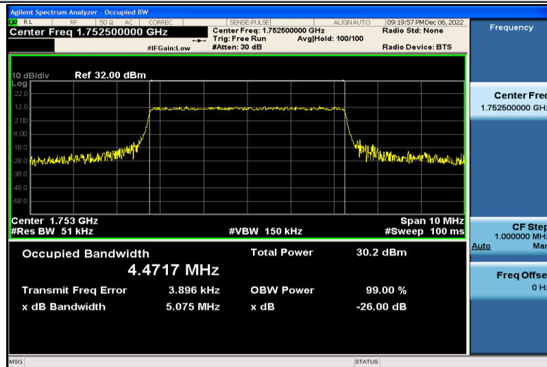
Band4-5MHz-16QAM-20375-25RB#0-4.4717
