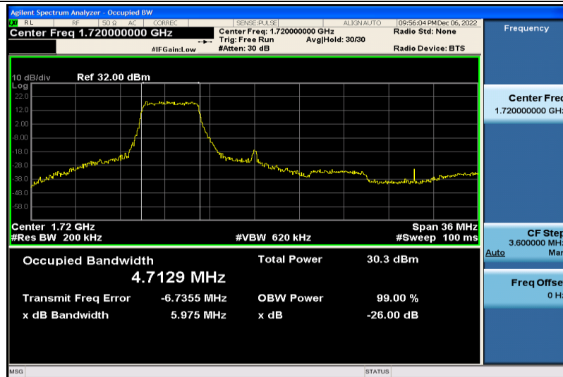
Band4-20MHz-16QAM-20050-25RB#0-4.7129
