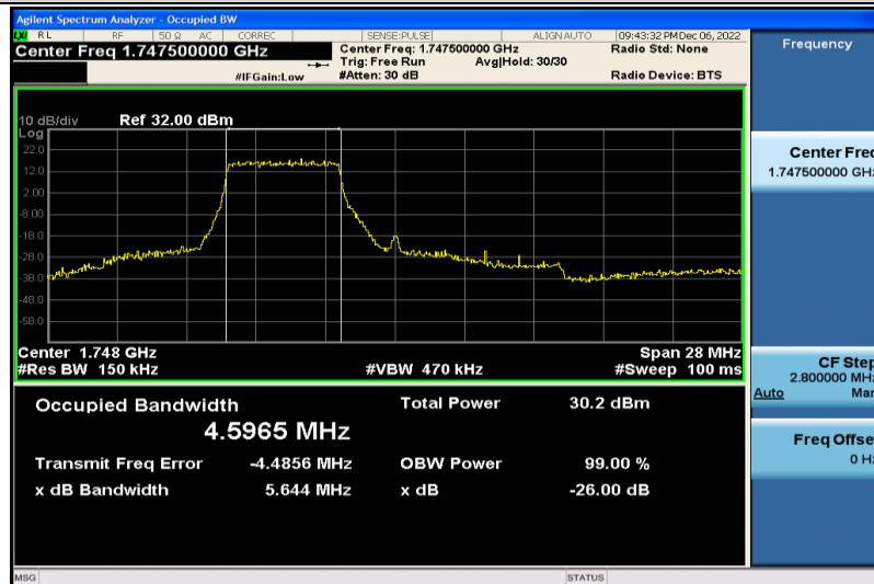
Band4-15MHz-16QAM-20325-25RB#0-4.5965
