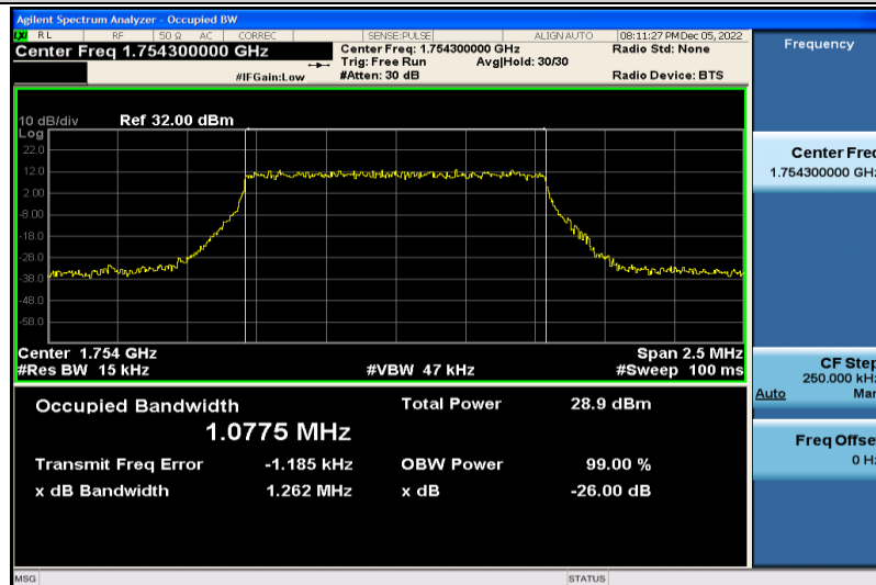
Band4-1.4MHz-QPSK-20393-6RB#0-1.0775
