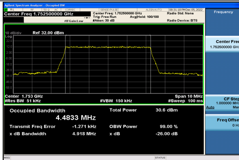
Band4-5MHz-QPSK-20375-25RB#0-4.4833
