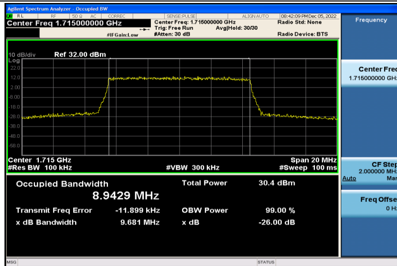
Band4-10MHz-QPSK-20000-50RB#0-8.9429
