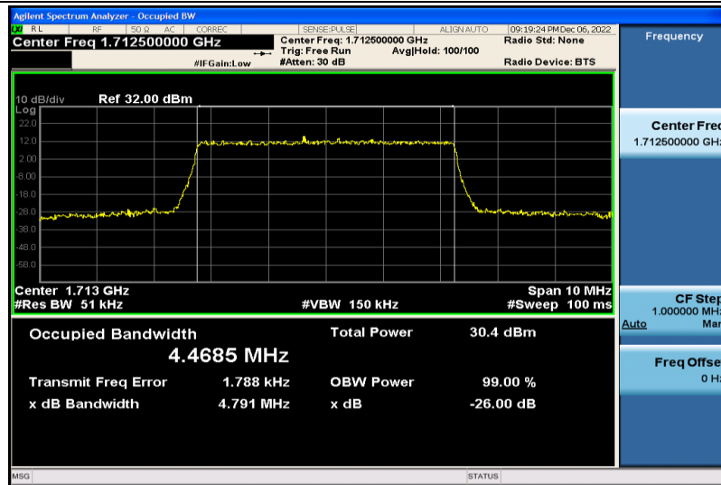
Band4-5MHz-16QAM-19975-25RB#0-4.4685
