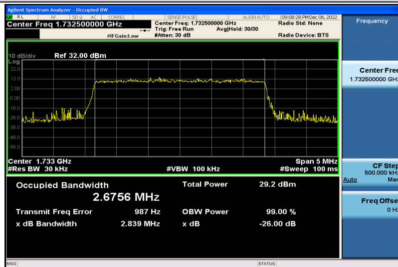
Band4-3MHz-16QAM-20175-15RB#0-2.6756
