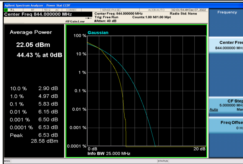
Band26-10MHz-16QAM-26990-25RB#0
