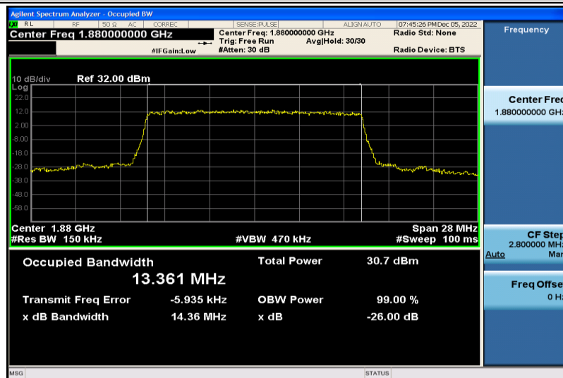
Band2-15MHz-QPSK-18900-75RB#0-13.361
