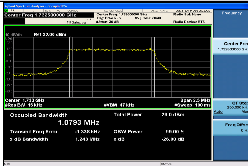
Band4-1.4MHz-QPSK-20175-6RB#0-1.0793
