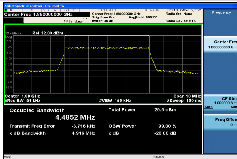
Band2-5MHz-QPSK-18900-25RB#0-4.4852
