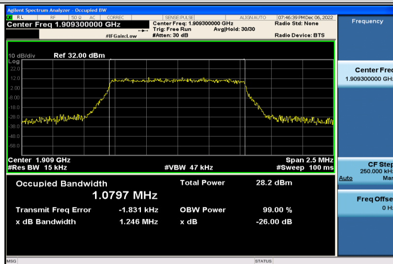
Band2-1.4MHz-16QAM-19193-6RB#0-1.0797
