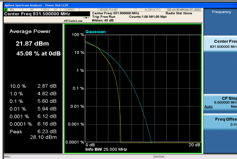
Band26-15MHz-16QAM-26865-25RB#0
