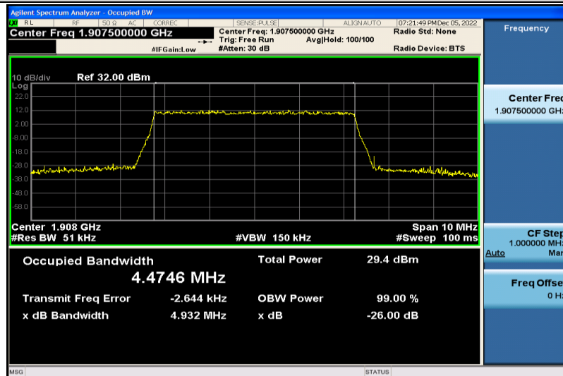
Band2-5MHz-QPSK-19175-25RB#0-4.4746
