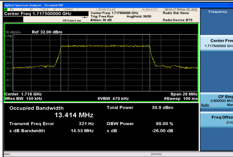
Band4-15MHz-QPSK-20025-75RB#0-13.414
