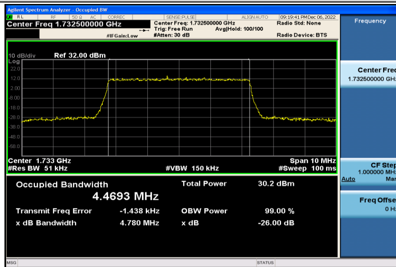
Band4-5MHz-16QAM-20175-25RB#0-4.4693
