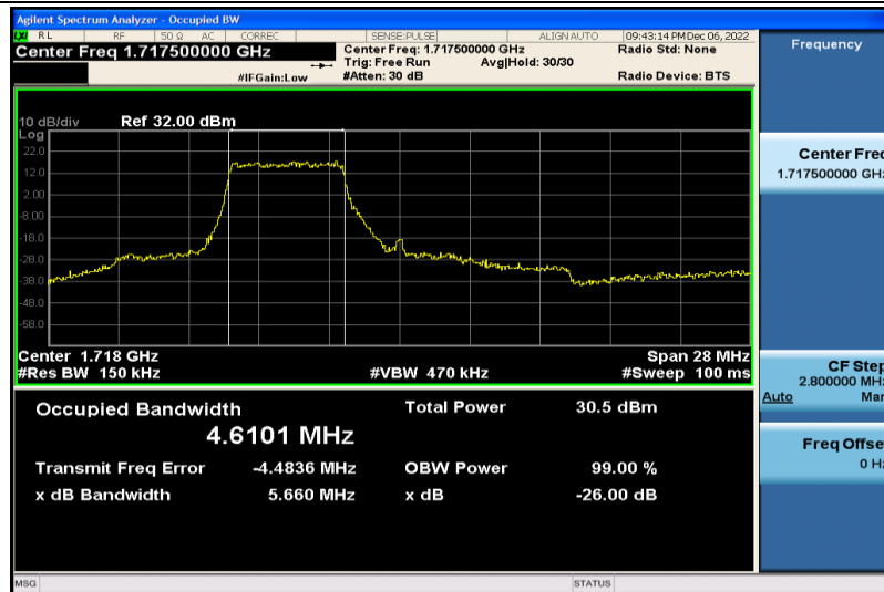
Band4-15MHz-16QAM-20025-25RB#0-4.6101
