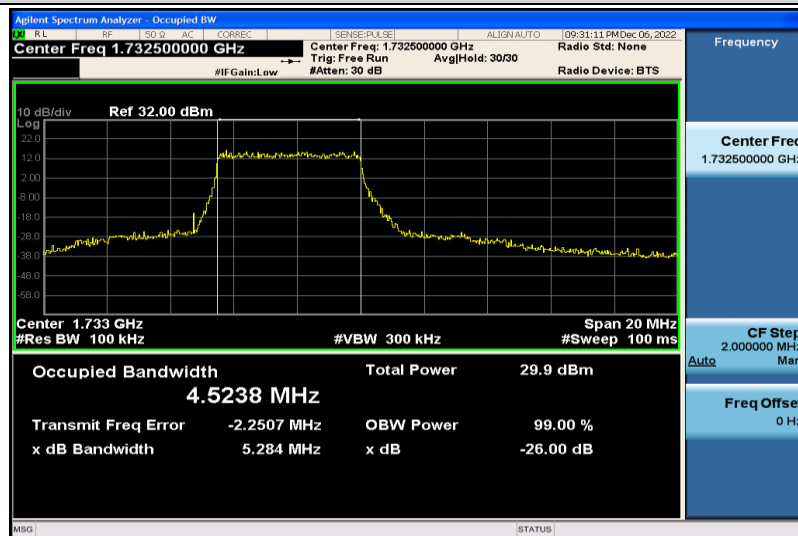
Band4-10MHz-16QAM-20175-25RB#0-4.5238
