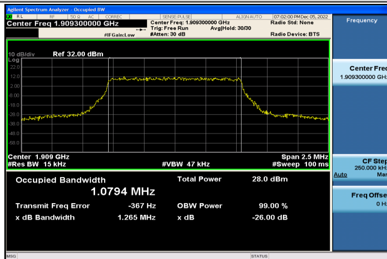
Band2-1.4MHz-QPSK-19193-6RB#0-1.0794
