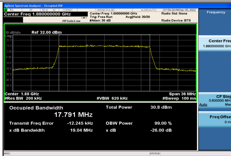
Band2-20MHz-QPSK-18900-100RB#0-17.791
