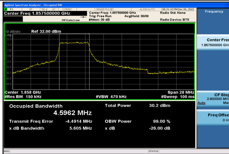
Band2-15MHz-16QAM-18675-25RB#0-4.5962
