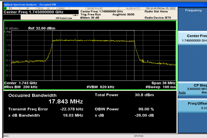
Band4-20MHz-QPSK-20300-100RB#0-17.843
