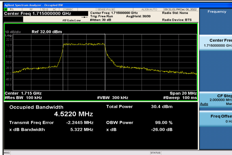
Band4-10MHz-16QAM-20000-25RB#0-4.5220
