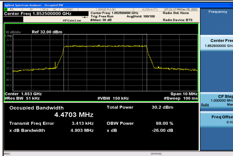
Band2-5MHz-QPSK-18625-25RB#0-4.4703
