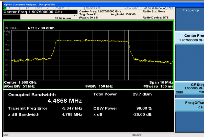
Band2-5MHz-16QAM-19175-25RB#0-4.4656
