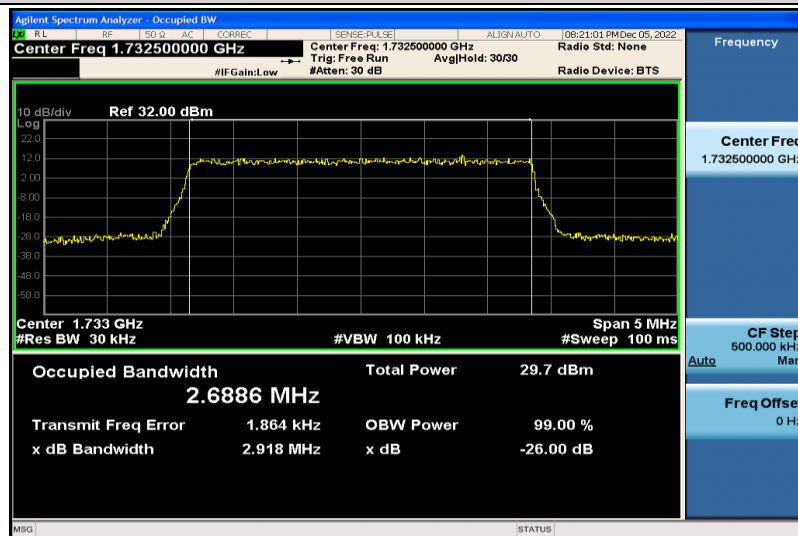
Band4-3MHz-QPSK-20175-15RB#0-2.6886
