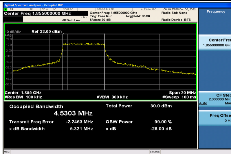
Band2-10MHz-16QAM-18650-25RB#0-4.5303
