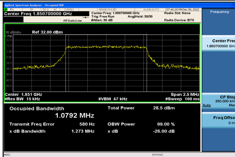
Band2-1.4MHz-16QAM-18607-6RB#0-1.0792
