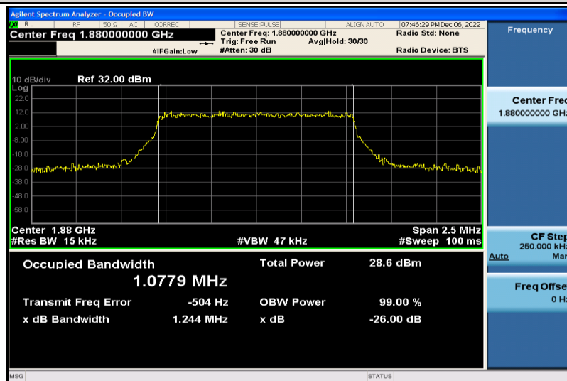
Band2-1.4MHz-16QAM-18900-6RB#0-1.0779
