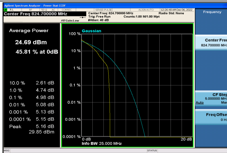
Band26-1.4MHz-QPSK-26797-1RB#0
