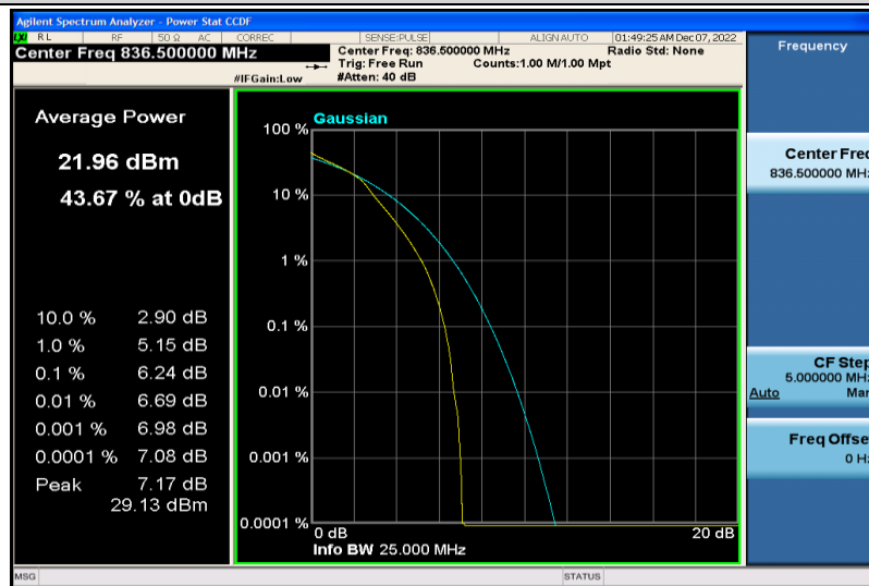
Band26-5MHz-16QAM-26915-25RB#0
