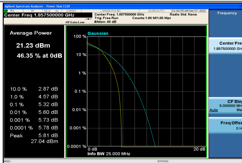
Band25-15MHz-16QAM-26115-25RB#0
