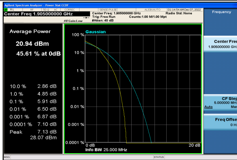
Band25-20MHz-16QAM-26590-25RB#0
