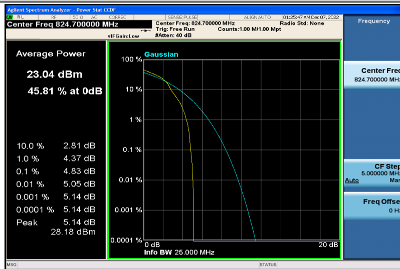
Band26-1.4MHz-16QAM-26797-1RB#0
