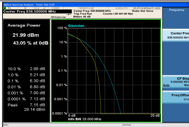
Band26-3MHz-16QAM-26915-15RB#0
