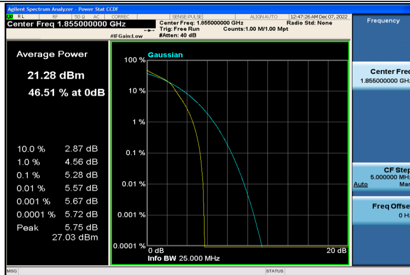
Band25-10MHz-16QAM-26090-25RB#0
