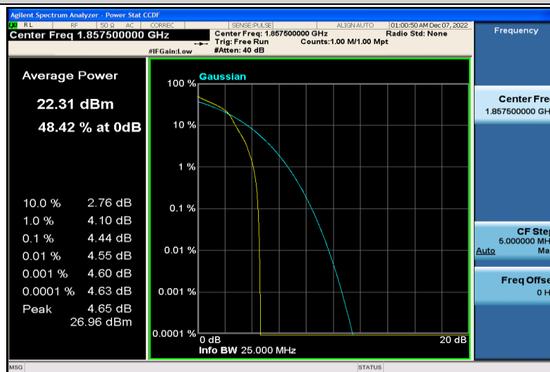
Band25-15MHz-16QAM-26115-1RB#0
