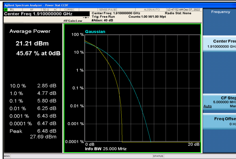
Band25-10MHz-16QAM-26640-25RB#0
