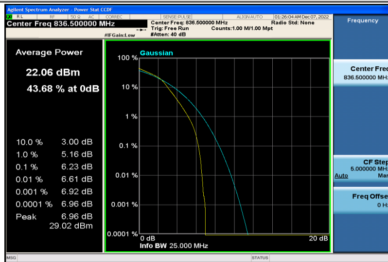
Band26-1.4MHz-16QAM-26915-6RB#0
