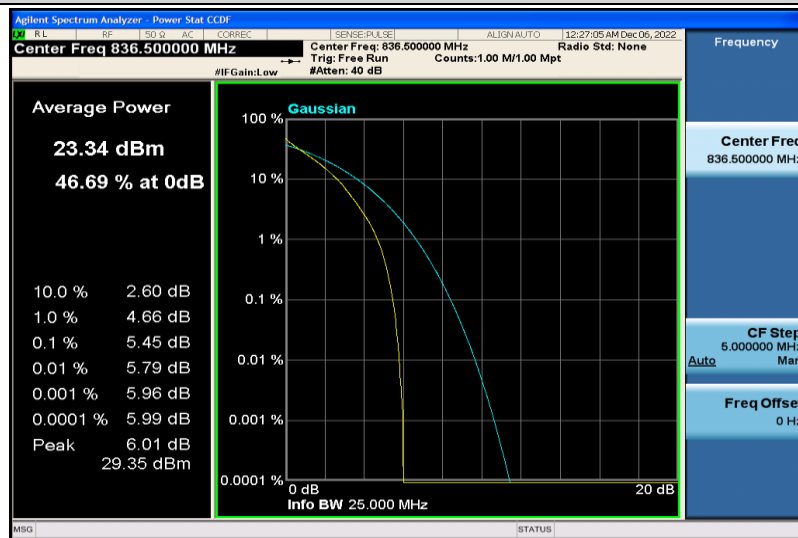
Band26-1.4MHz-QPSK-26915-6RB#0
