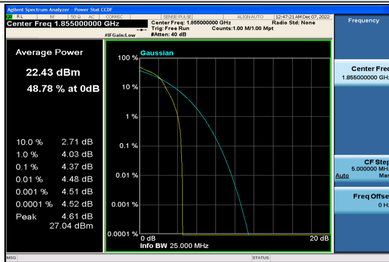
Band25-10MHz-16QAM-26090-1RB#0
