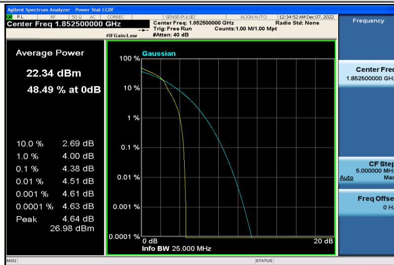
Band25-5MHz-16QAM-26065-1RB#0
