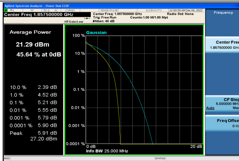
Band25-15MHz-QPSK-26115-1RB#0
