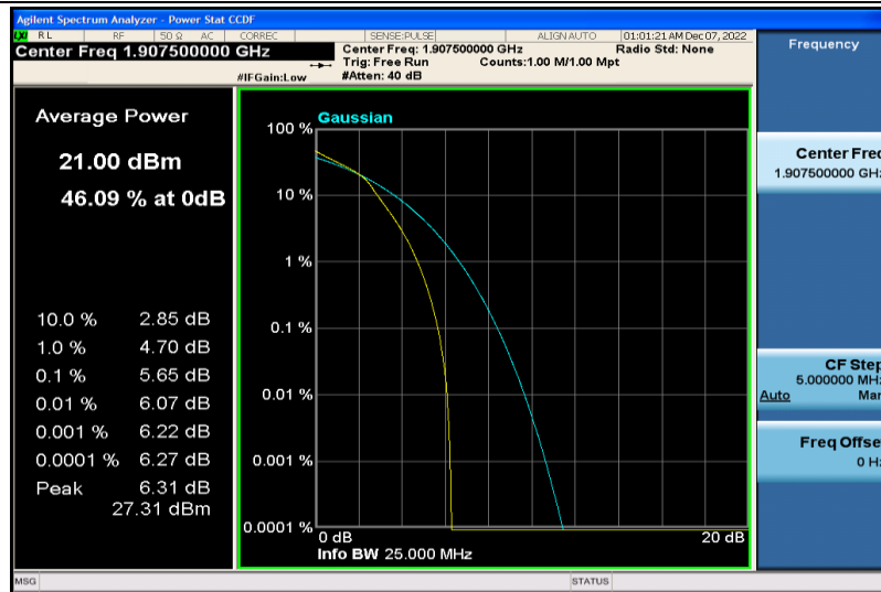
Band25-15MHz-16QAM-26615-25RB#0
