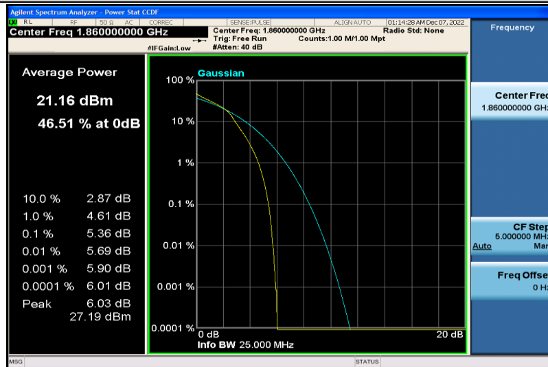
Band25-20MHz-16QAM-26140-25RB#0
