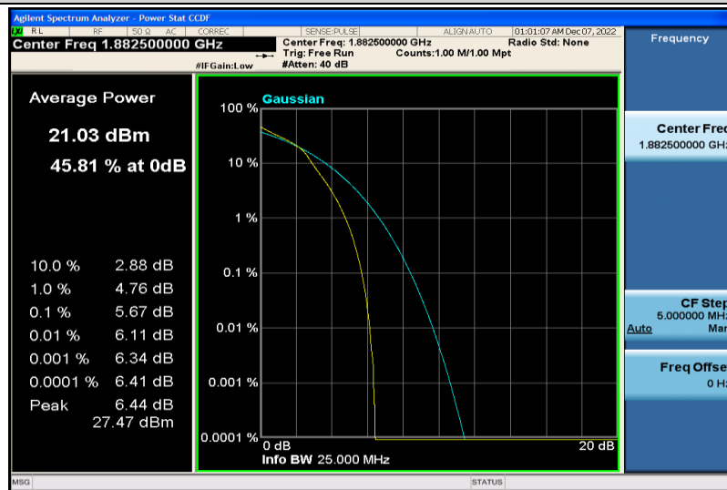
Band25-15MHz-16QAM-26365-25RB#0
