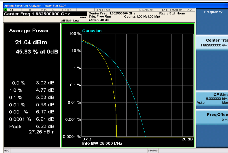
Band25-1.4MHz-16QAM-26365-6RB#0
