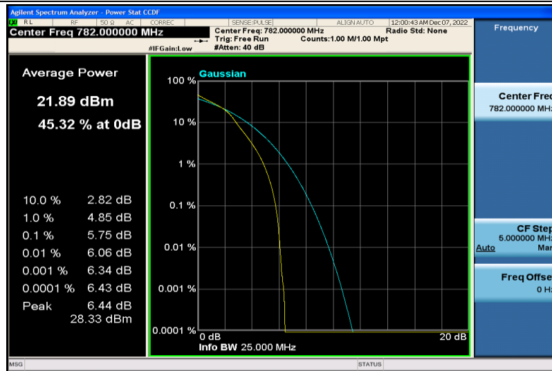
Band13-10MHz-16QAM-23230-25RB#0
