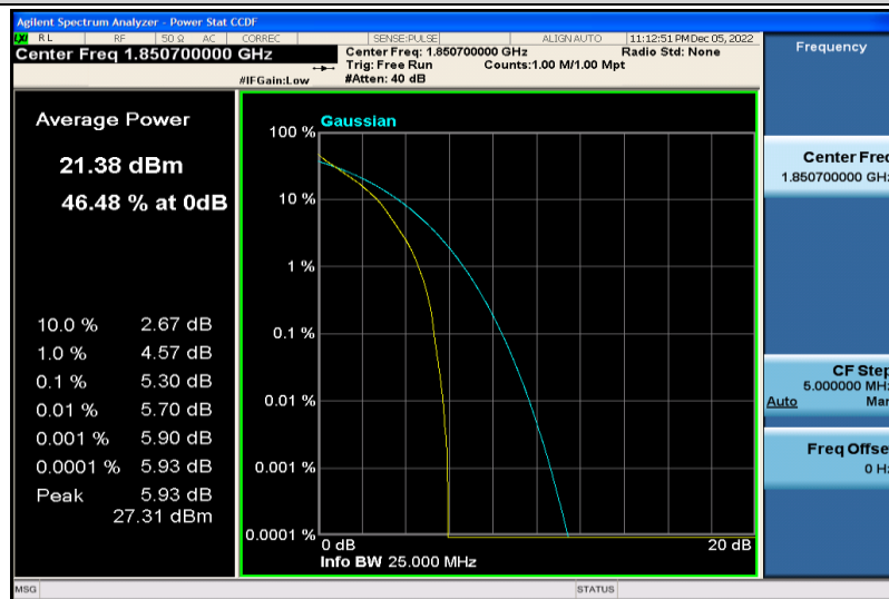
Band25-1.4MHz-QPSK-26047-1RB#0
