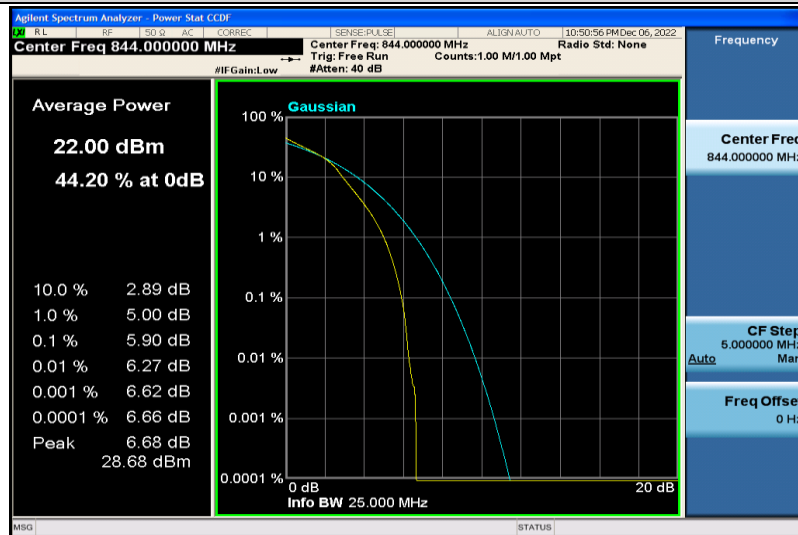
Band5-10MHz-16QAM-20600-25RB#0
