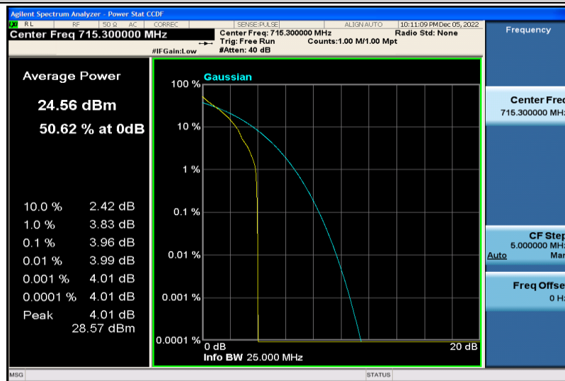
Band12-1.4MHz-QPSK-23173-1RB#0
