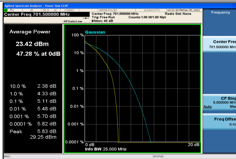
Band12-5MHz-QPSK-23035-25RB#0
