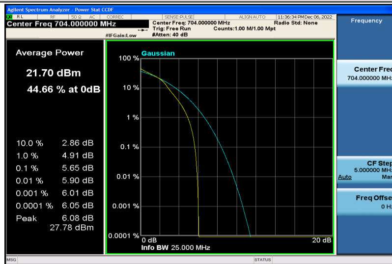
Band12-10MHz-16QAM-23060-25RB#0
