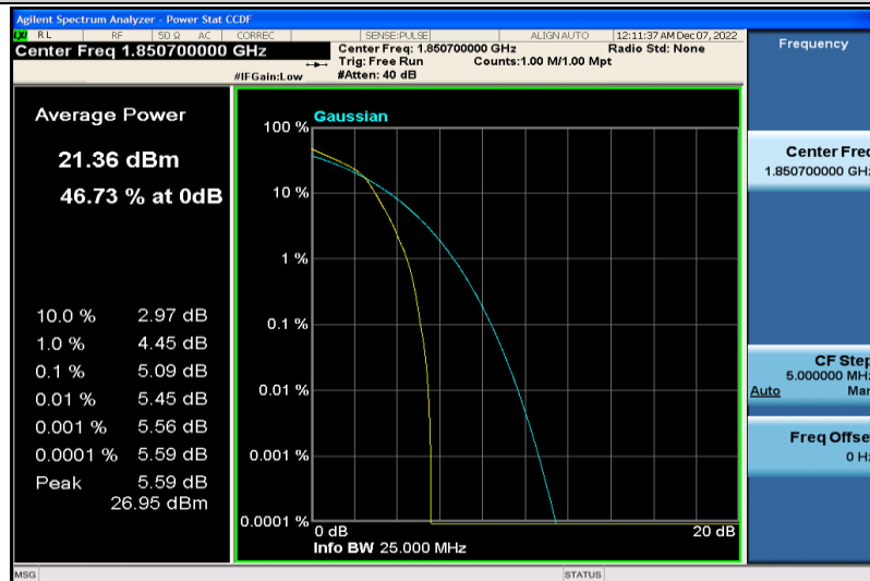
Band25-1.4MHz-16QAM-26047-6RB#0
