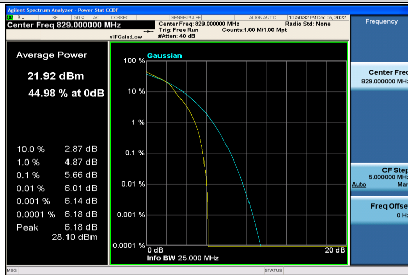
Band5-10MHz-16QAM-20450-25RB#0
