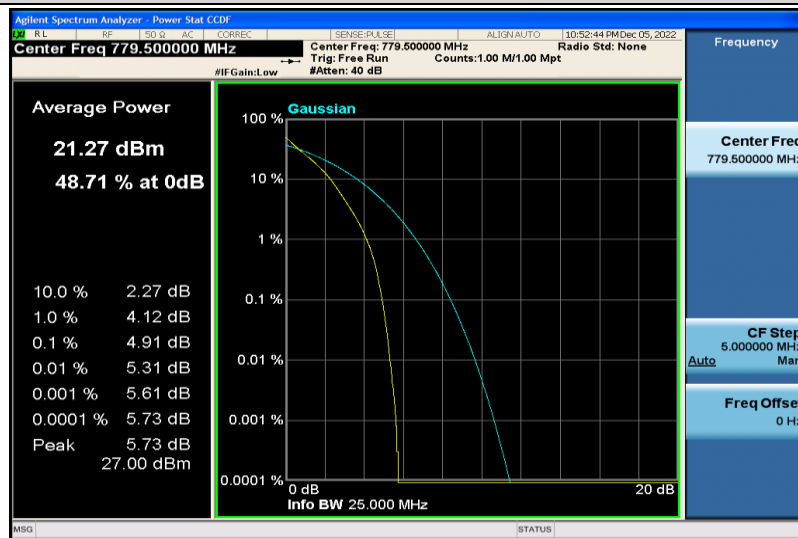
Band13-5MHz-QPSK-23205-25RB#0
