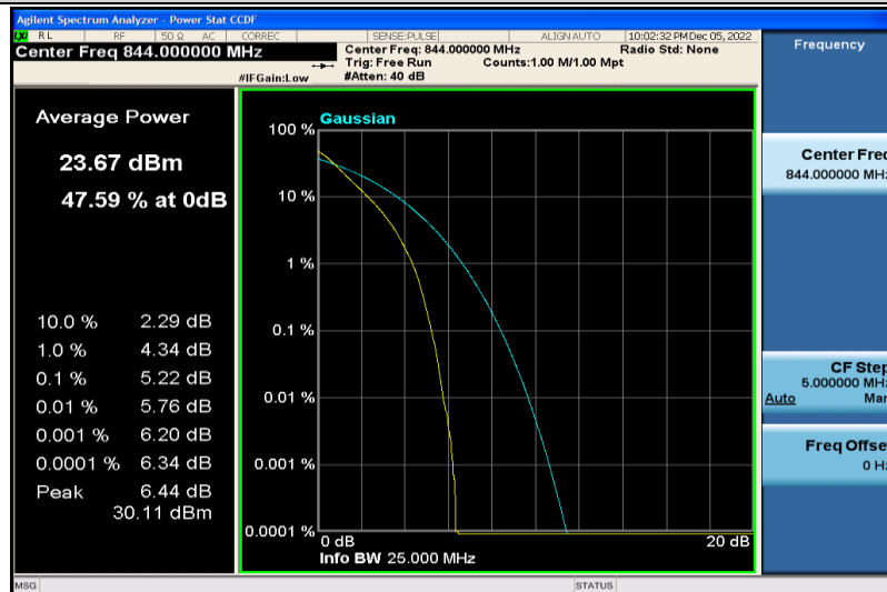
Band5-10MHz-QPSK-20600-50RB#0
