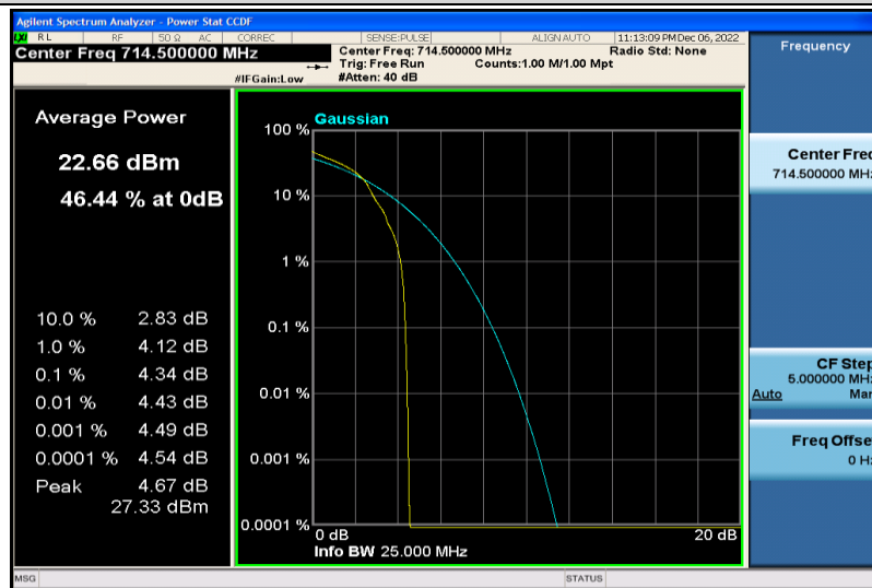
Band12-3MHz-16QAM-23165-1RB#0
