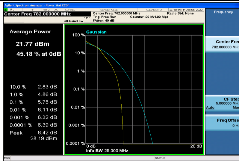
Band13-5MHz-16QAM-23230-25RB#0
