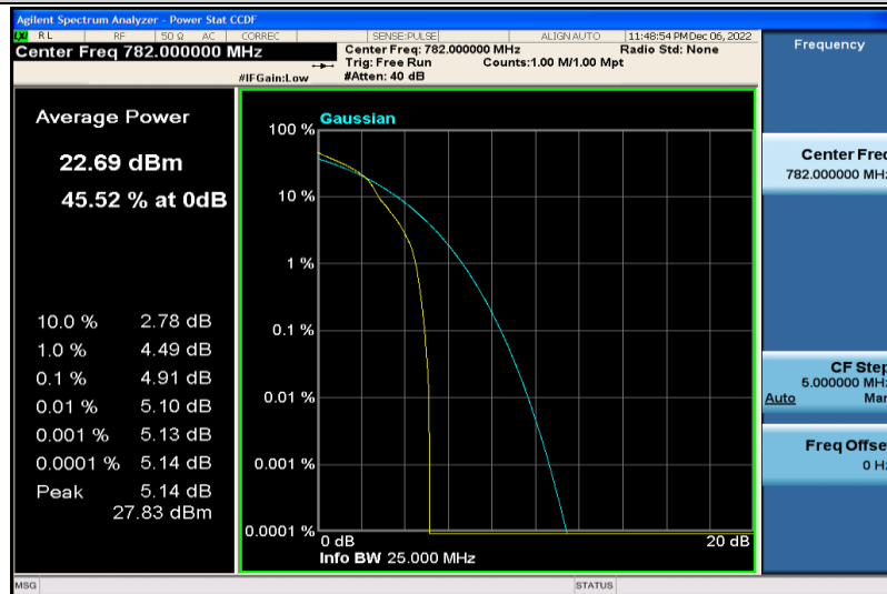
Band13-5MHz-16QAM-23230-1RB#0
