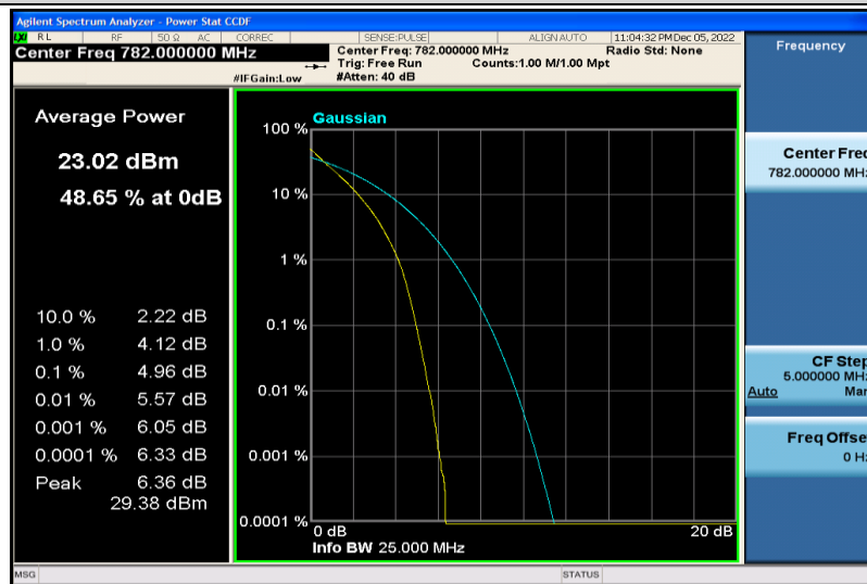
Band13-10MHz-QPSK-23230-50RB#0
