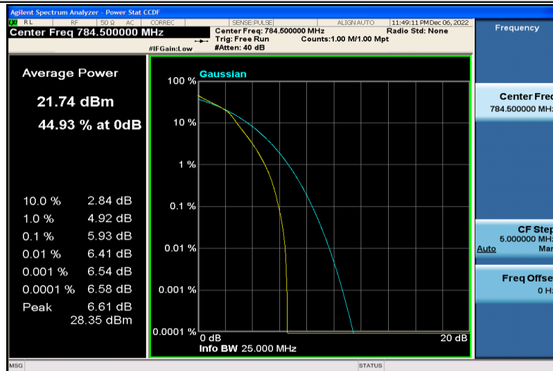
Band13-5MHz-16QAM-23255-25RB#0
