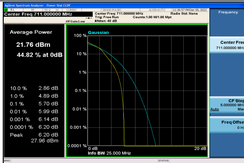
Band12-10MHz-16QAM-23130-25RB#0
