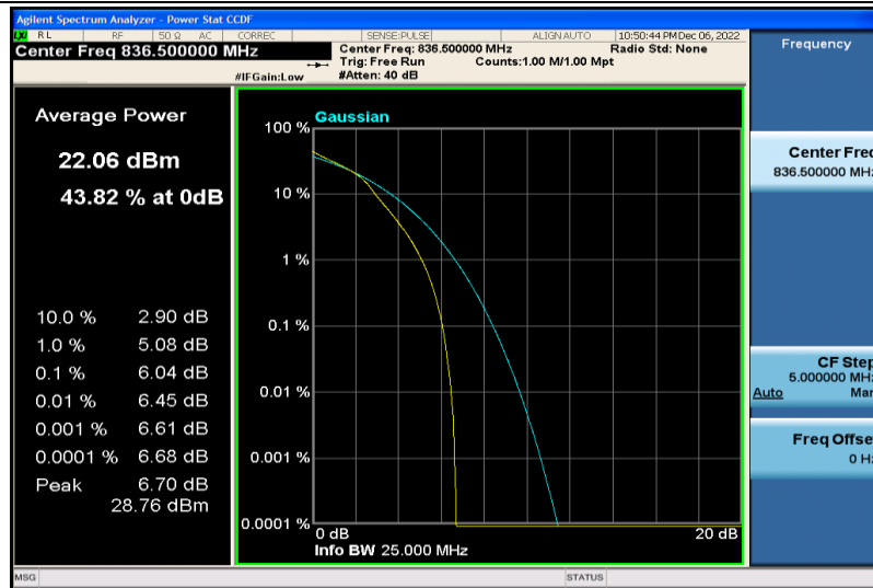
Band5-10MHz-16QAM-20525-25RB#0
