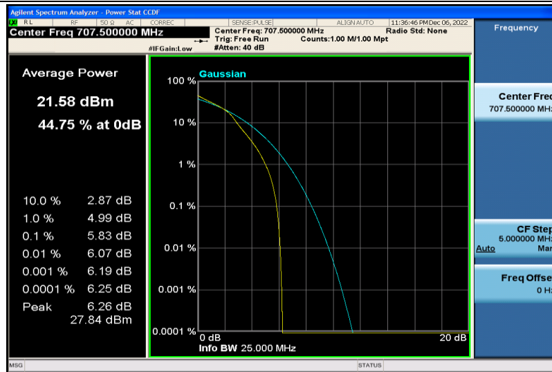
Band12-10MHz-16QAM-23095-25RB#0
