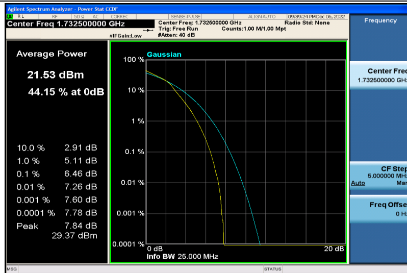
Band4-10MHz-16QAM-20175-25RB#0
