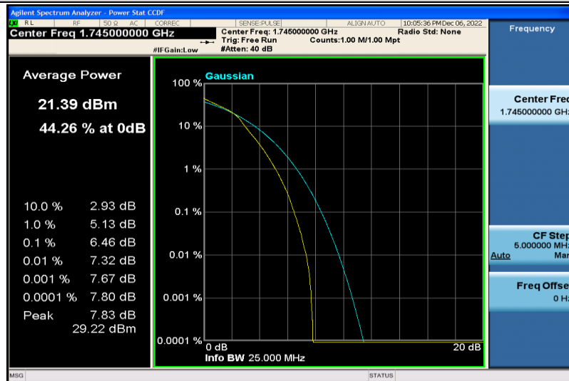
Band4-20MHz-16QAM-20300-25RB#0
