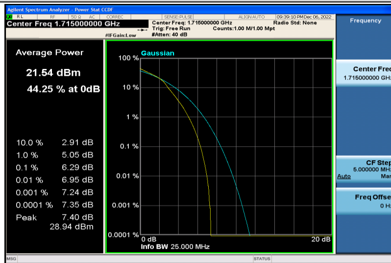
Band4-10MHz-16QAM-20000-25RB#0
