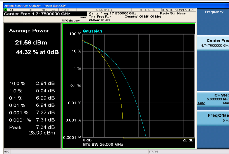
Band4-15MHz-16QAM-20025-25RB#0
