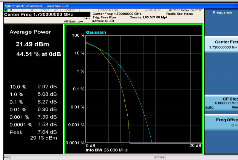
Band4-20MHz-16QAM-20050-25RB#0
