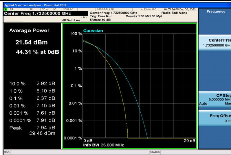
Band4-20MHz-16QAM-20175-25RB#0
