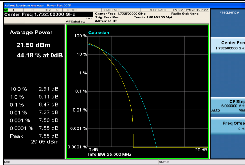
Band4-15MHz-16QAM-20175-25RB#0
