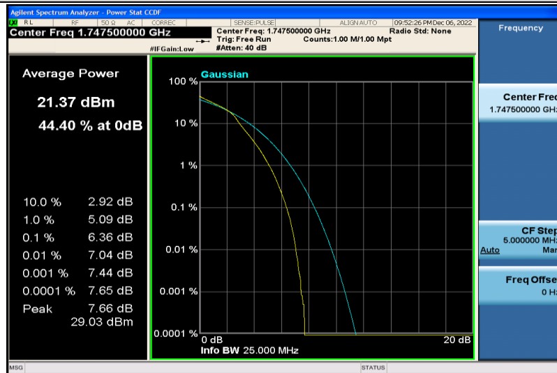
Band4-15MHz-16QAM-20325-25RB#0
