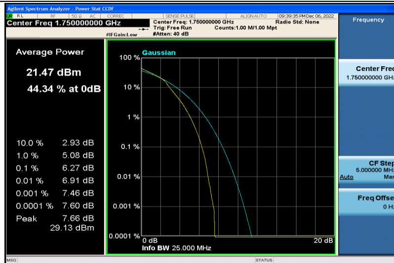
Band4-10MHz-16QAM-20350-25RB#0
