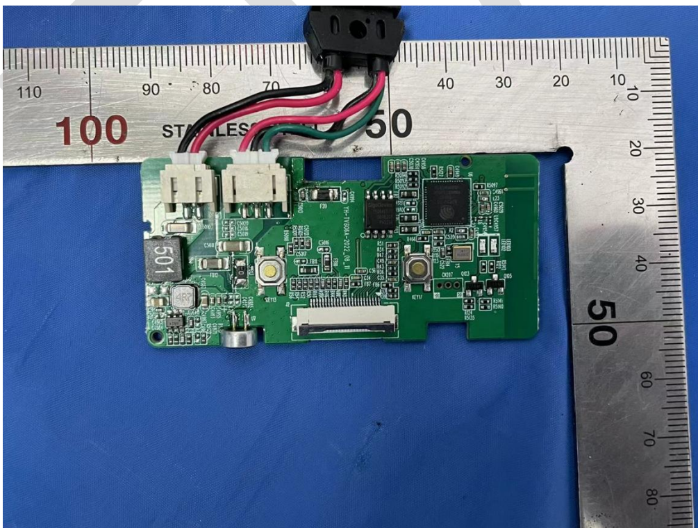
UNCOVER VIEW
