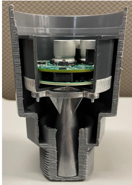
Picture 1- Cut away picture of RLI80.
