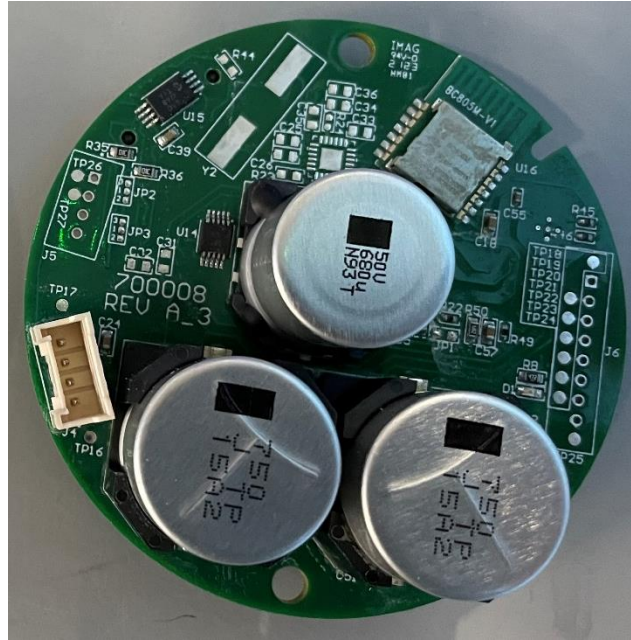
Picture 3 - RLI80 IO board top view
