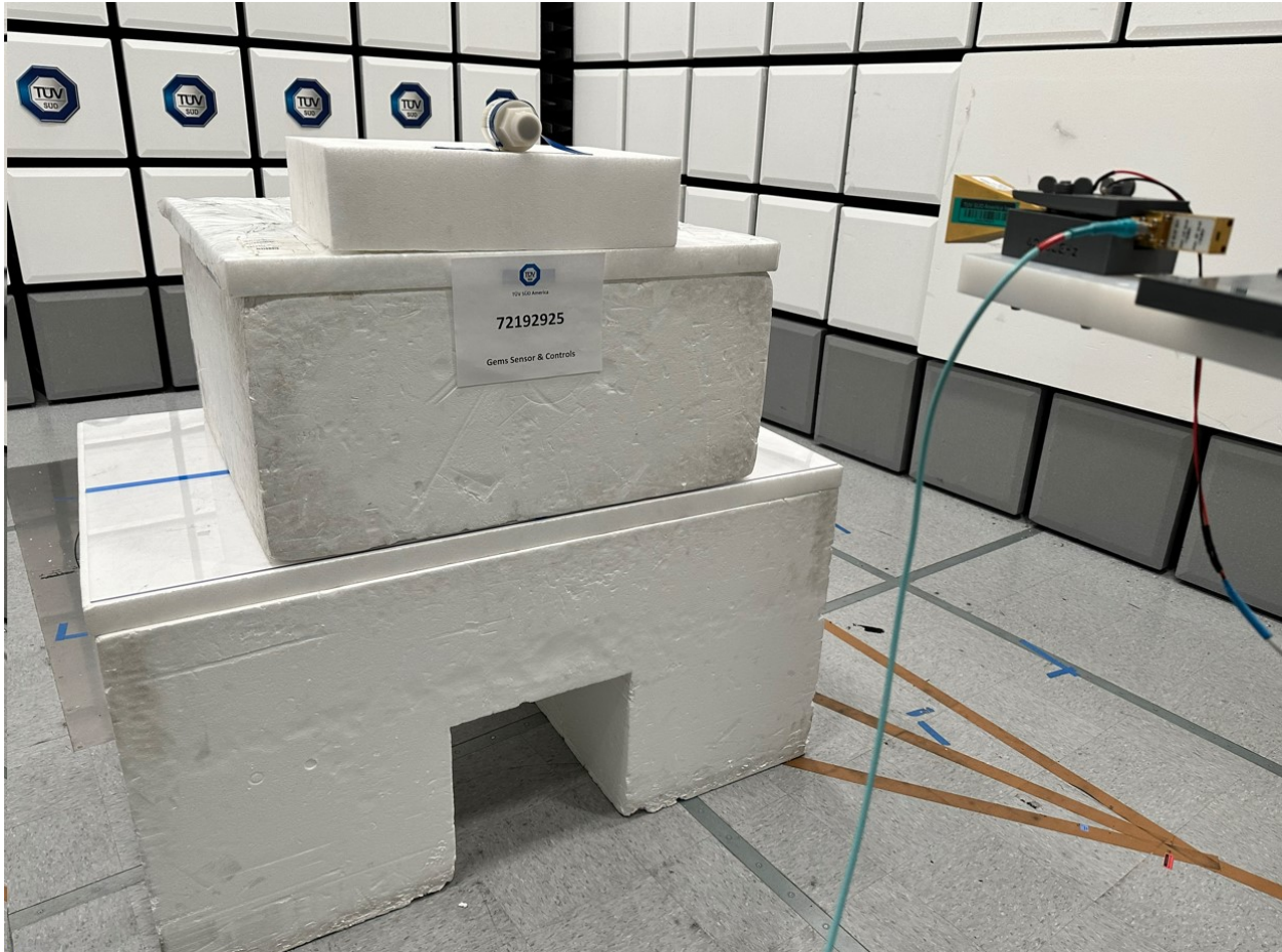
Radiated Emissions Test Setup (40GHz to 60GHz)
