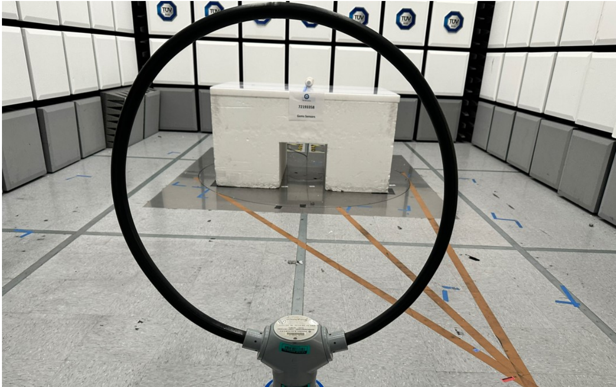
Radiated Emissions Test Setup (9kHz to 30MHz)
