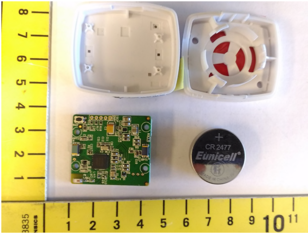
Figure 4 – Internal view 2
