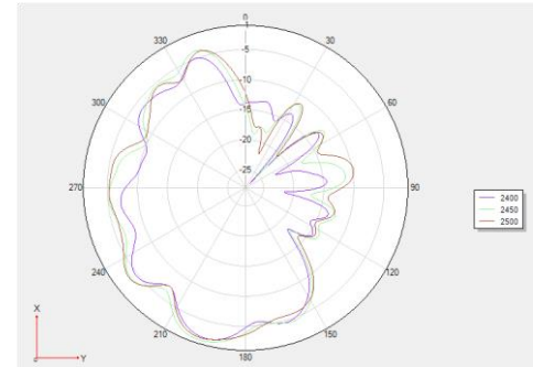
Theta 90° 2D
