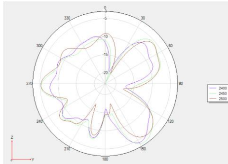
Phi 90° 2D
