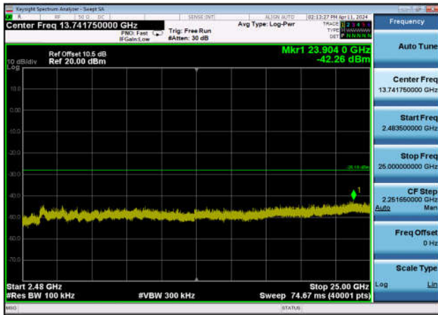
,Plot 4,2483.5MHz~25000MHz-802.11ax(40MHz),2452MHz,Ant13
