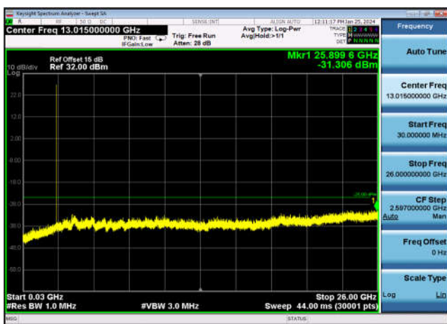
FDD07_HighRange_20MHz_30MHz~26GHz
