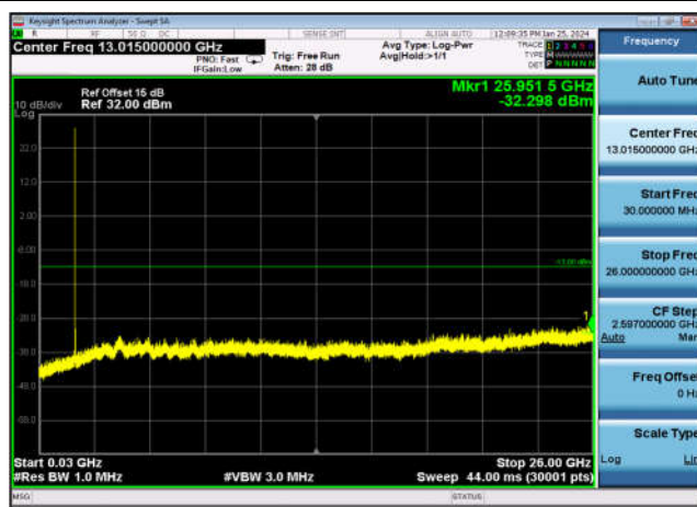
FDD04_HighRange_20MHz_30MHz~26GHz
