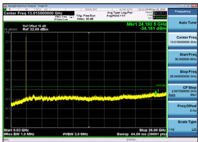
TDD41_LowRange_20MHz_30MHz~26GHz
