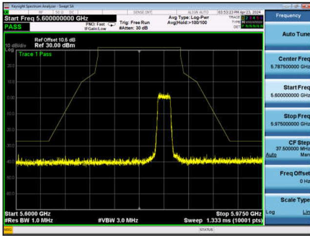
U-NII-3 Band Edge-802.11ax(40MHz) ,5795MHz,Ant1
