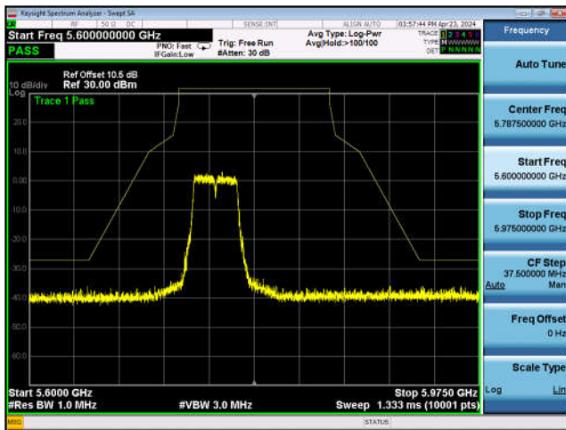
U-NII-3 Band Edge-802.11ac(80MHz) ,5775MHz,Ant1
