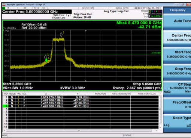
U-NII-2c Band Edge-802.11ax(80MHz) ,5530MHz,Ant1
