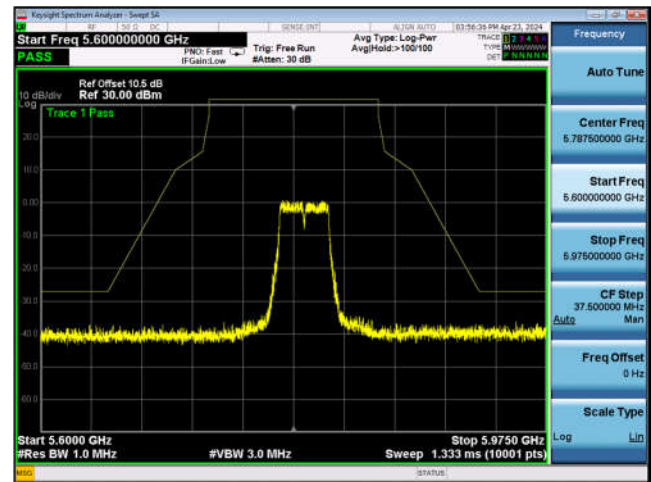
U-NII-3 Band Edge-802.11ax(20MHz) ,5745MHz,Ant1
