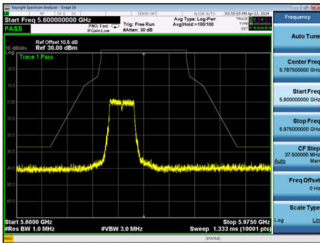
U-NII-3 Band Edge-802.11a(20MHz) ,5745MHz,Ant1
