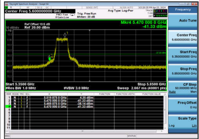
U-NII-2c Band Edge-802.11ac(80MHz) ,5530MHz,Ant1
