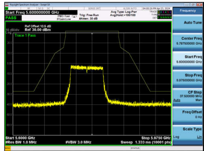
U-NII-3 Band Edge-802.11ax(80MHz) ,5775MHz,Ant1
