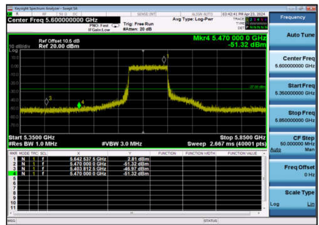
U-NII-2c Band Edge-802.11ax(80MHz) ,5610MHz,Ant1
