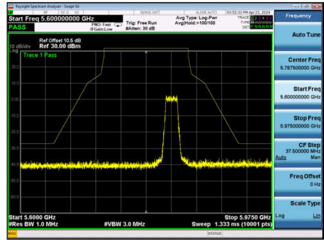
U-NII-3 Band Edge-802.11ac(40MHz) ,5795MHz,Ant1
