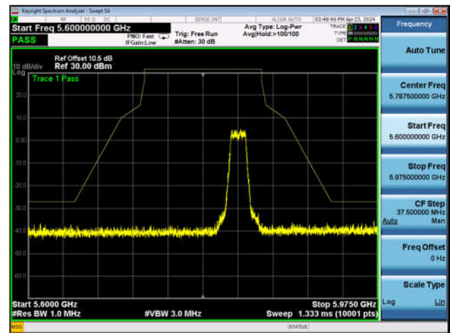
U-NII-3 Band Edge-802.11a(20MHz) ,5825MHz,Ant1
