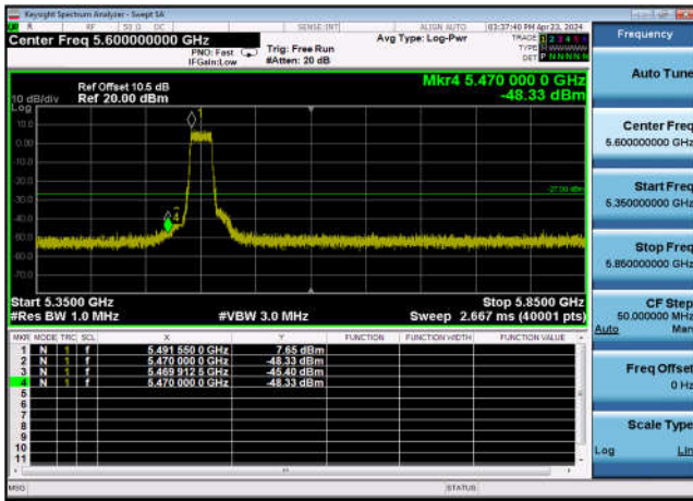
U-NII-2c Band Edge-802.11ax(40MHz) ,5510MHz,Ant1
