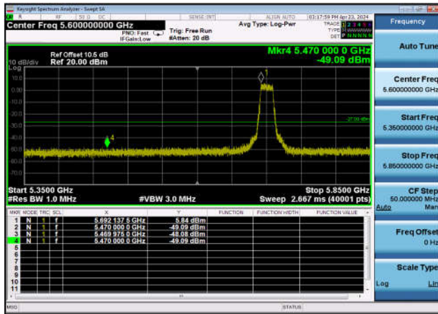
U-NII-2c Band Edge-802.11ac(40MHz) ,5670MHz,Ant1
