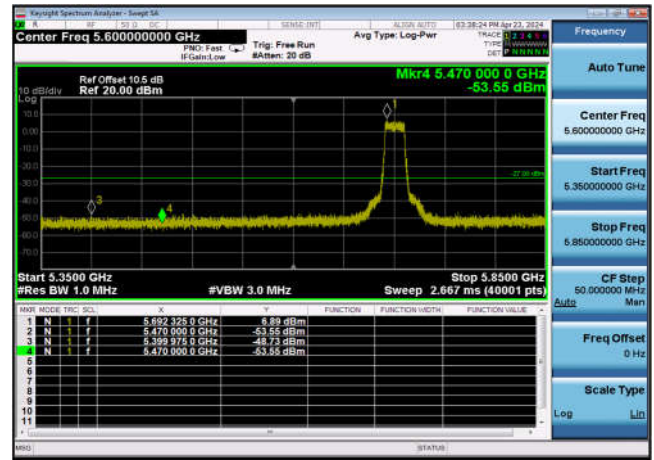
U-NII-2c Band Edge-802.11ax(40MHz) ,5670MHz,Ant1
