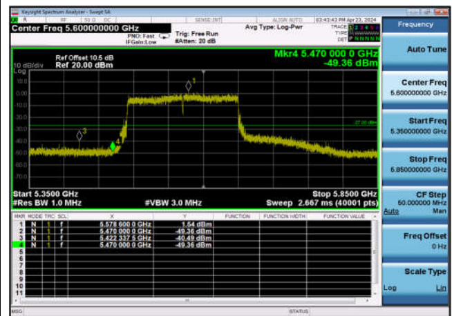
U-NII-2c Band Edge-802.11ax(160MHz) ,5570MHz,Ant1
