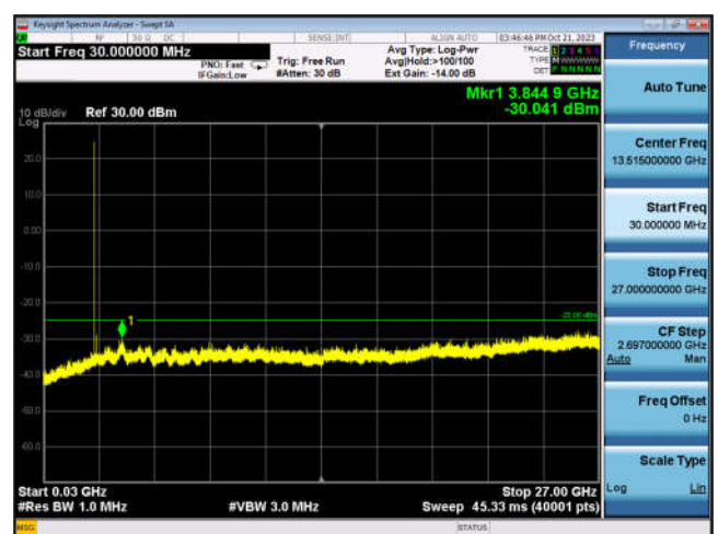
N41_100MHz_DFT-s-OFDM_BPSK_ Edge_1RB_Left_High_CH
