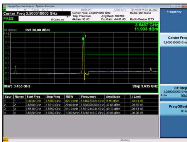
N78_80MHz_DFT-s-OFDM_PI/2-BPSK_Edge_1RB_Right_High_CH
