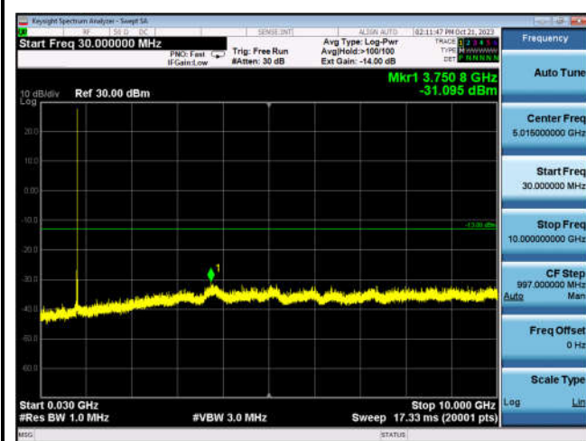
N41_100MHz_DFT-s-OFDM_BPSK_ Edge_1RB_Left_Mid_CH
