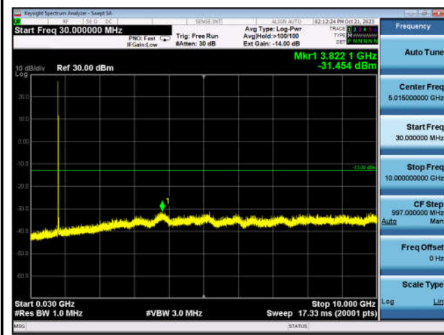
N5_20MHz_DFT-s-OFDM_BPSK_ Edge_1RB_Left_High_CH
