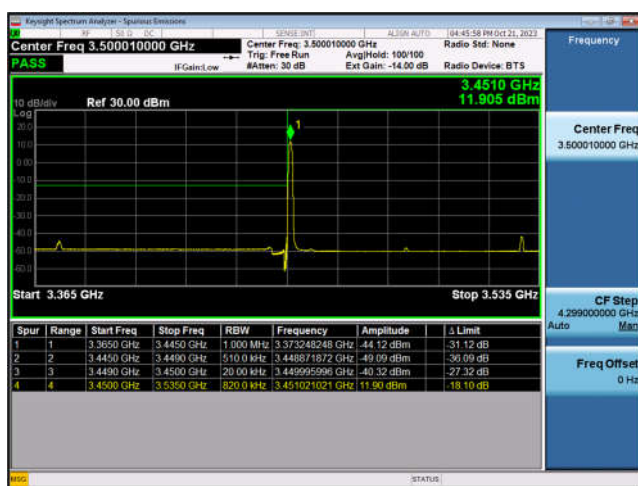
N78_80MHz_DFT-s-OFDM_PI/2-BPSK_Edge_1RB_Right_High_CH
