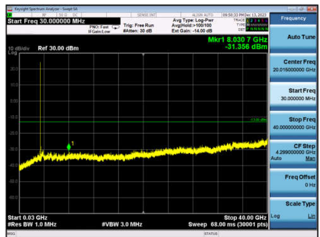
N78_80MHz_DFT-s-OFDM_BPSK_ Edge_1RB_Left_Mid_CH
