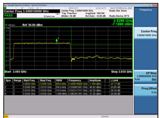
N78_80MHz_DFT-s-OFDM_PI/2-BPSK_Edge_Outer_Full_High_CH
