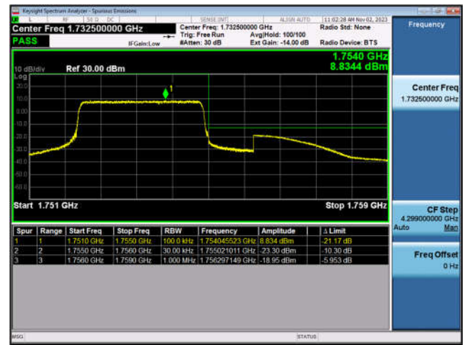
LTE Band 4-5MHz-QPSK-LCH-25RB#0
