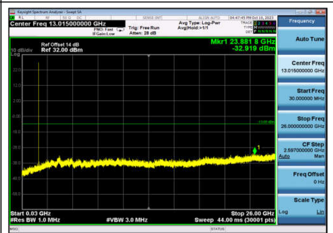
FDD04_HighRange_10MHz_30MHz~26GHz
