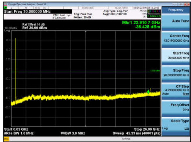
FDD07_LowRange_10MHz_30MHz~26GHz
