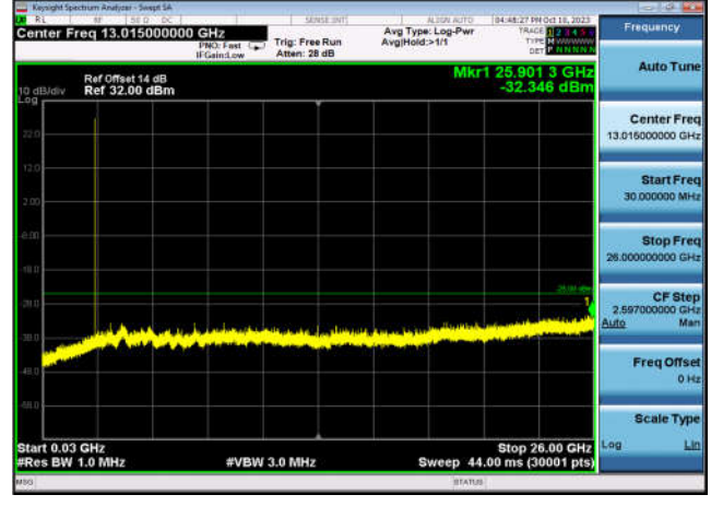
FDD07_HighRange_10MHz_30MHz~26GHz
