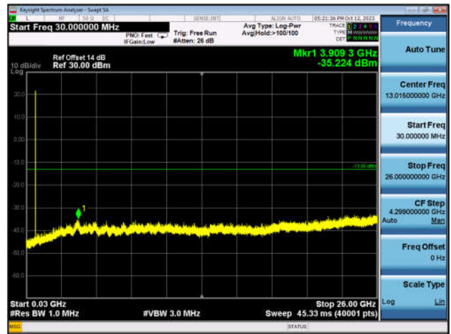
FDD17_LowRange_10MHz_30MHz~26GHz
