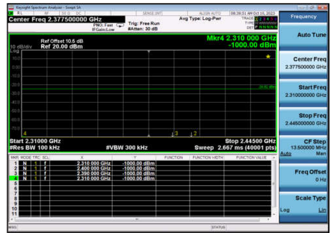
,Plot 2,Band Edge-802.11n(HT40) ,2437MHz,Ant9
