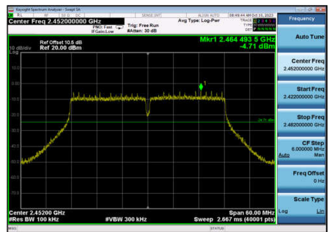
,Plot 1,Reference Level-802.11n(HT40) ,2452MHz,Ant9
