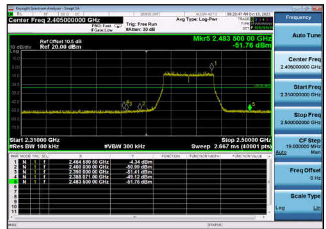
,Plot 2,Band Edge-802.11ax(HT40) ,2452MHz,Ant9
