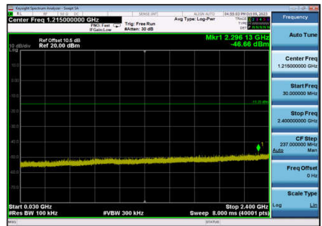
,Plot 3,30MHz~2400MHz-802.11g,2462MHz ,Ant9
