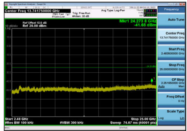
,Plot 4,2483.5MHz~25000MHz-802.11ax(H T40),2437MHz,Ant9
