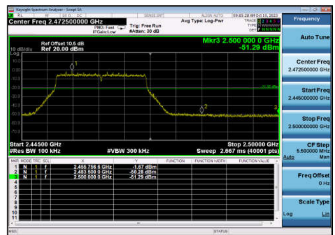
,Plot 2,Band Edge-802.11ax(HT20) ,2462MHz,Ant9
