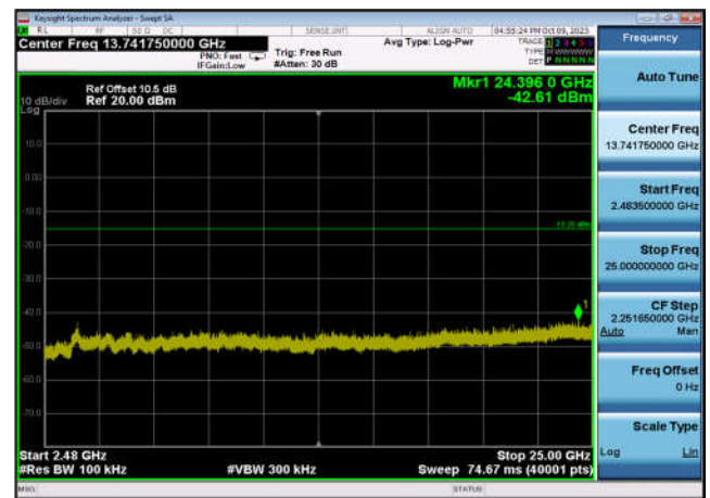
,Plot 4,2483.5MHz~25000MHz-802.11g ,2462MHz,Ant9
