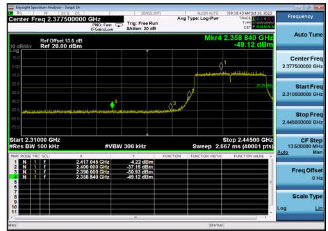
,Plot 2,Band Edge-802.11ax(HT40) ,2437MHz,Ant9
