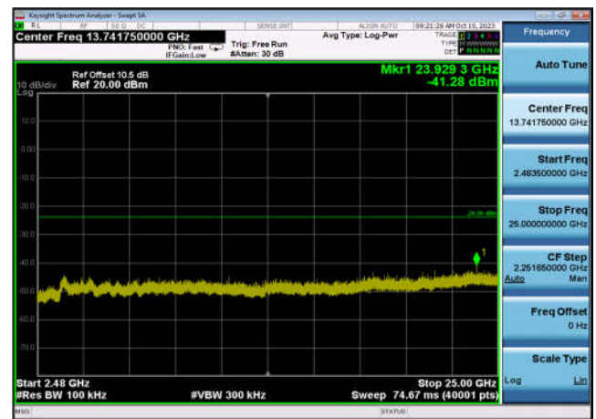
,Plot 4,2483.5MHz~25000MHz-802.11ax(H T40),2452MHz,Ant9
