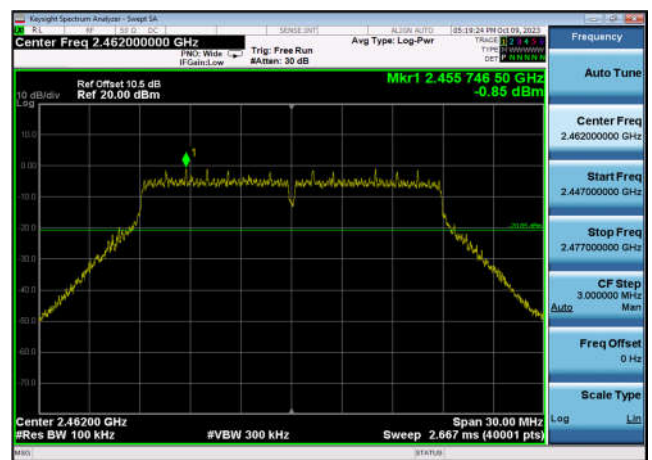
,Plot 1,Reference Level-802.11n(HT20) ,2462MHz,Ant9
