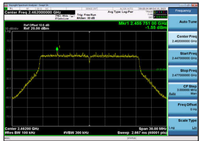
,Plot 1,Reference Level-802.11ax(HT20 ) ,2462MHz,Ant9
