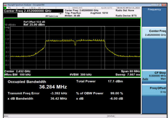
6dB Bandwidth-802.11n(HT40),2452MHz ,Ant9
