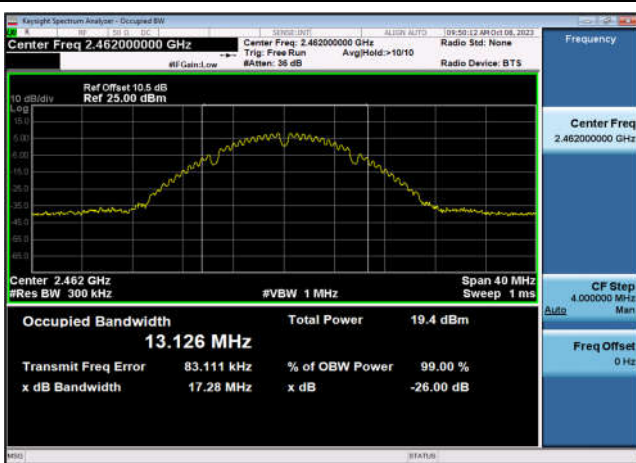
99% Bandwidth-802.11b,2462MHz,Ant7
