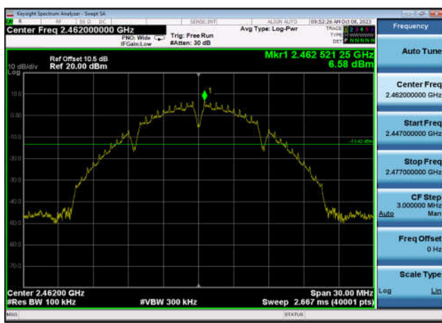
,Plot 1,Reference Level-802.11b ,2462MHz,Ant7
