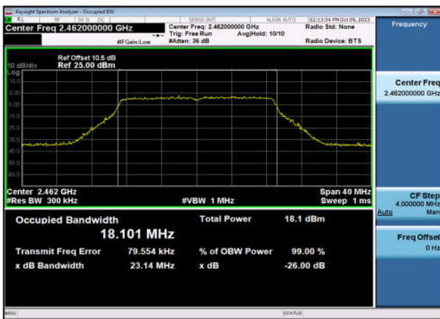
99% Bandwidth-802.11n(HT20),2462MHz ,Ant7
