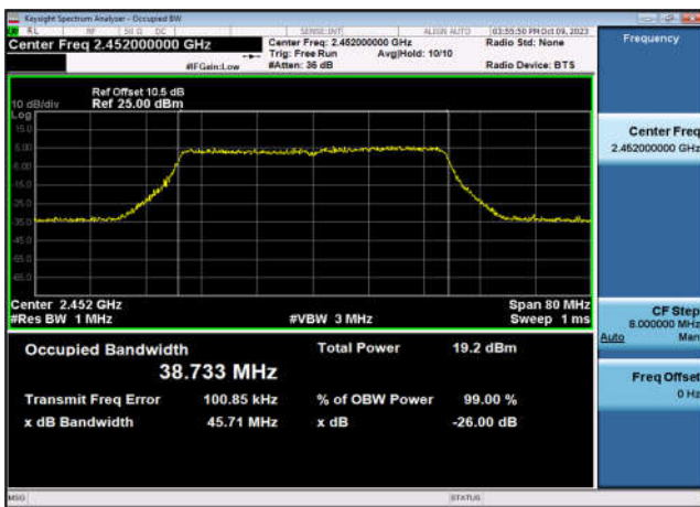
99% Bandwidth-802.11ax(HT40),2452MHz ,Ant7
