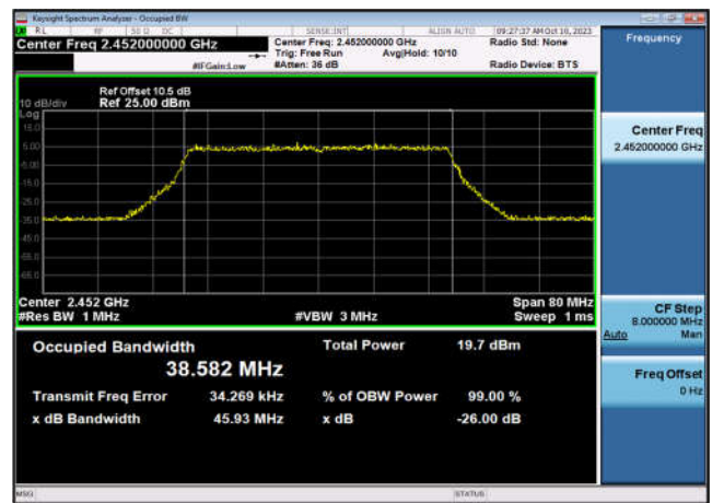
99% Bandwidth-802.11ax(HT40),2452MHz ,Ant9
