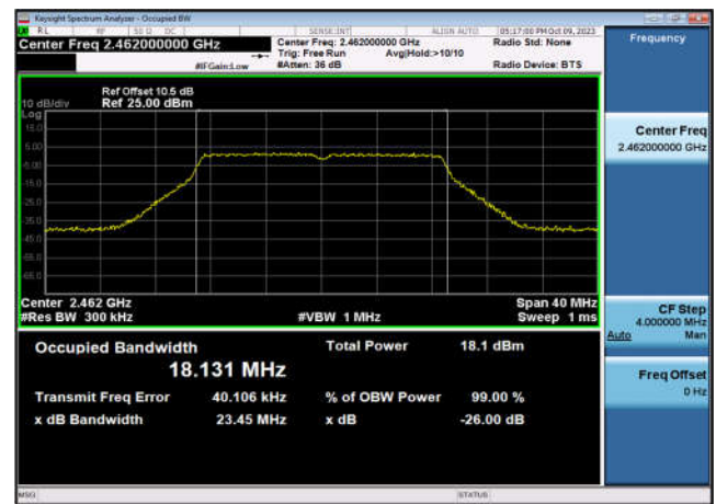
99% Bandwidth-802.11n(HT20),2462MHz ,Ant9
