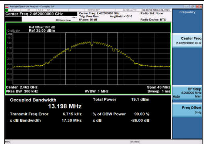
99% Bandwidth-802.11b,2462MHz,Ant9
