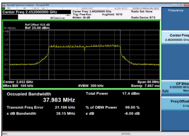
6dB Bandwidth-802.11ax(HT40),2452MHz ,Ant7
