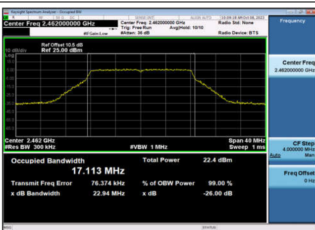
99% Bandwidth-802.11g,2462MHz,Ant7
