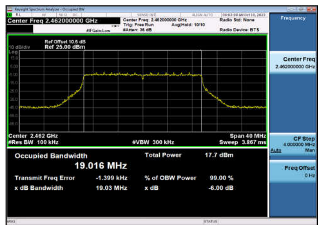
6dB Bandwidth-802.11ax(HT20),2462MHz ,Ant9
