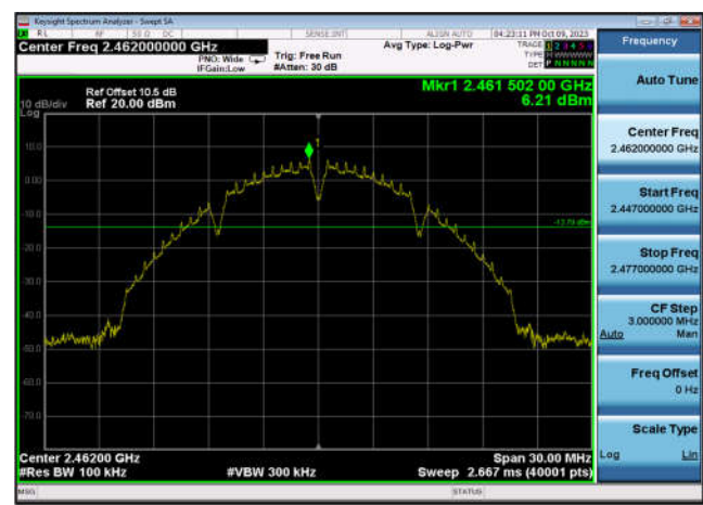
,Plot 1,Reference Level-802.11b ,2462MHz,Ant9
