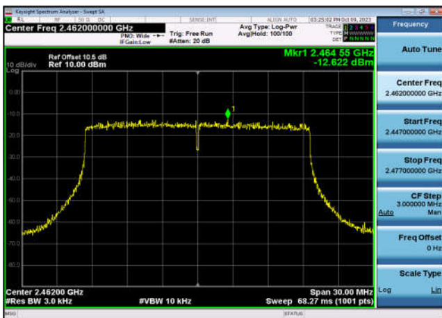
Power spectral density-802.11ax(HT20) ,2462MHz,Ant7
