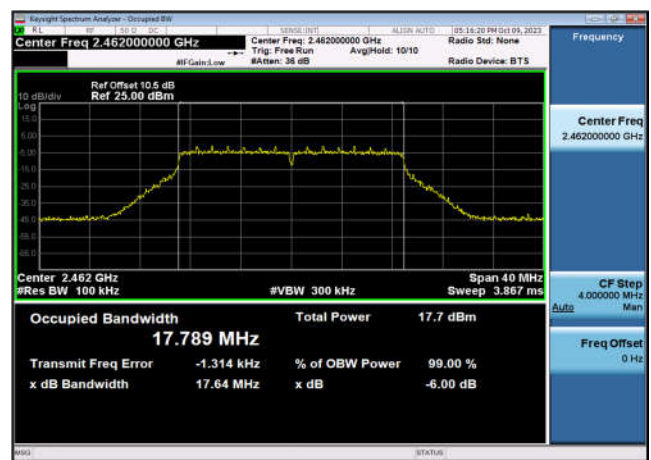
6dB Bandwidth-802.11n(HT20),2462MHz ,Ant9
