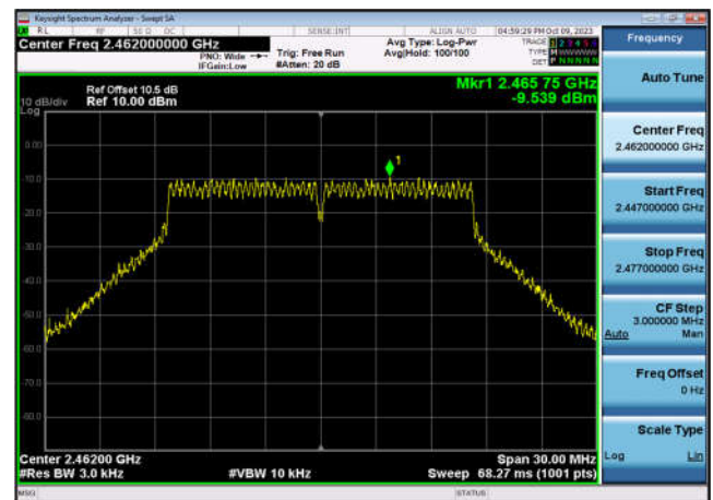
Power spectral density-802.11g ,2462MHz,Ant9
