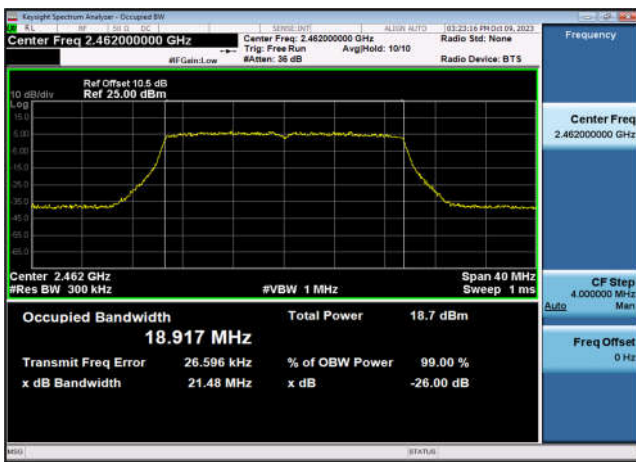
99% Bandwidth-802.11ax(HT20),2462MHz ,Ant7
