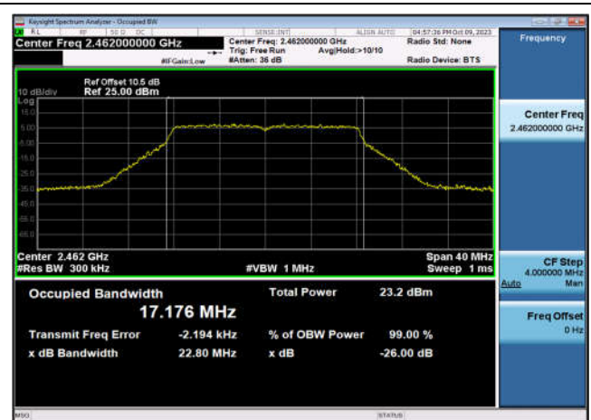
99% Bandwidth-802.11g,2462MHz,Ant9
