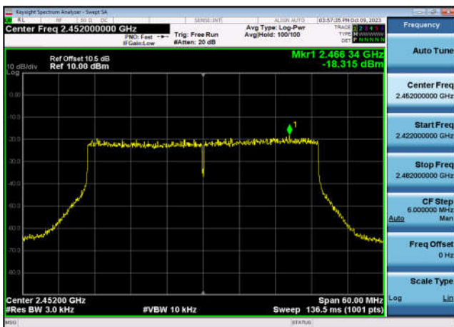
Power spectral density-802.11ax(HT40) ,2452MHz,Ant7
