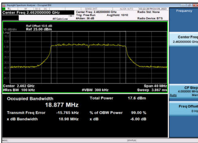
6dB Bandwidth-802.11ax(HT20),2462MHz ,Ant7
