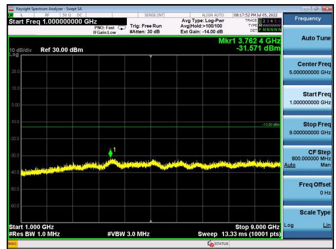
CDMA2000 BC0-384, 1GHz to 9GHz
