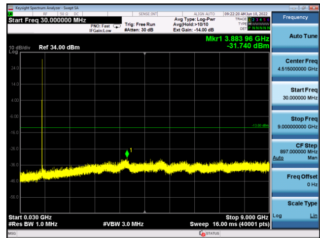
N5(20M)_CP-OFDM_QPSK_ Edge_1RB_Left_Mid_CH
