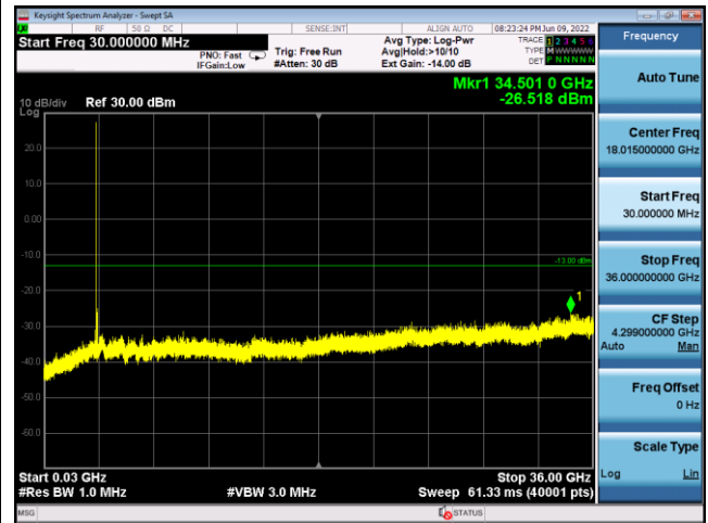
N78(90M)_CP-OFDM_QPSK_ Edge_1RB_Left_Mid_CH
