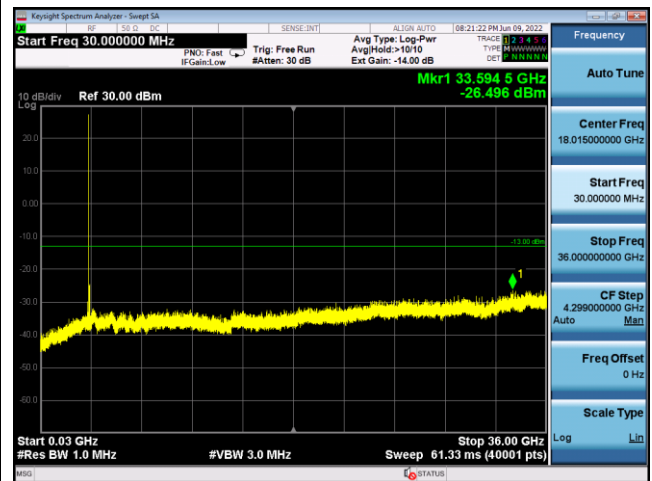
N78(90M)_CP-OFDM_QPSK_ Edge_1RB_Left_High_CH
