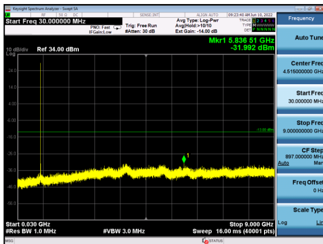
N5(20M)_DFT-s-OFDM_BPSK_ Edge_1RB_Left_High_CH
