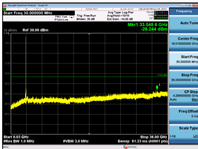
N78(90M)_DFT-s-OFDM_BPSK_ Edge_1RB_Left_High_CH
