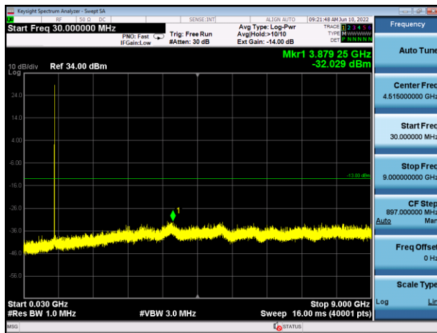
N5(20M)_DFT-s-OFDM_BPSK_ Edge_1RB_Left_Mid_CH
