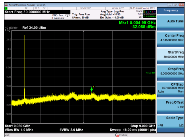
N5(20M)_CP-OFDM_QPSK_ Edge_1RB_Left_High_CH
