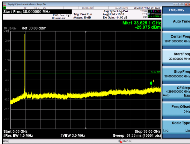
N78(90M)_DFT-s-OFDM_BPSK_ Edge_1RB_Left_Mid_CH
