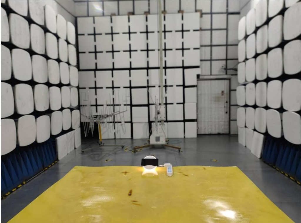
Radiated Emission from 30MHz to 1GHz
