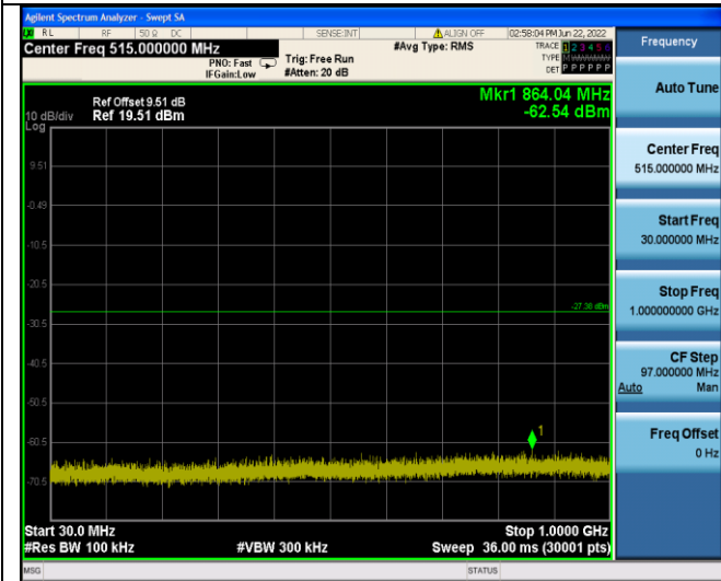
802.11b on Channel 11
