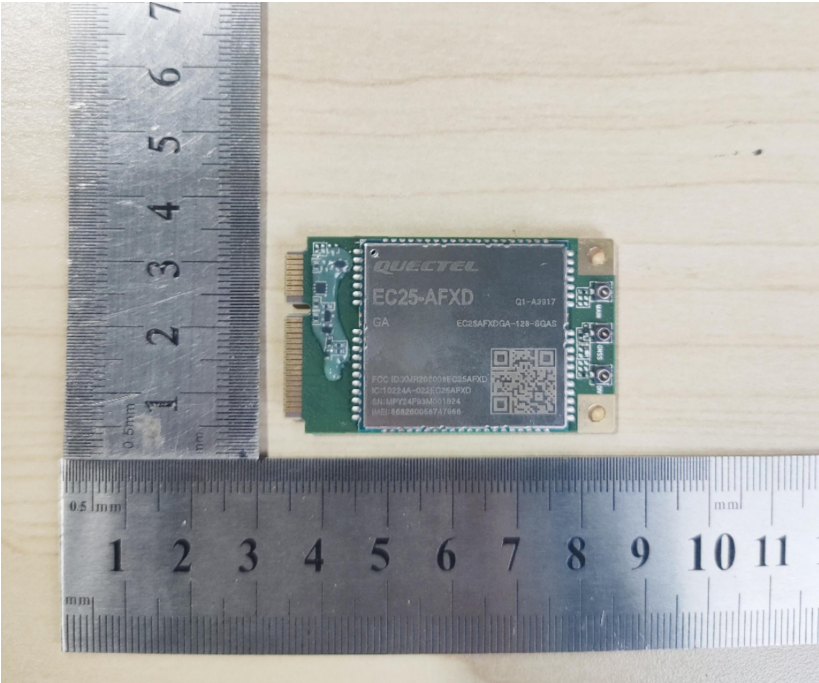
INTERNAL PHOTO OF SAMPLE PCB
