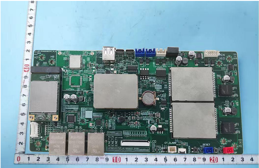
INTERNAL PHOTO OF SAMPLE PCB
