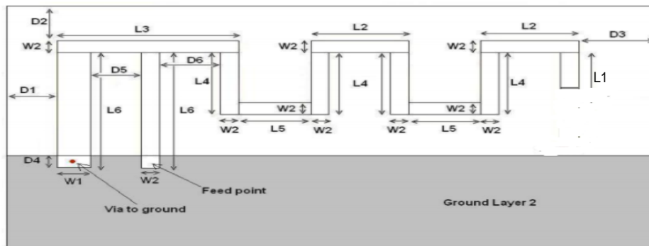
Figure 3: Antenna Dimensions
