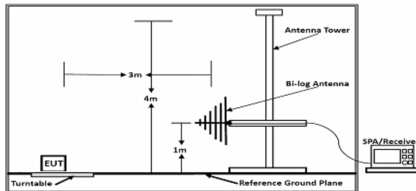
Below 1GHz
