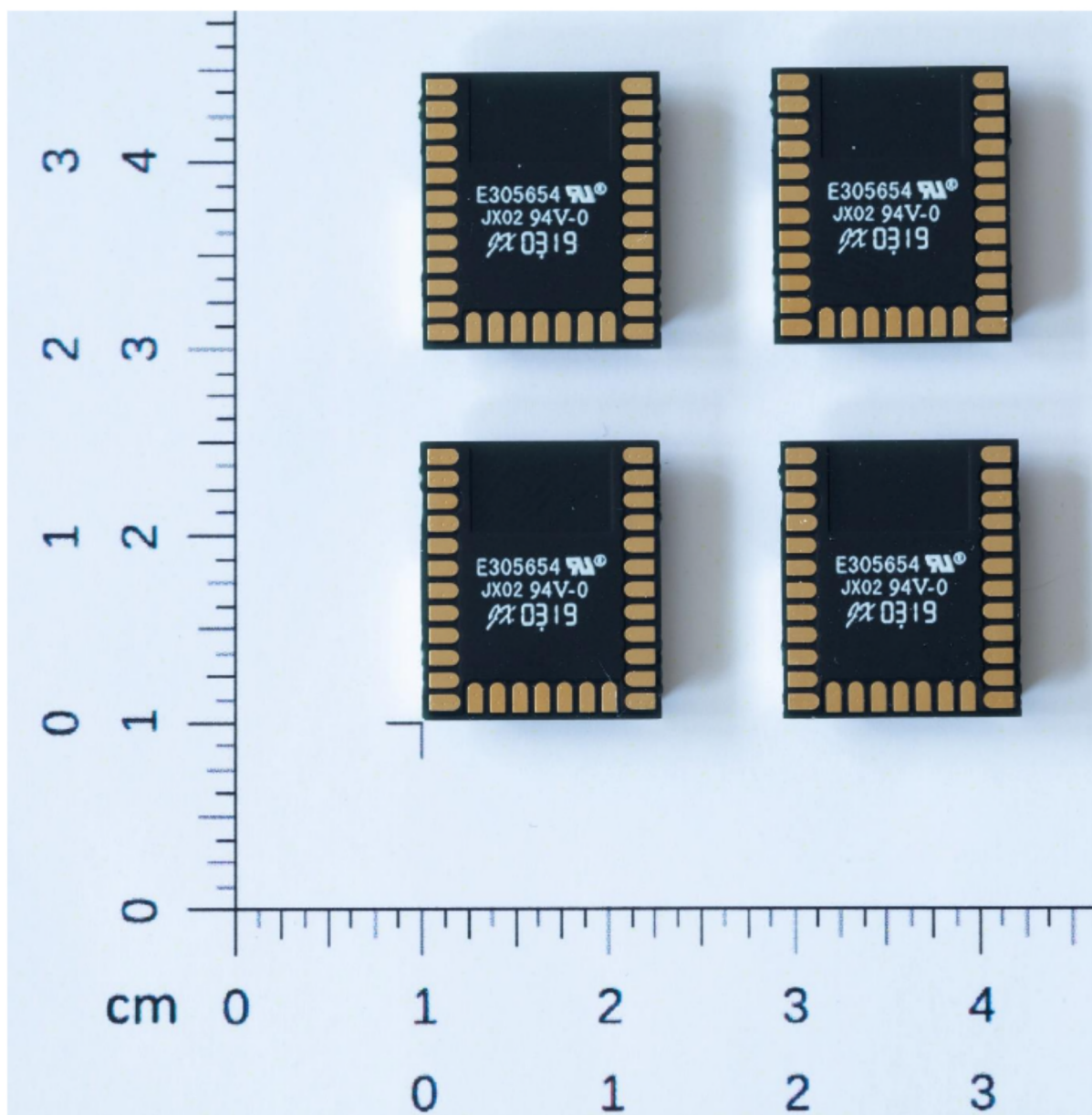
Figure 1: Bottom (rear) view of all variants – Left column: low-power variants / Right column: high-power variants / Top row: BGMx / Bottom row: MGMx
