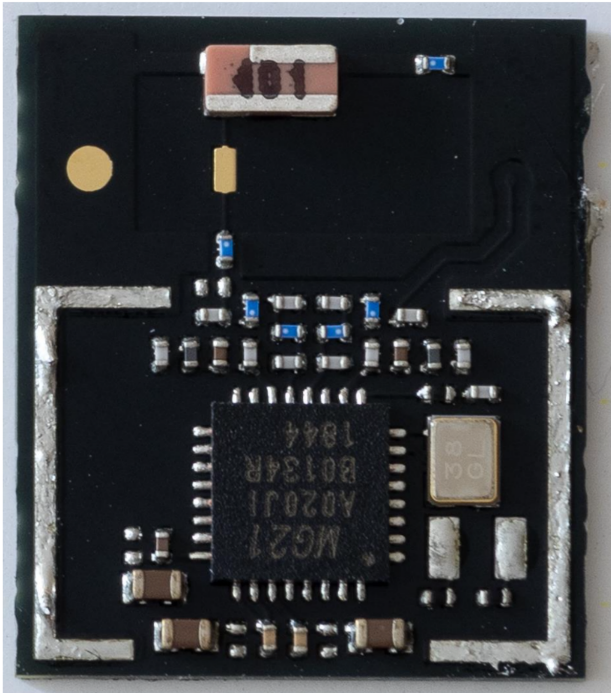
Figure 3: Detail of MGM210P32A – Top (front) internal view
