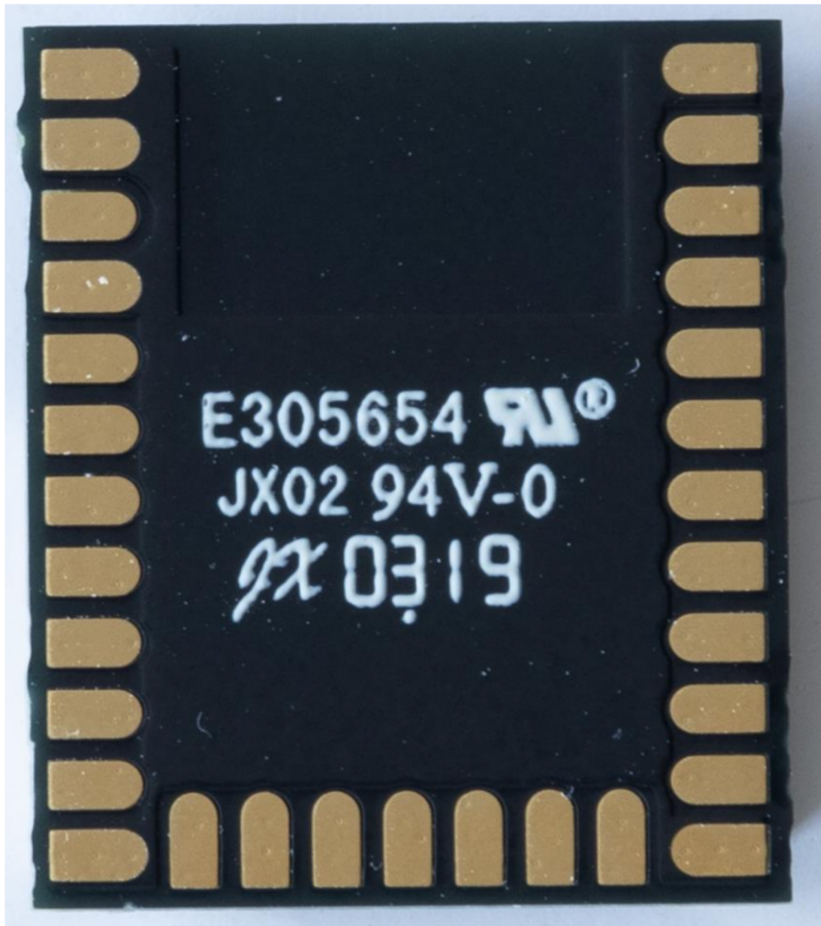
Figure 5: Detail of MGM210P32A – Bottom (rear) external view
