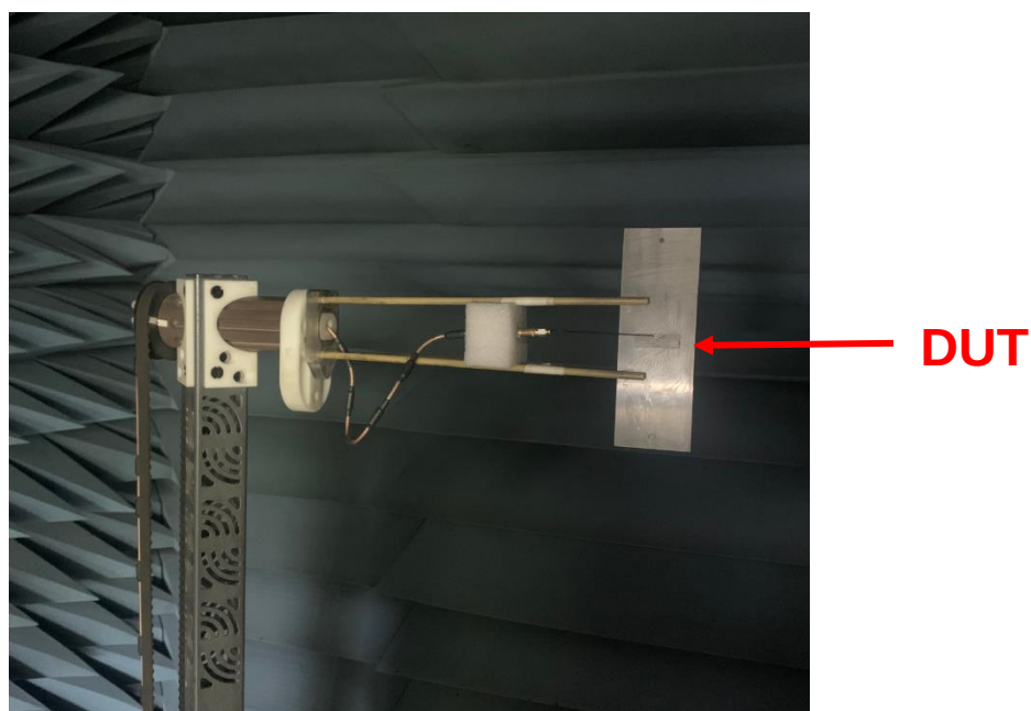
FIGURE4.1.3 ANTENNA LOADED WITH PC/ABS BLOCK OF 1.5 MM THICKNESS WITH OTA CHAMBER
