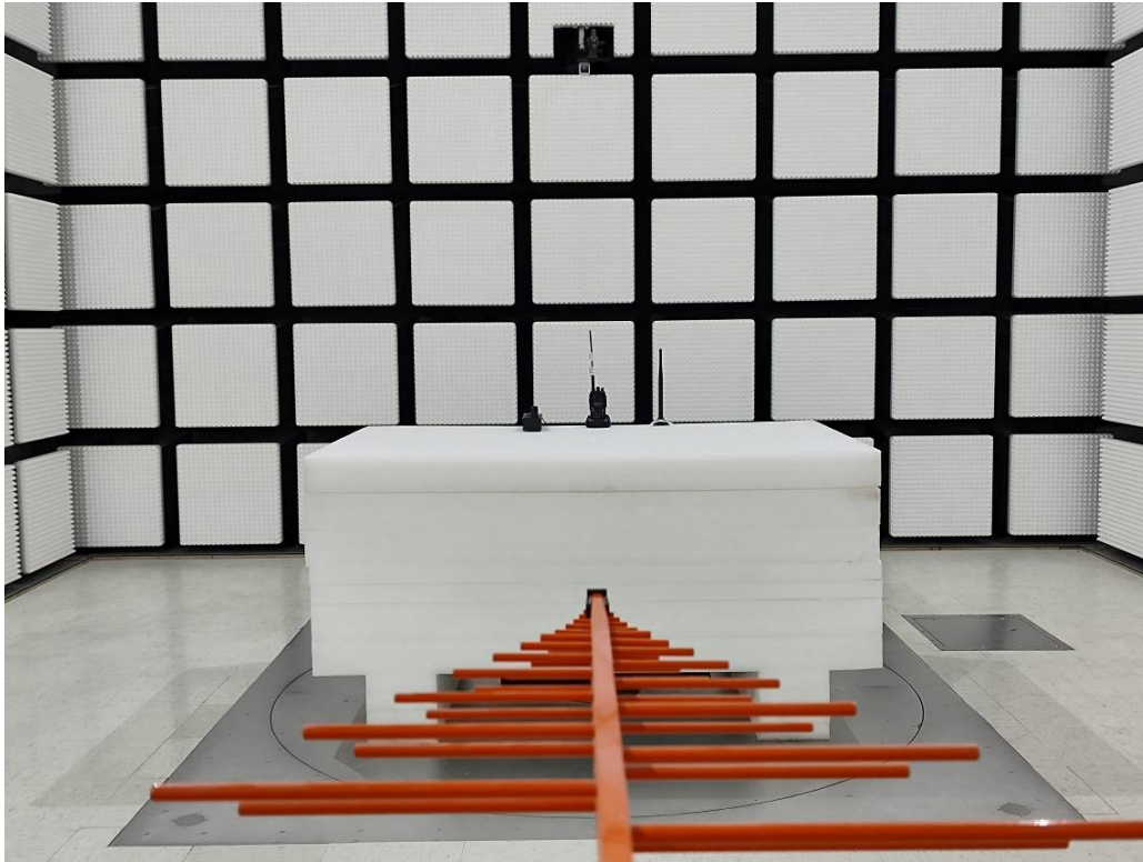
Radiated Emission Below 1GHz Rear View-M2&M3
