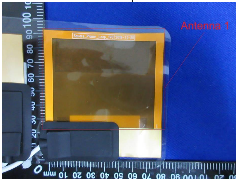
Antenna 1- Loop Antenna
