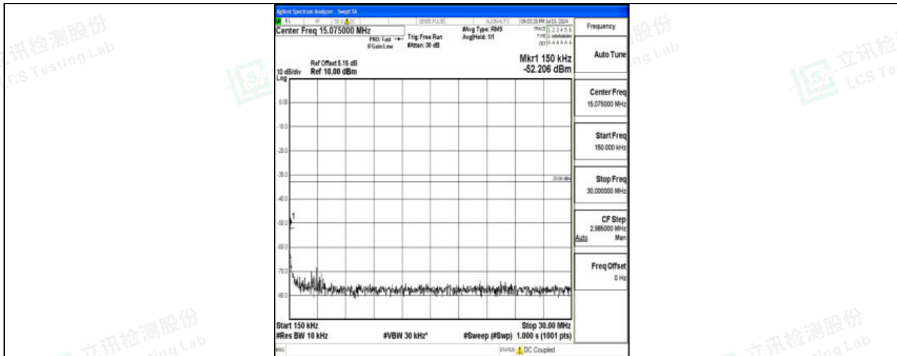
Band66_5MHz_QPSK_131997_1RB#0_0.15~30_0.15~30
