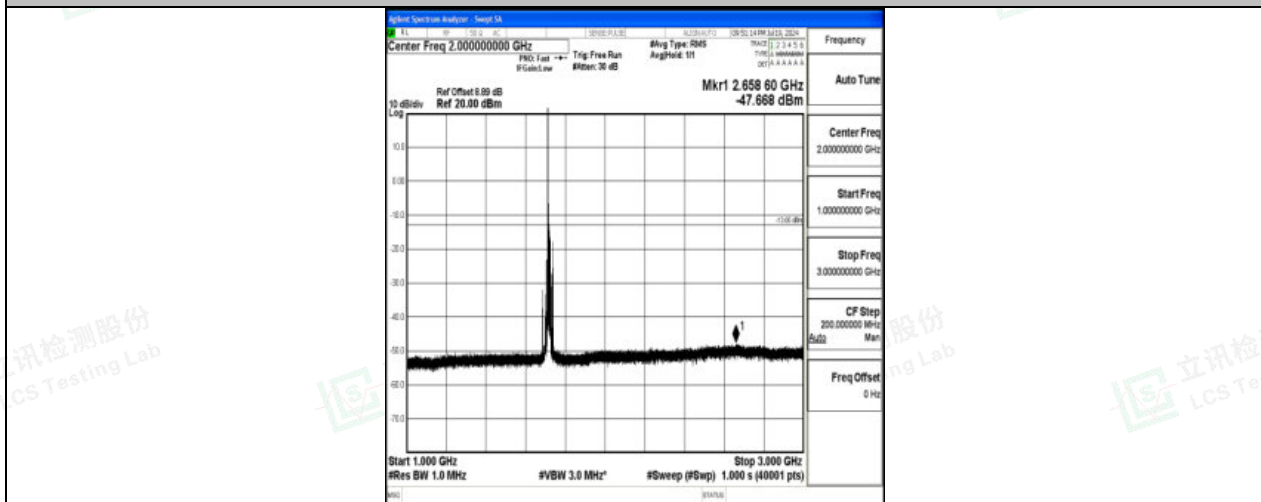
Band66_15MHz_16QAM_132047_1RB#0_1000~3000_1000~3000
