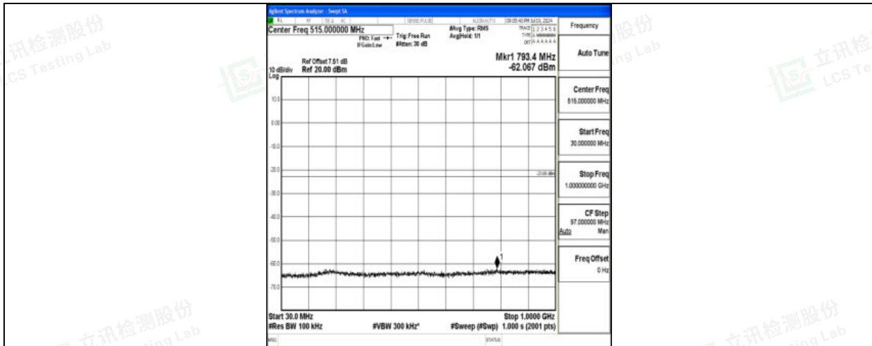
Band66_5MHz_QPSK_132647_1RB#0_30~1000_30~1000
