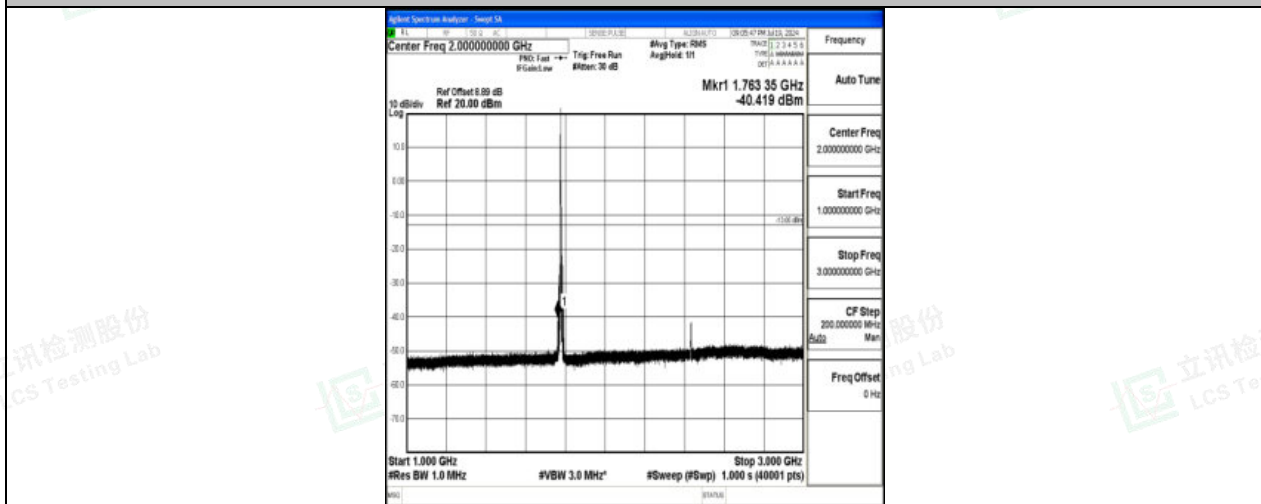
Band66_5MHz_QPSK_132647_1RB#0_1000~3000_1000~3000
