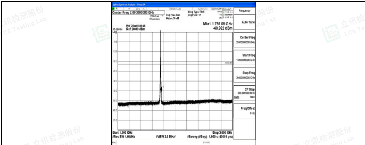
Band66_5MHz_QPSK_132322_1RB#0_1000~3000_1000~3000
