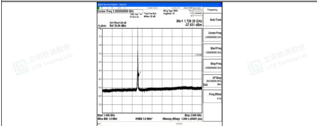
Band66_5MHz_QPSK_131997_1RB#0_1000~3000_1000~3000
