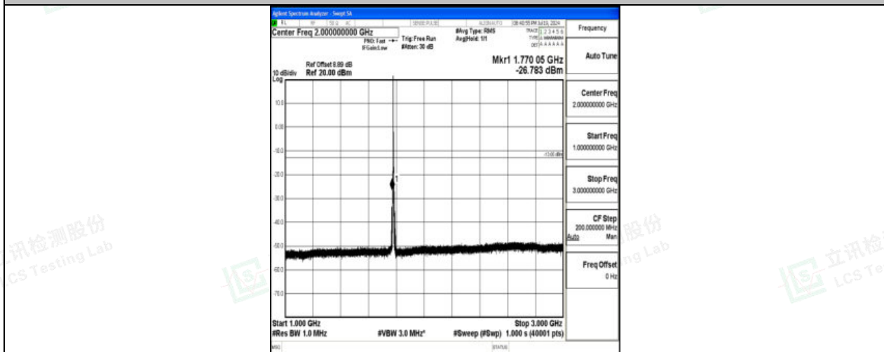
Band66_3MHz_QPSK_132657_1RB#0_1000~3000_1000~3000
