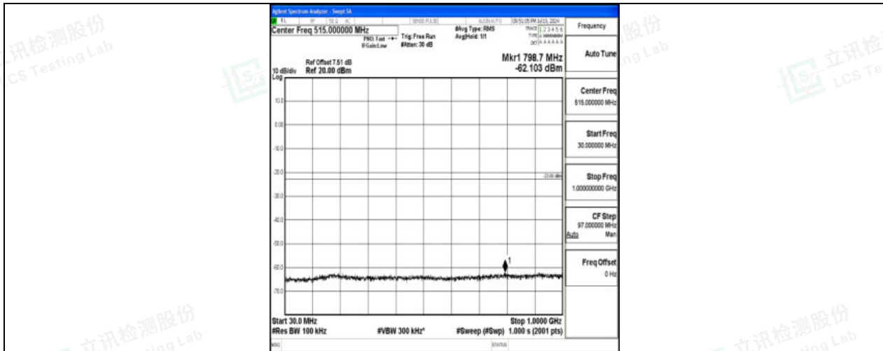
Band66_15MHz_16QAM_132047_1RB#0_30~1000_30~1000
