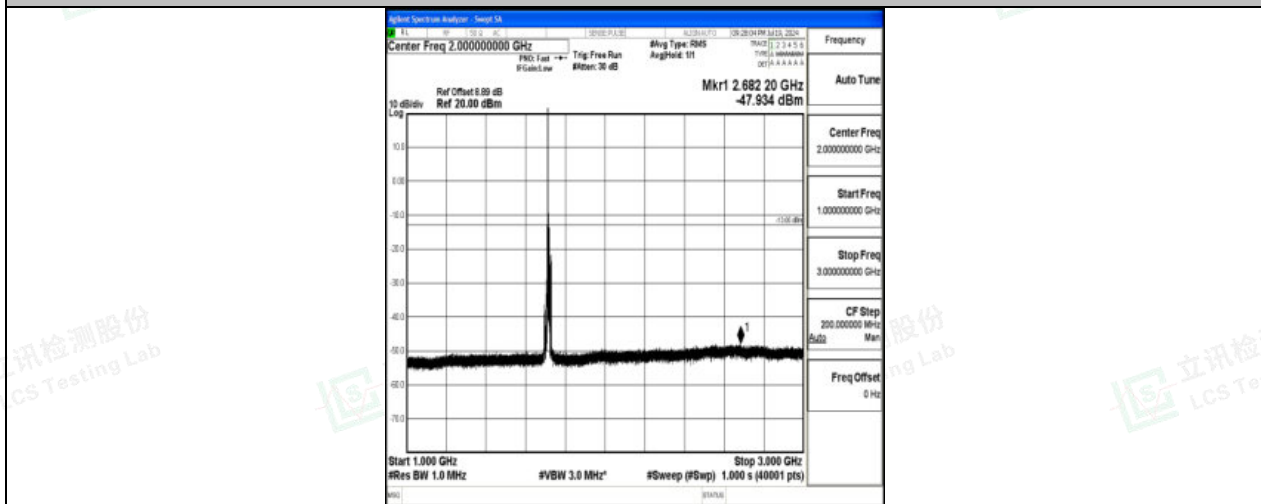
Band66_10MHz_16QAM_132022_1RB#0_1000~3000_1000~3000
