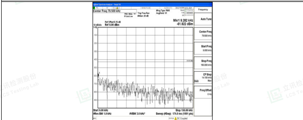
Band66_10MHz_16QAM_132022_1RB#0_0.009~0.15_0.009~0.15
