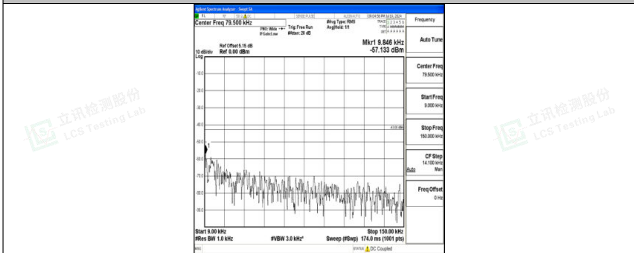
Band66_5MHz_16QAM_132322_1RB#0_0.009~0.15_0.009~0.15
