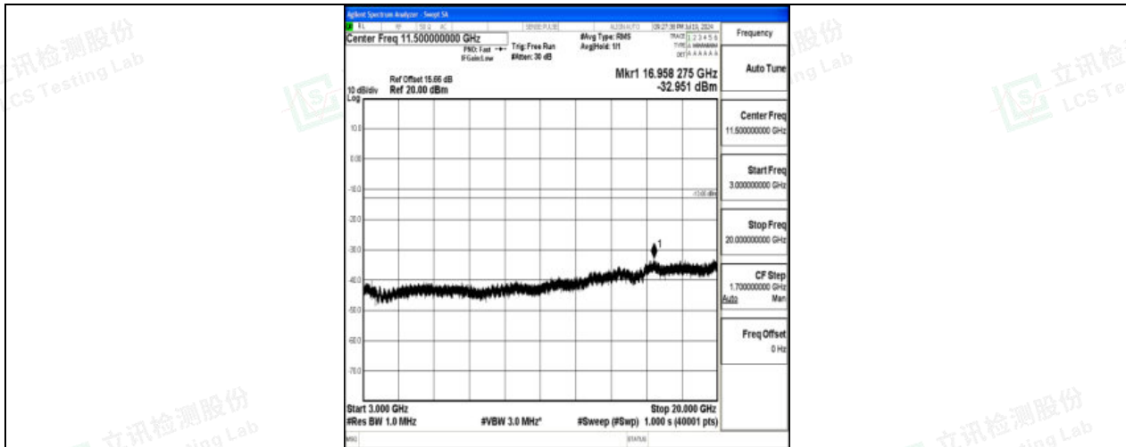
Band66_10MHz_QPSK_132022_1RB#0_3000~20000_3000~20000
