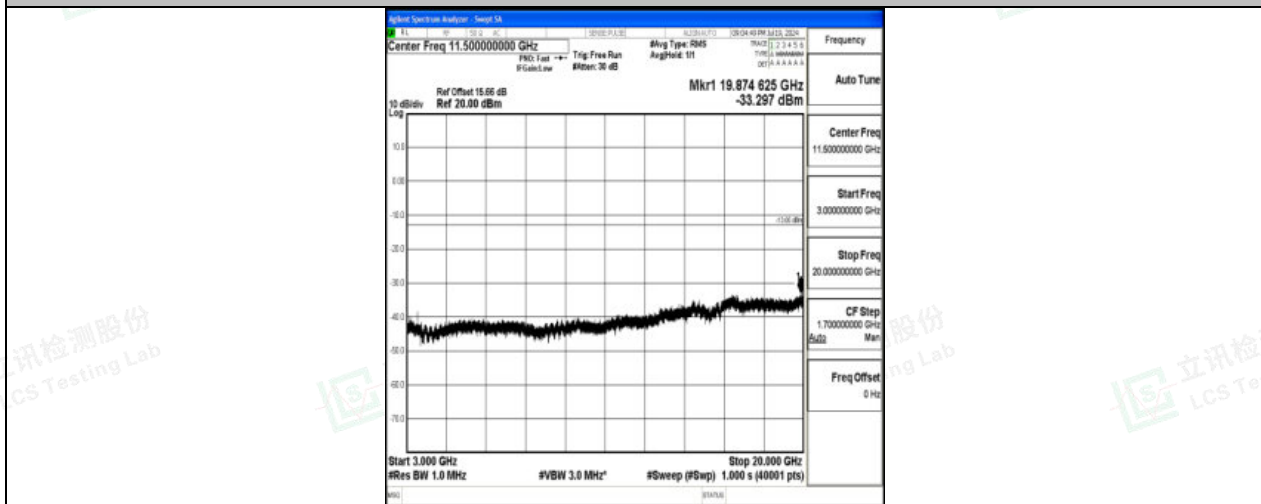
Band66_5MHz_QPSK_132322_1RB#0_3000~20000_3000~20000
