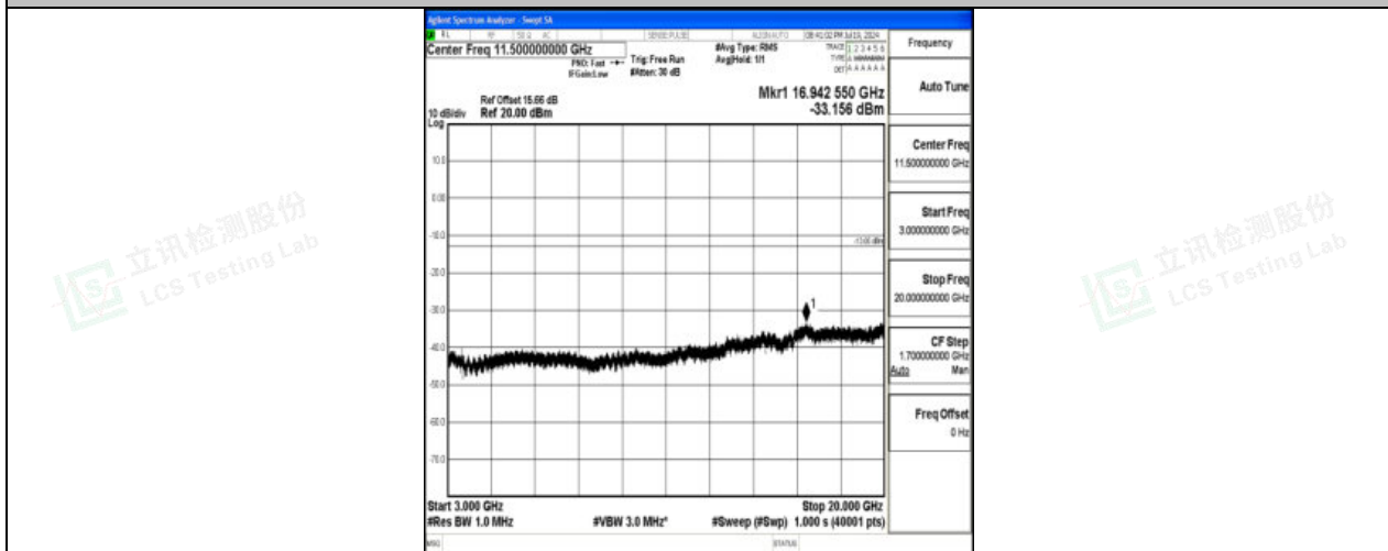
Band66_3MHz_QPSK_132657_1RB#0_3000~20000_3000~20000
