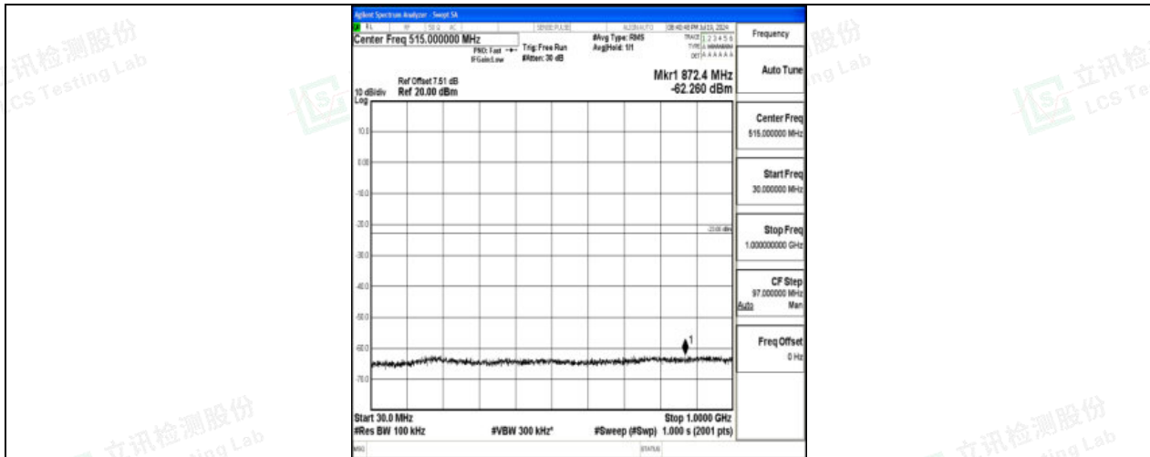
Band66_3MHz_QPSK_132657_1RB#0_30~1000_30~1000
