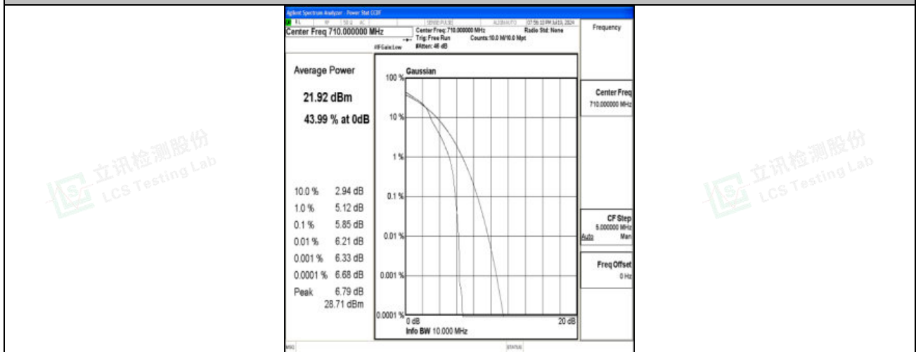
Band17-10MHz-16QAM-23790-1RB#0-PASS
