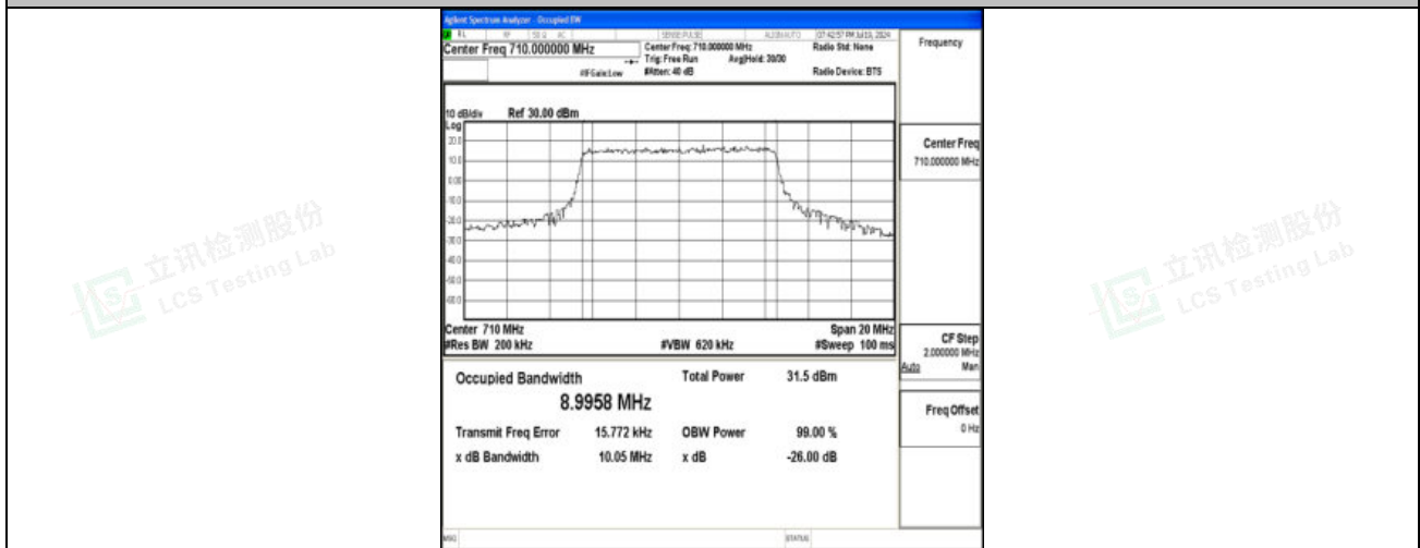
Band17-10MHz-QPSK-23790-50RB#0-PASS
