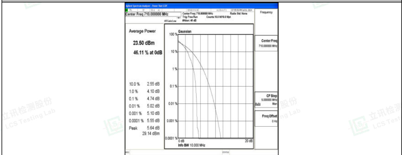
Band17-10MHz-QPSK-23790-1RB#0-PASS
