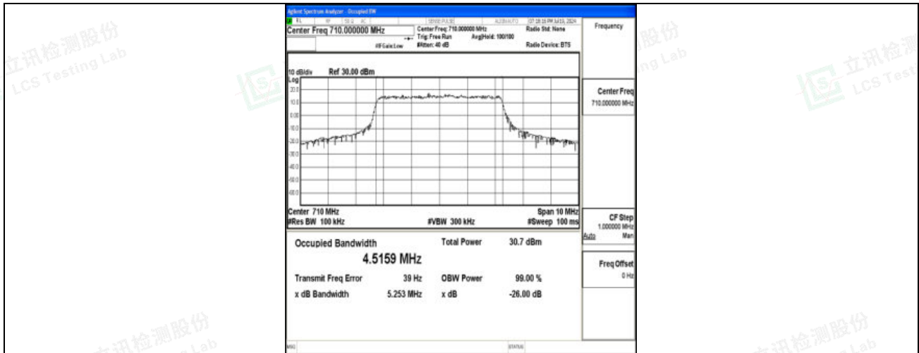
Band17-5MHz-16QAM-23790-25RB#0-PASS
