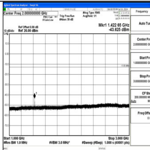
Band12_5MHz_QPSK_23155_1RB#0_1000~3000_1000~3000
