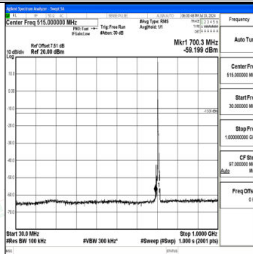
Band12_5MHz_QPSK_23155_1RB#0_30~1000_30~1000
