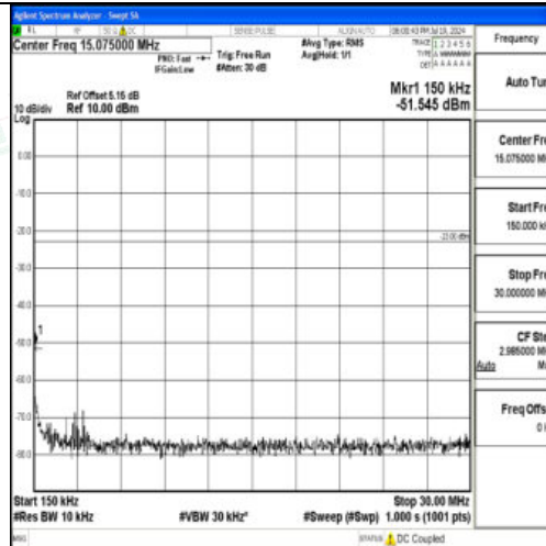
Band12_5MHz_QPSK_23155_1RB#0_0.15~30_0.15~30
