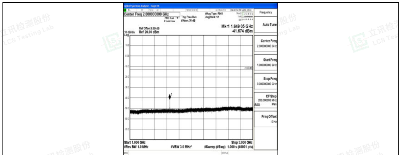
Band5_10MHz_QPSK_20450_1RB#0_1000~3000_1000~3000
