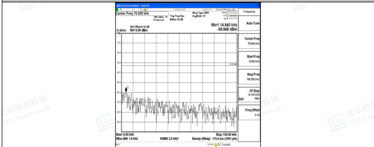
Band5_10MHz_16QAM_20600_1RB#0_0.009~0.15_0.009~0.15
