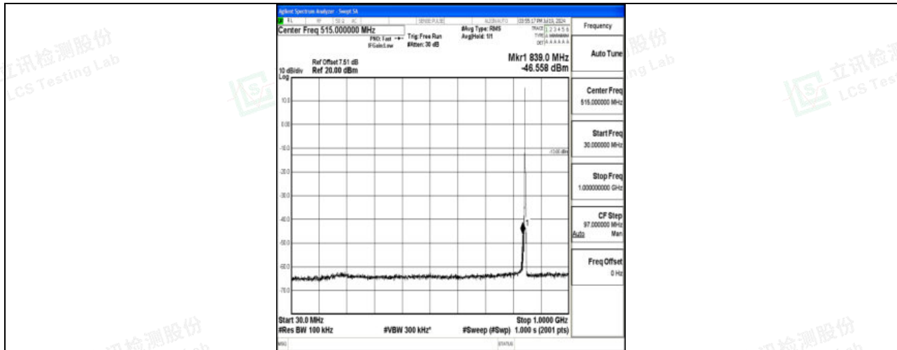
Band5_3MHz_16QAM_20635_1RB#0_30~1000_30~1000
