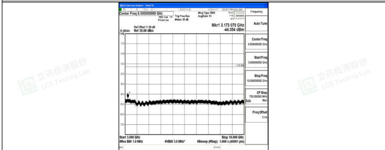
Band5_1.4MHz_16QAM_20643_1RB#0_3000~10000_3000~10000
