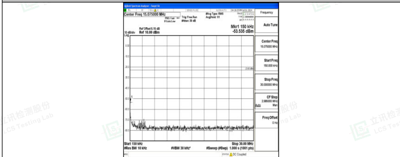
Band5_5MHz_16QAM_20525_1RB#0_0.15~30_0.15~30
