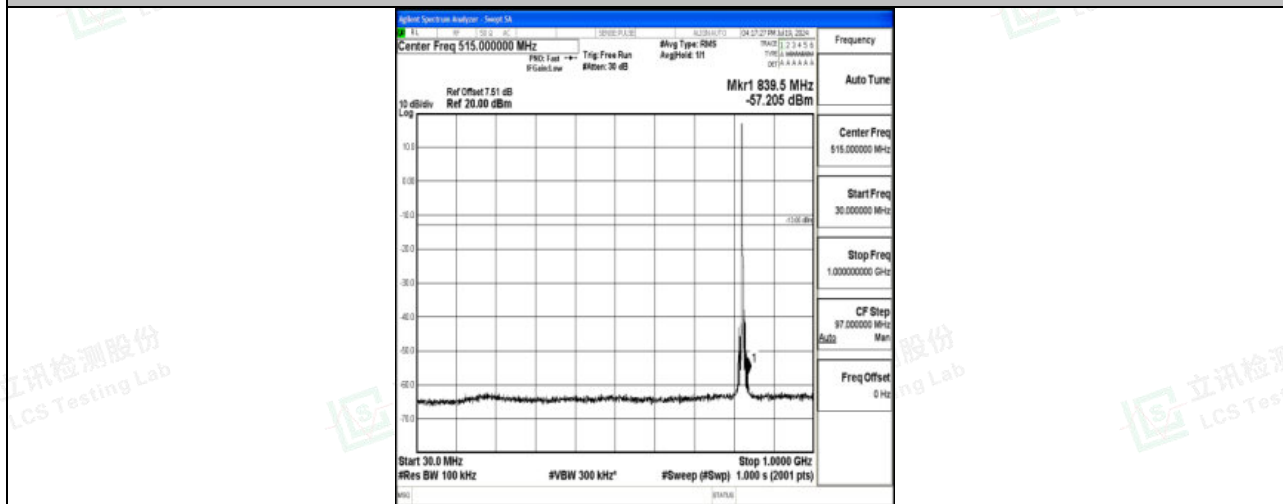
Band5_5MHz_16QAM_20425_1RB#0_30~1000_30~1000
