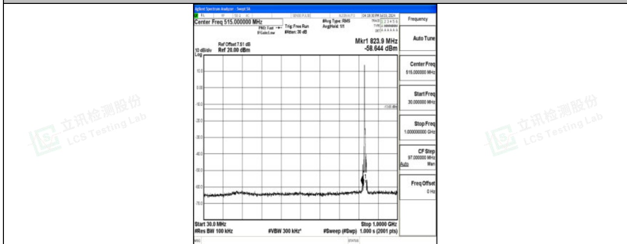
Band5_5MHz_16QAM_20525_1RB#0_30~1000_30~1000
