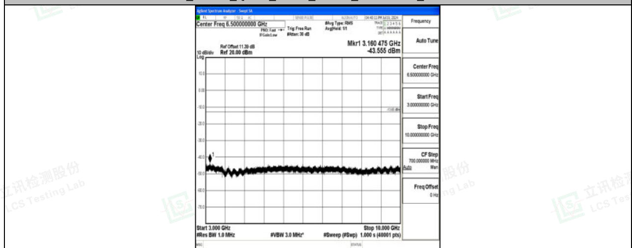
Band5_10MHz_QPSK_20450_1RB#0_3000~10000_3000~10000
