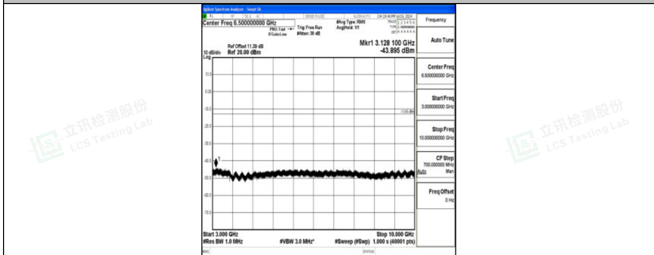
Band5_5MHz_16QAM_20625_1RB#0_3000~10000_3000~10000
