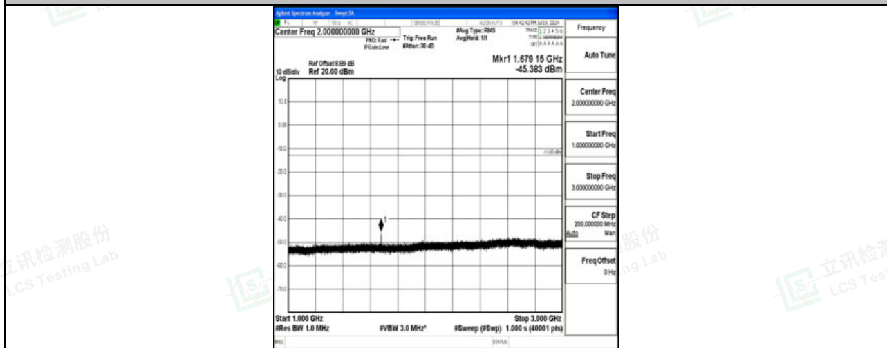
Band5_10MHz_16QAM_20600_1RB#0_1000~3000_1000~3000
