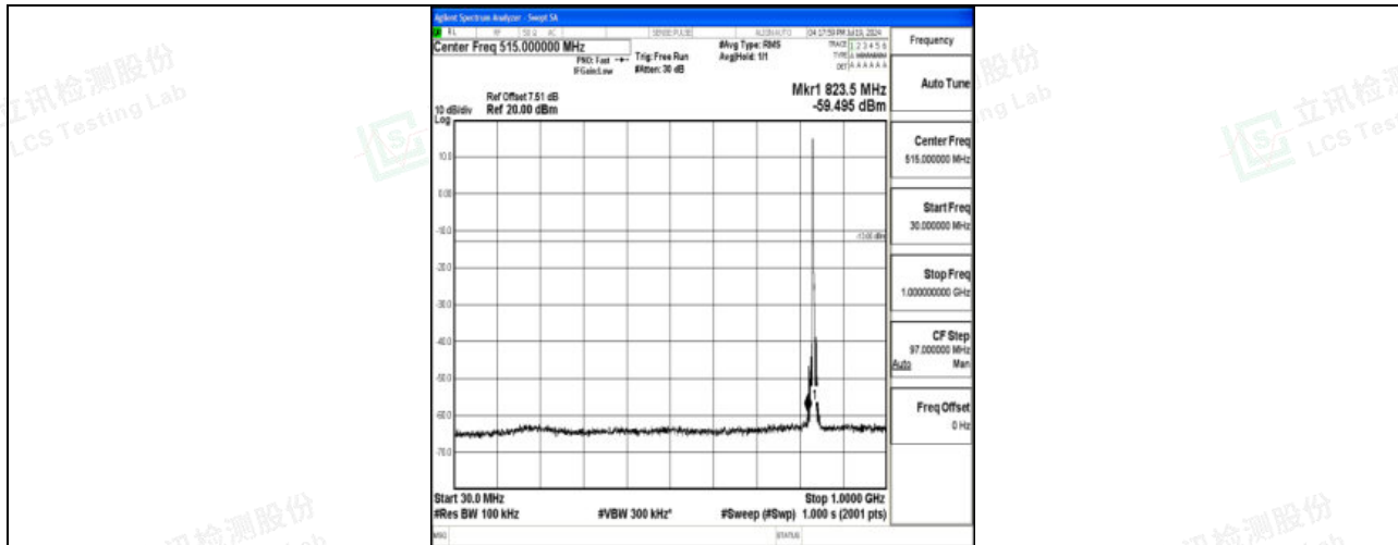
Band5_5MHz_QPSK_20525_1RB#0_30~1000_30~1000
