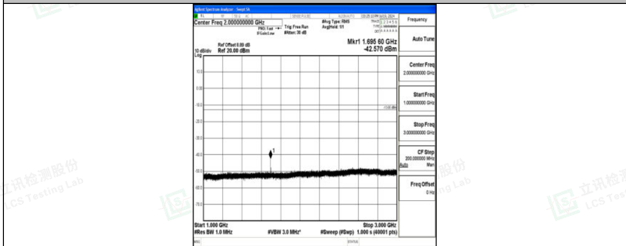
Band5_1.4MHz_16QAM_20643_1RB#0_1000~3000_1000~3000
