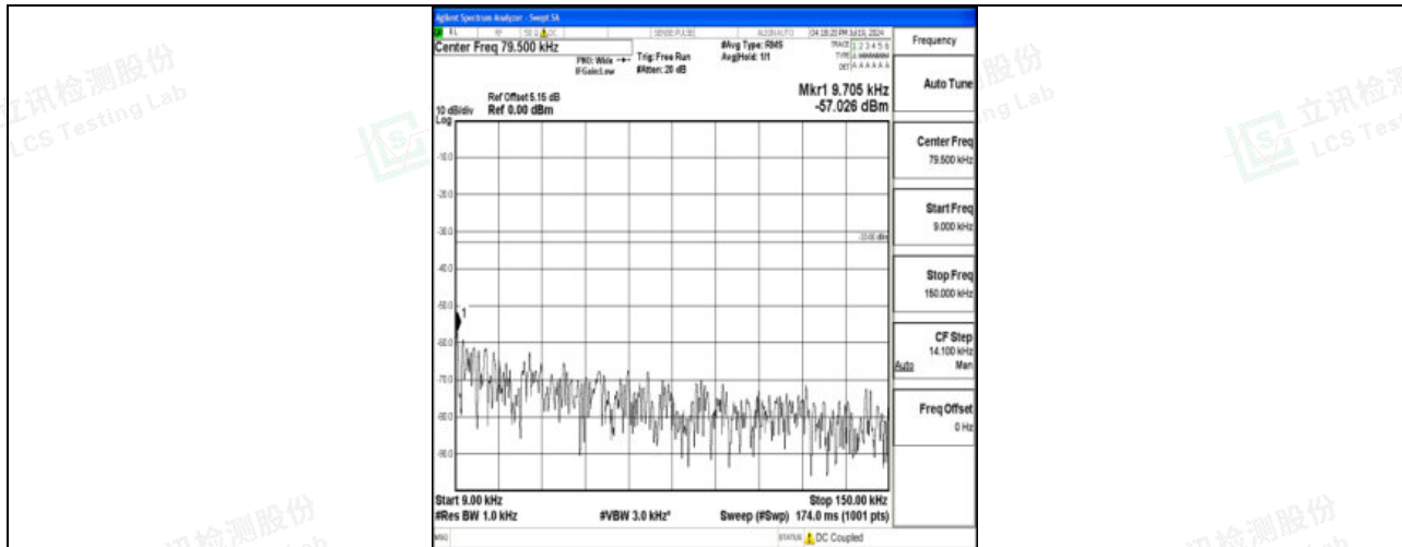
Band5_5MHz_16QAM_20525_1RB#0_0.009~0.15_0.009~0.15
