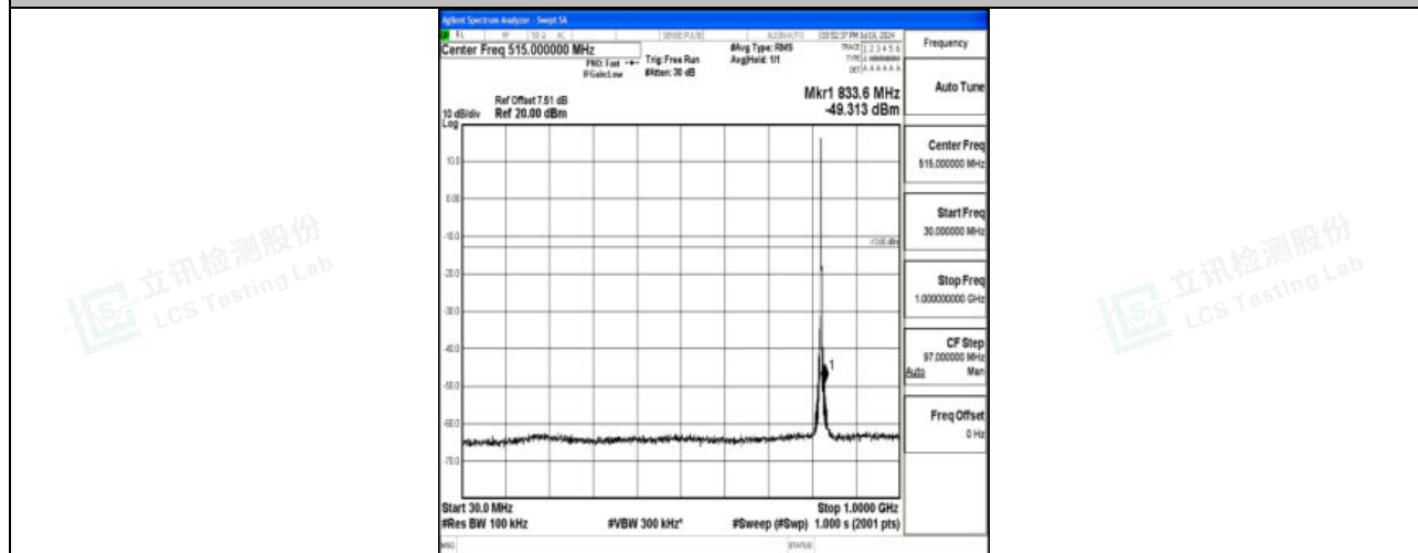
Band5_3MHz_QPSK_20415_1RB#0_30~1000_30~1000
