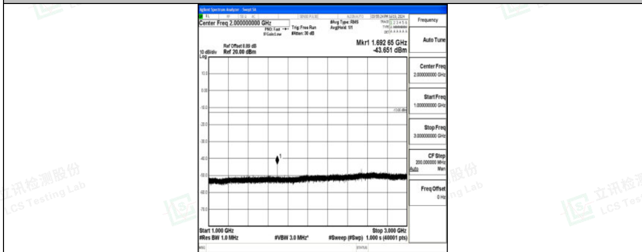
Band5_3MHz_16QAM_20635_1RB#0_1000~3000_1000~3000
