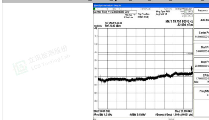
Band4_20MHz_QPSK_20300_1RB#0_3000~20000_3000~20000
