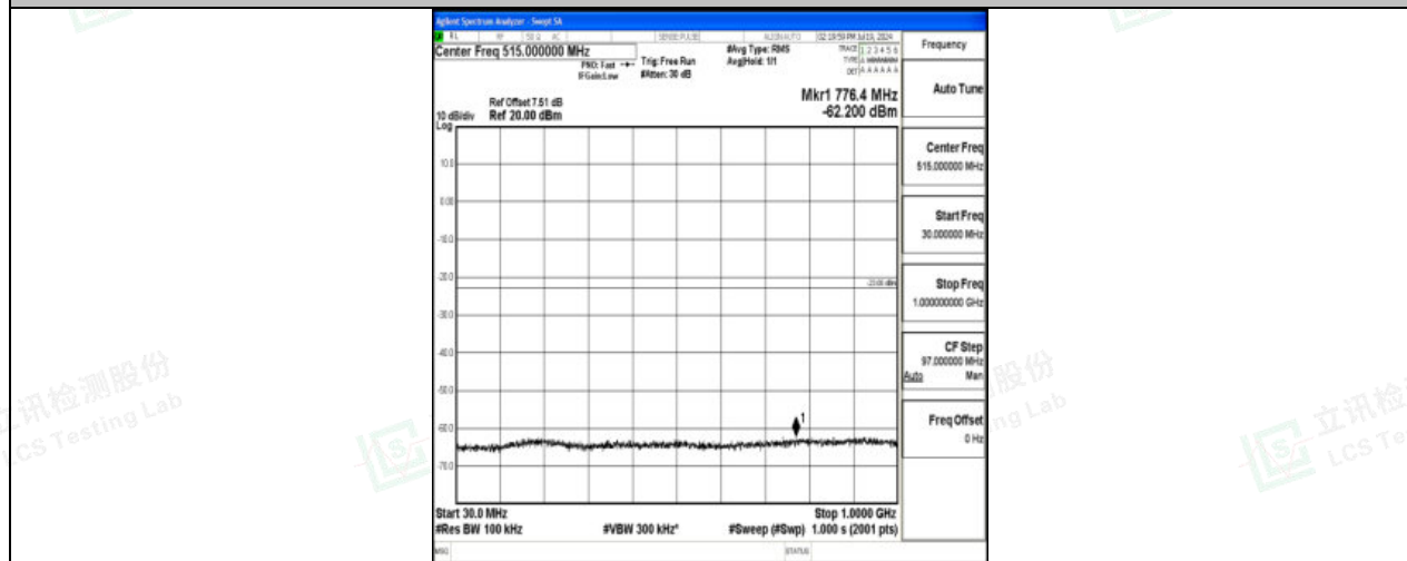
Band4_10MHz_QPSK_20000_1RB#0_30~1000_30~1000
