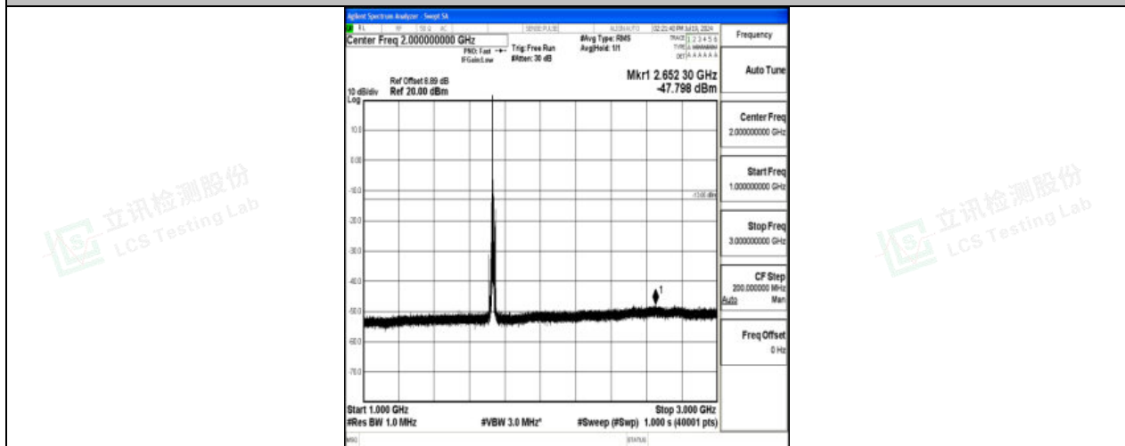
Band4_10MHz_16QAM_20175_1RB#0_1000~3000_1000~3000
