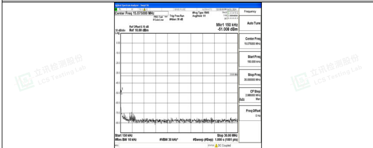
Band4_5MHz_QPSK_20375_1RB#0_0.15~30_0.15~30
