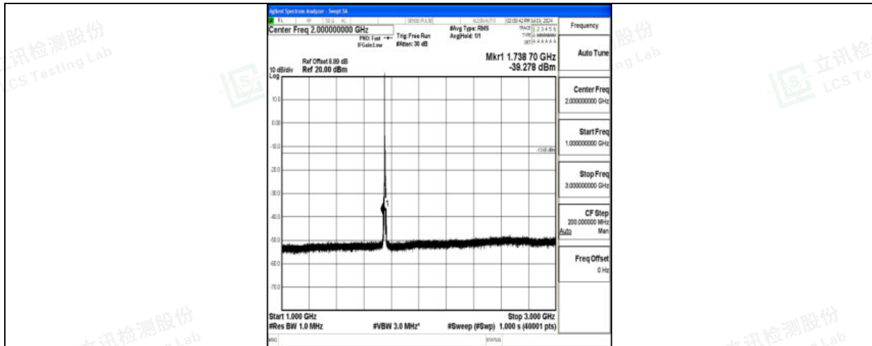
Band4_5MHz_16QAM_20375_1RB#0_1000~3000_1000~3000
