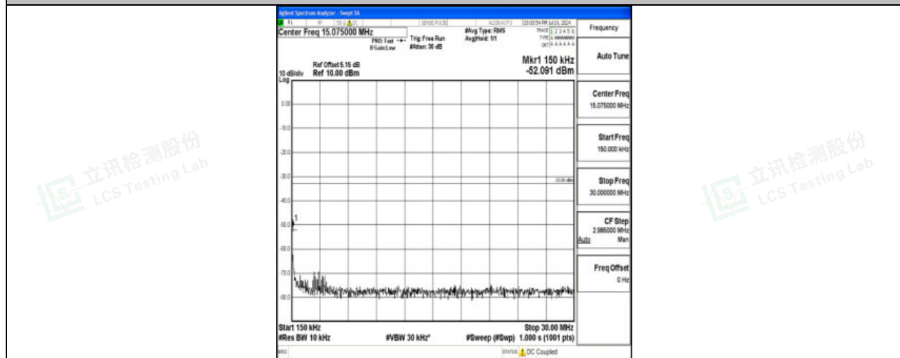
Band4_20MHz_QPSK_20300_1RB#0_0.15~30_0.15~30
