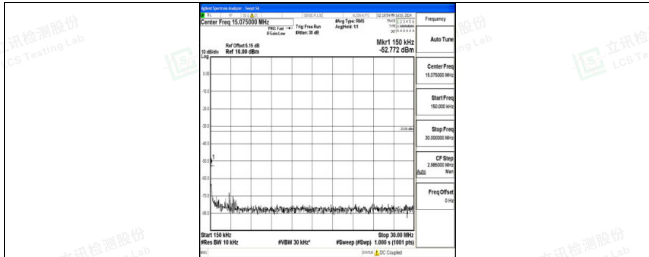
Band4_10MHz_QPSK_20000_1RB#0_0.15~30_0.15~30
