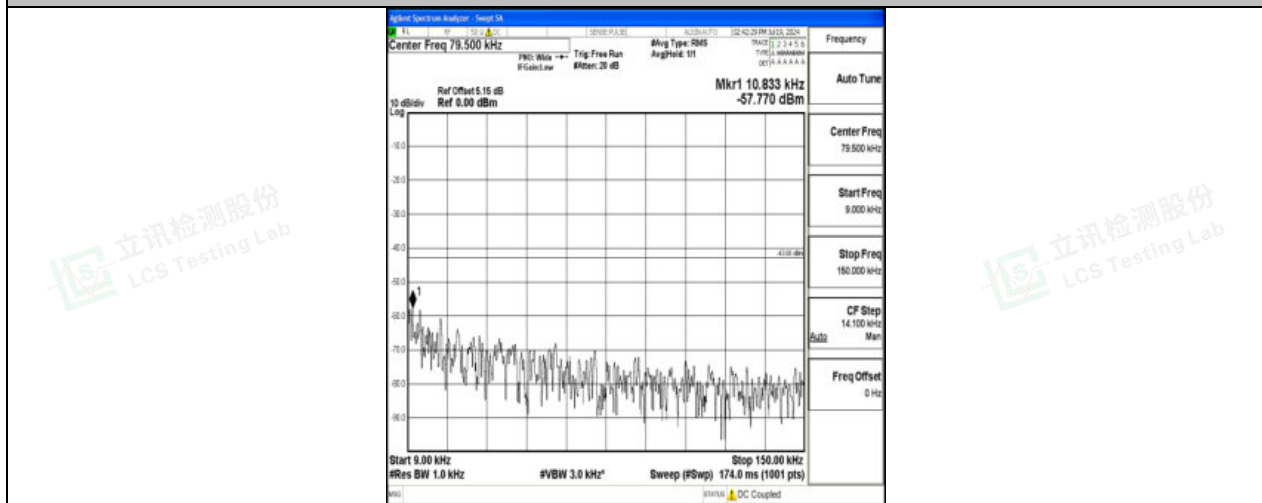
Band4_15MHz_16QAM_20175_1RB#0_0.009~0.15_0.009~0.15
