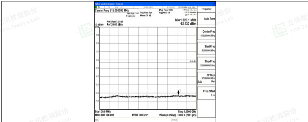
Band4_5MHz_16QAM_19975_1RB#0_30~1000_30~1000
