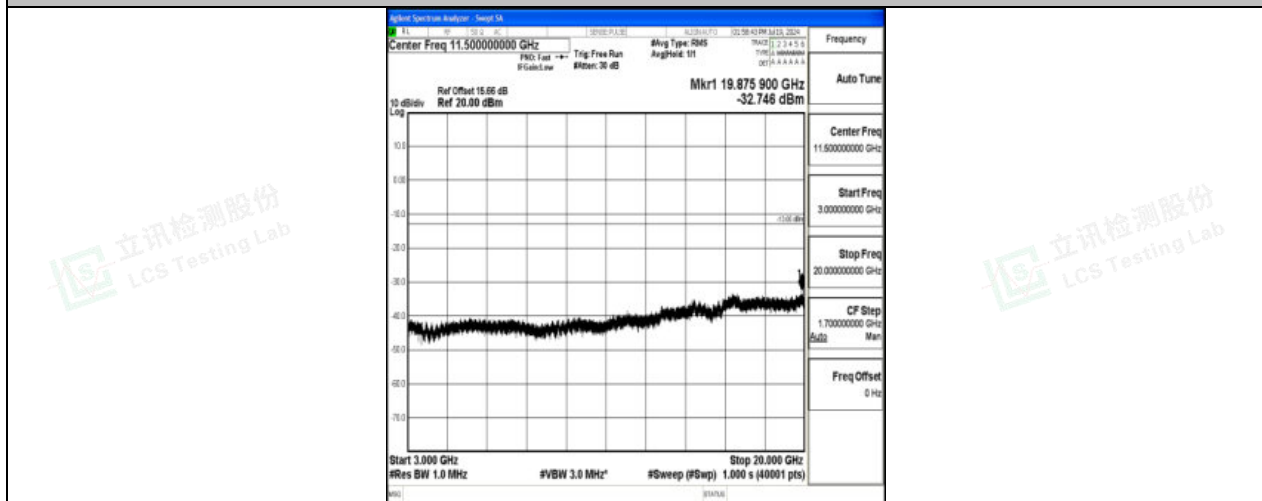
Band4_5MHz_16QAM_19975_1RB#0_3000~20000_3000~20000
