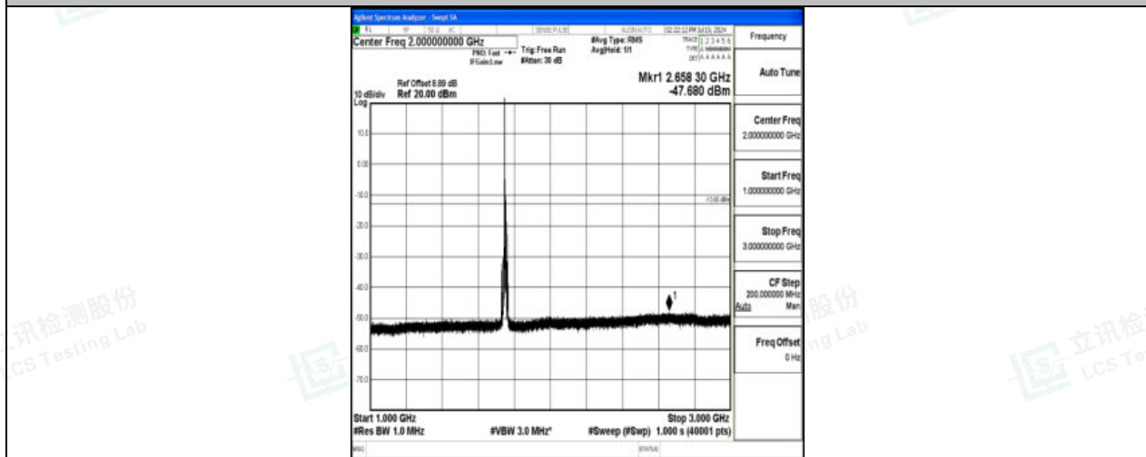
Band4_10MHz_QPSK_20350_1RB#0_1000~3000_1000~3000
