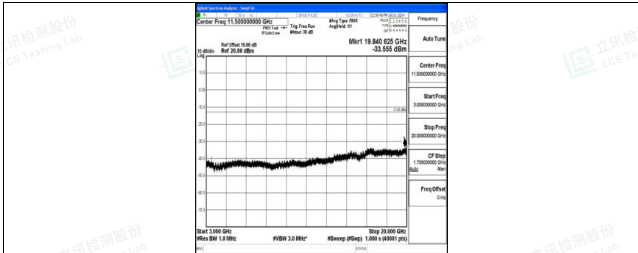
Band4_5MHz_16QAM_20175_1RB#0_3000~20000_3000~20000
