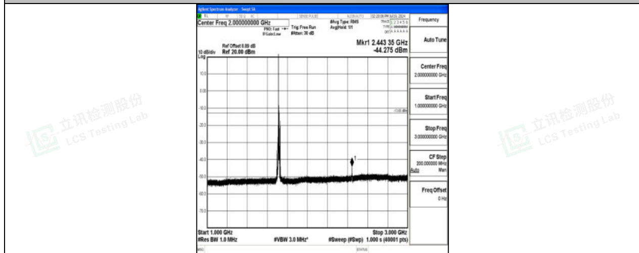
Band4_10MHz_QPSK_20000_1RB#0_1000~3000_1000~3000
