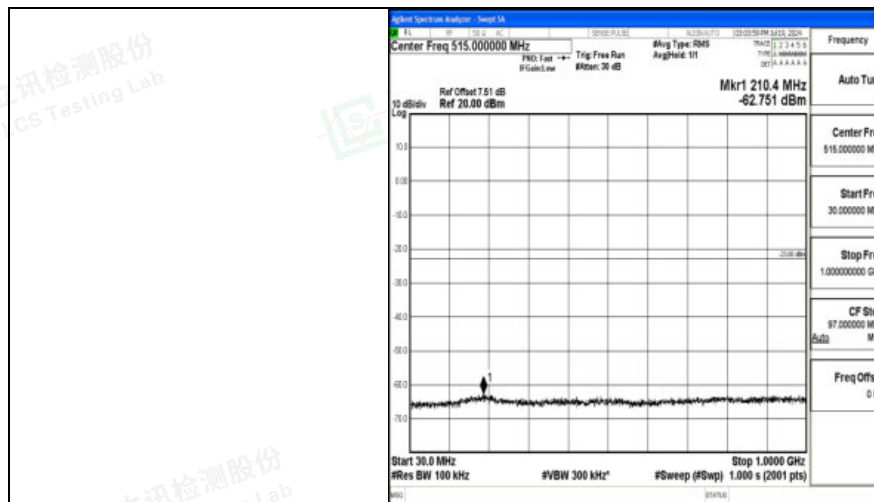
Band4_20MHz_QPSK_20300_1RB#0_30~1000_30~1000
