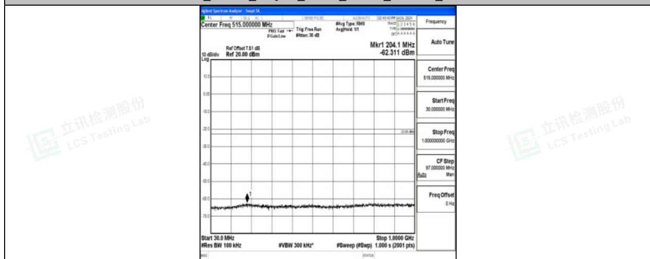
Band4_15MHz_16QAM_20325_1RB#0_30~1000_30~1000
