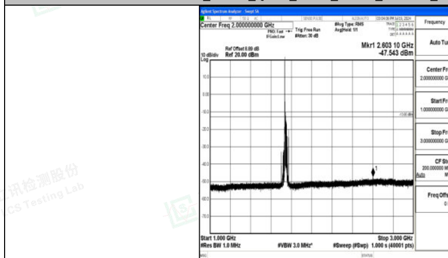
Band4_20MHz_QPSK_20300_1RB#0_1000~3000_1000~3000
