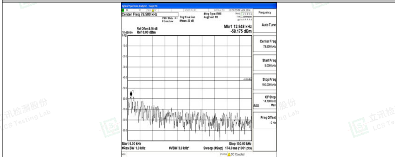
Band4_5MHz_QPSK_20375_1RB#0_0.009~0.15_0.009~0.15
