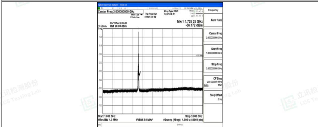
Band4_5MHz_16QAM_19975_1RB#0_1000~3000_1000~3000
