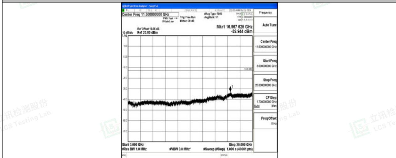
Band4_5MHz_16QAM_20375_1RB#0_3000~20000_3000~20000
