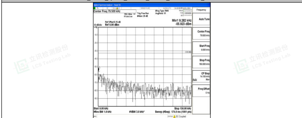
Band71_5MHz_16QAM_133147_1RB#0_0.009~0.15_0.009~0.15
