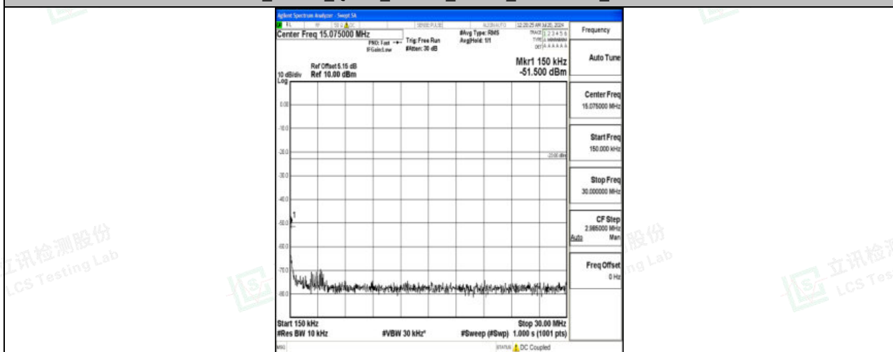
Band71_15MHz_QPSK_133197_1RB#0_0.15~30_0.15~30
