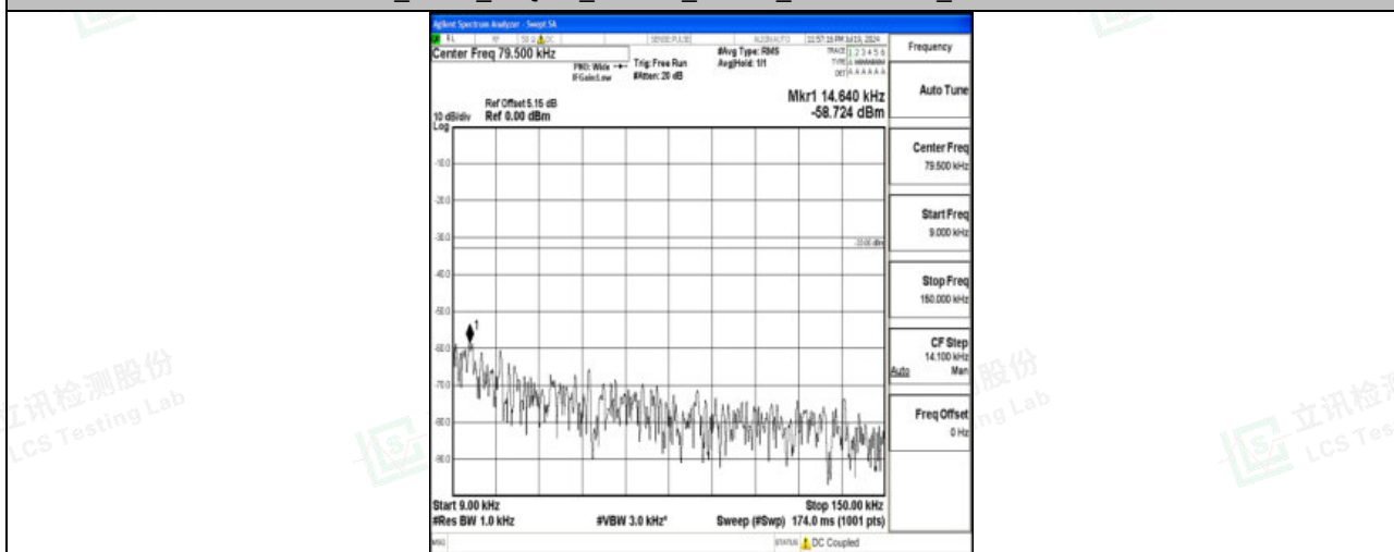
Band71_10MHz_16QAM_133422_1RB#0_0.009~0.15_0.009~0.15
