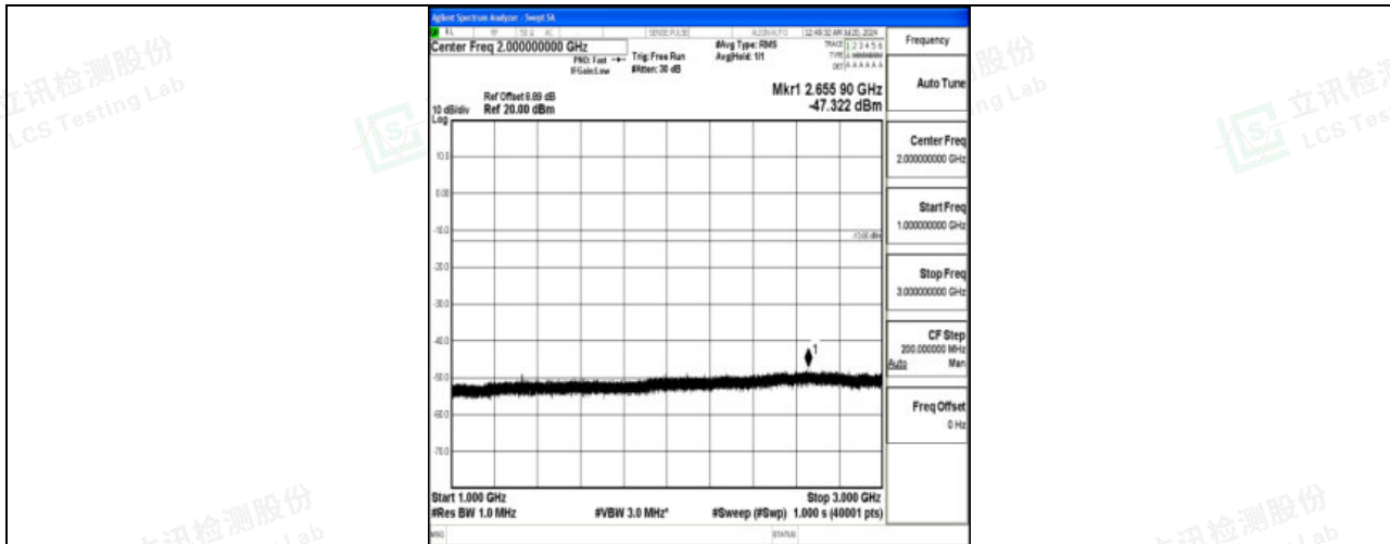
Band71_20MHz_QPSK_133222_1RB#0_1000~3000_1000~3000
