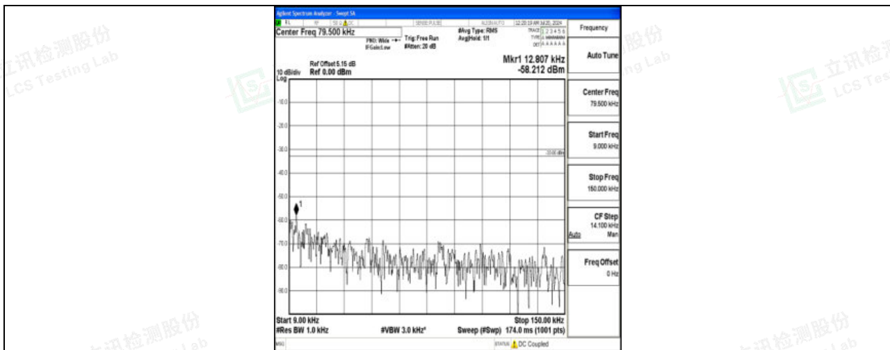
Band71_15MHz_QPSK_133197_1RB#0_0.009~0.15_0.009~0.15
