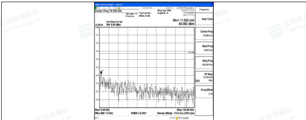
Band71_10MHz_QPSK_133422_1RB#0_0.009~0.15_0.009~0.15
