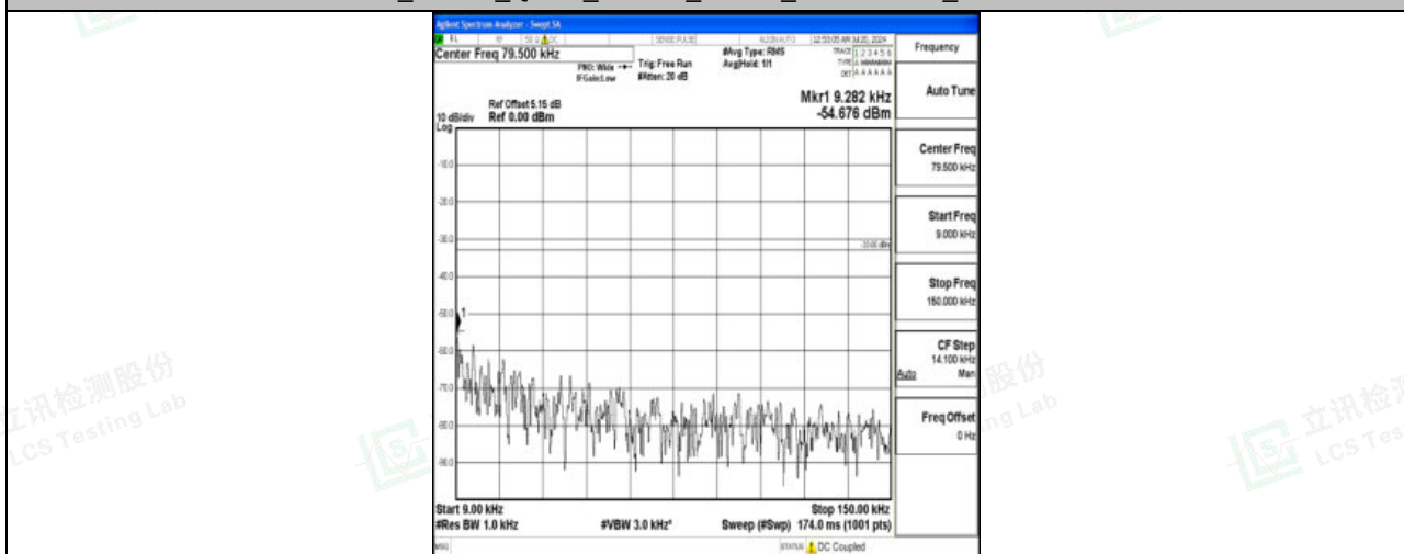
Band71_20MHz_16QAM_133322_1RB#0_0.009~0.15_0.009~0.15
