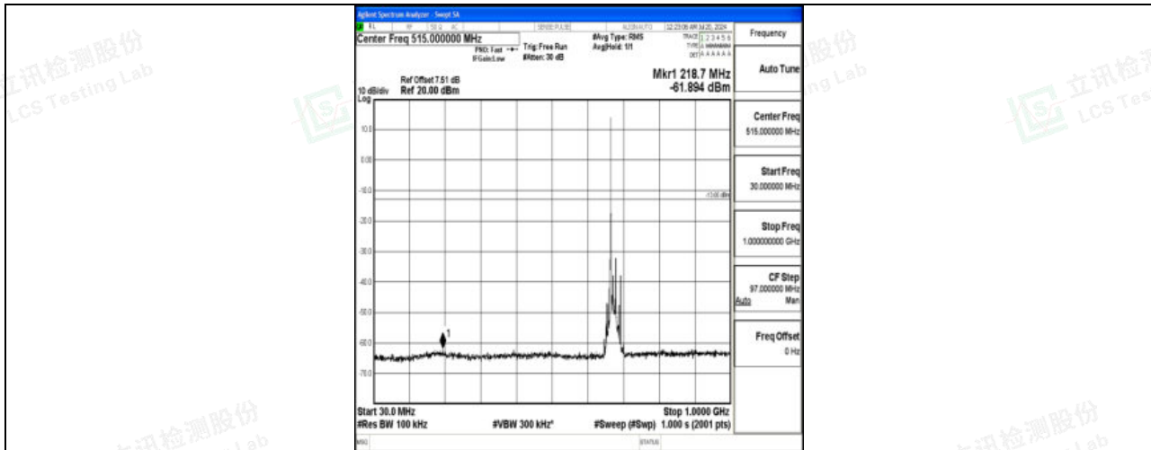
Band71_15MHz_QPSK_133297_1RB#0_30~1000_30~1000
