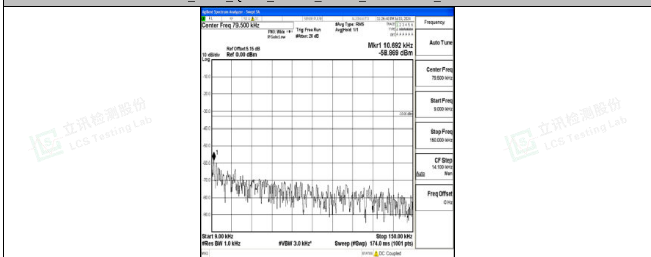
Band71_5MHz_16QAM_133447_1RB#0_0.009~0.15_0.009~0.15
