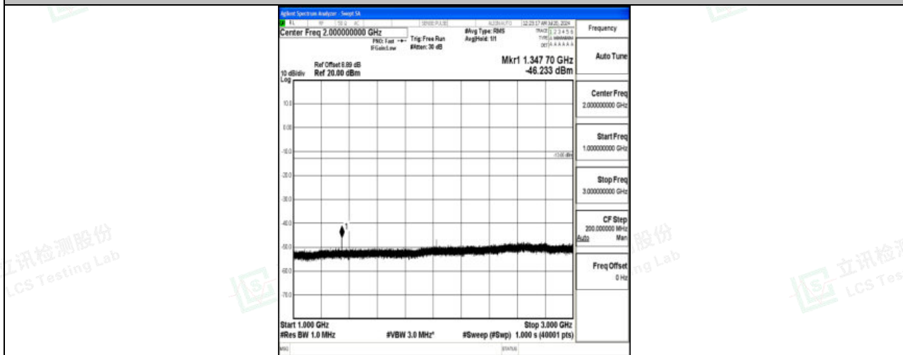
Band71_15MHz_QPSK_133297_1RB#0_1000~3000_1000~3000
