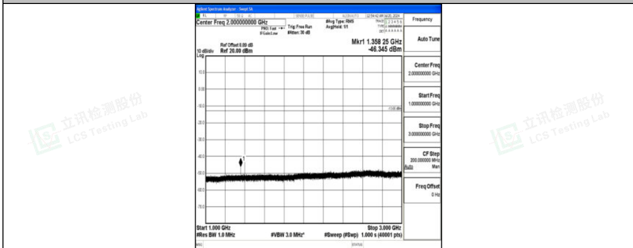
Band71_20MHz_QPSK_133372_1RB#0_1000~3000_1000~3000
