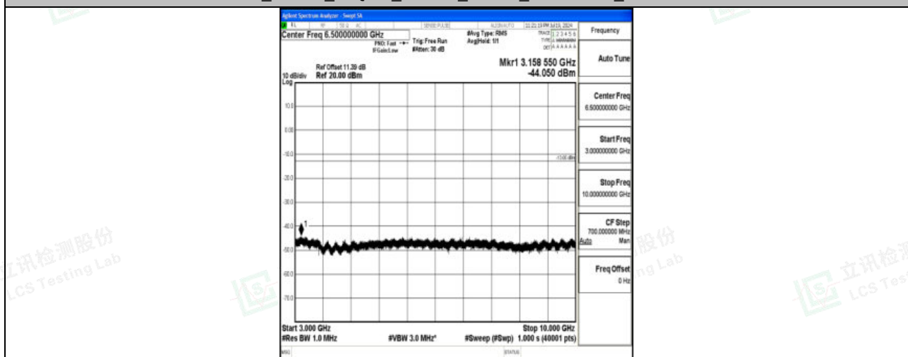
Band71_5MHz_QPSK_133147_1RB#0_3000~10000_3000~10000
