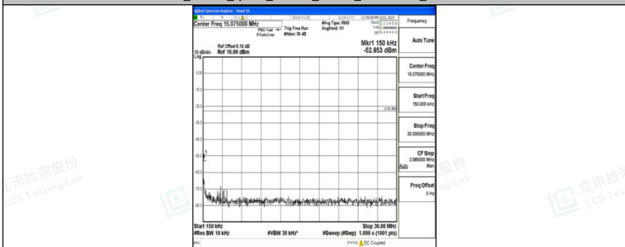
Band71_10MHz_QPSK_133422_1RB#0_0.15~30_0.15~30
