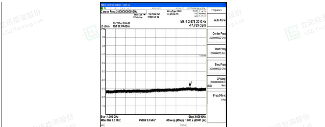
Band71_10MHz_16QAM_133297_1RB#0_1000~3000_1000~3000
