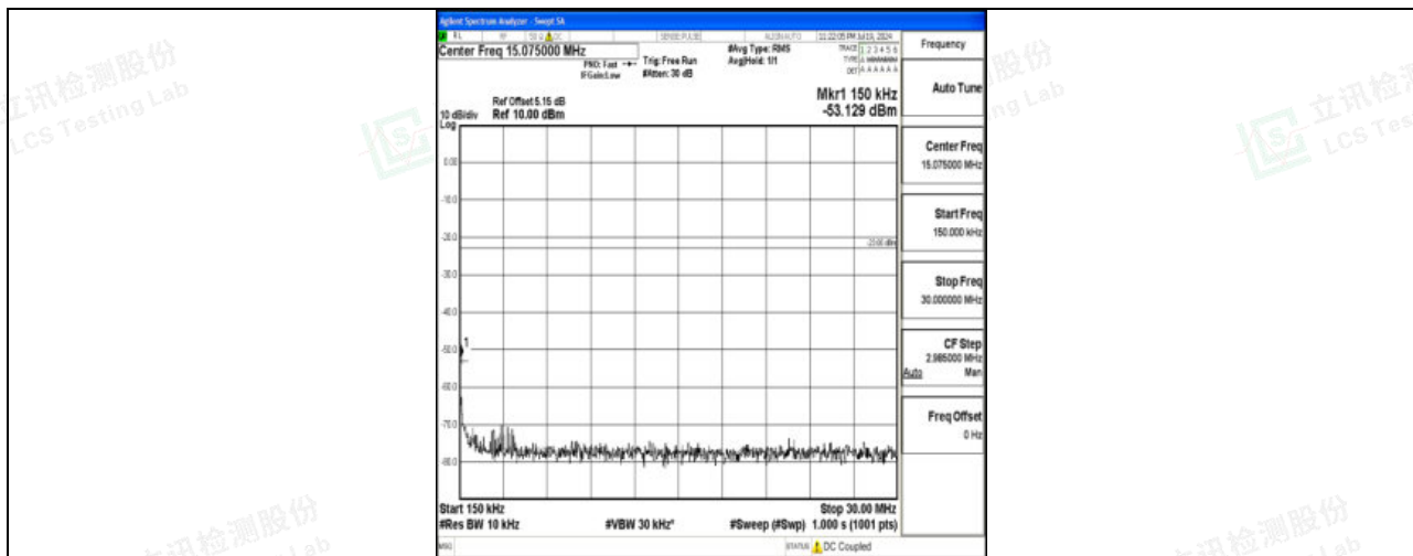
Band71_5MHz_16QAM_133147_1RB#0_0.15~30_0.15~30
