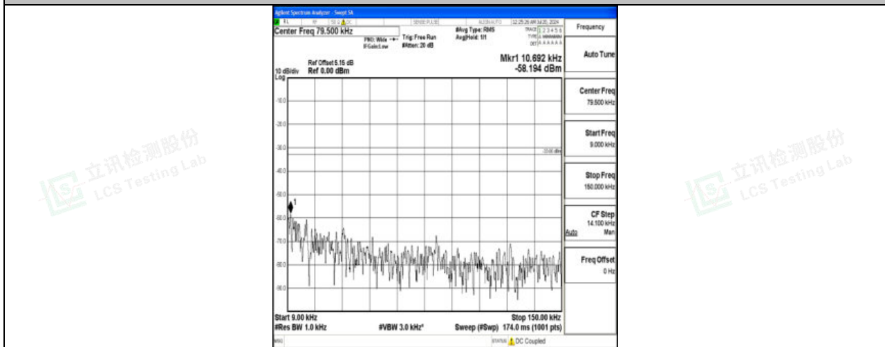
Band71_15MHz_QPSK_133397_1RB#0_0.009~0.15_0.009~0.15
