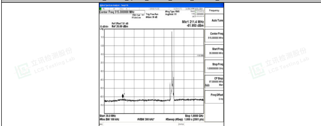
Band71_10MHz_QPSK_133422_1RB#0_30~1000_30~1000
