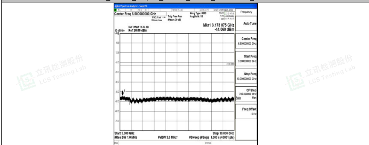
Band71_15MHz_16QAM_133397_1RB#0_3000~10000_3000~10000
