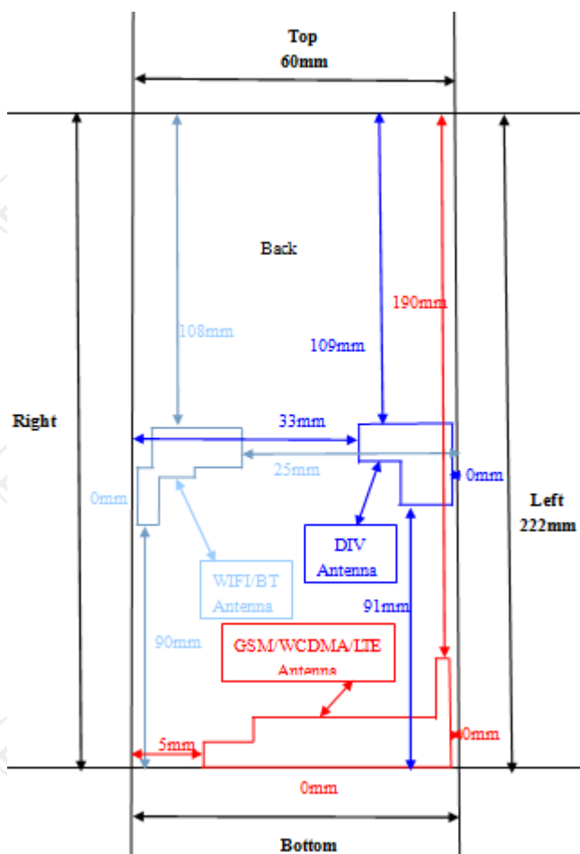
Antenna Configuration - open
