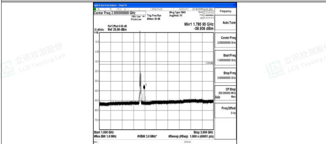
Band66_10MHz_QPSK_132022_1RB#0_1000~3000_1000~3000
