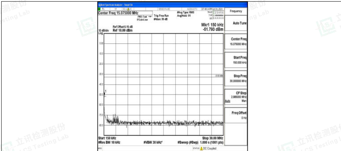
Band66_10MHz_QPSK_132022_1RB#0_0.15~30_0.15~30
