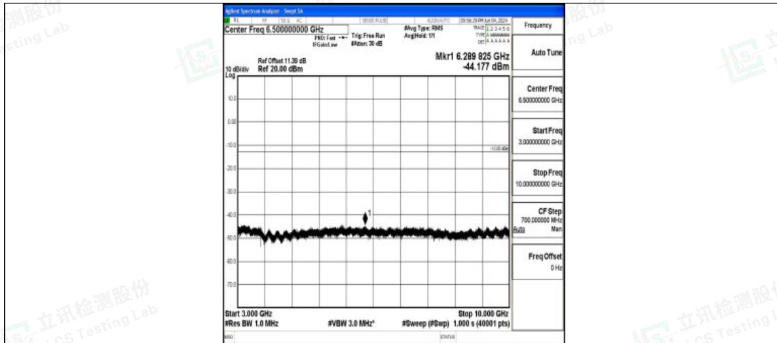
Band71_20MHz_QPSK_133322_1RB#0_3000~10000_3000~10000
