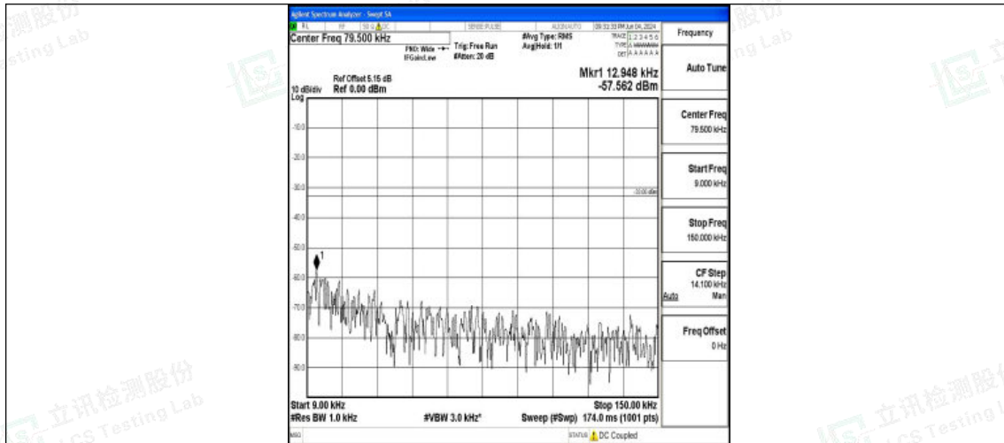
Band71_15MHz_16QAM_133197_1RB#0_0.009~0.15_0.009~0.15
