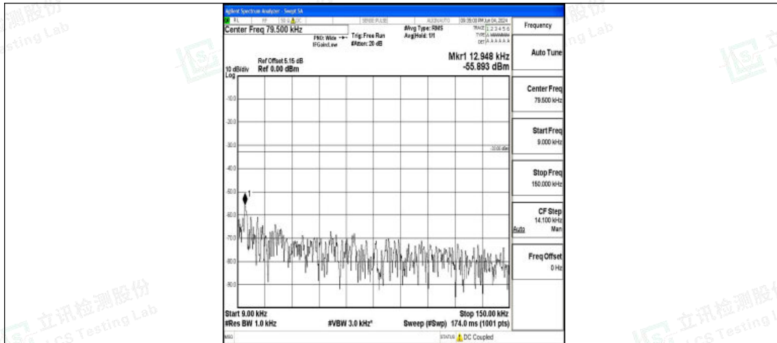
Band71_15MHz_QPSK_133397_1RB#0_0.009~0.15_0.009~0.15
