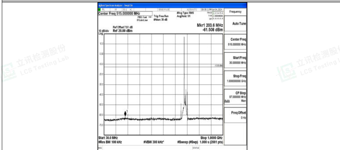
Band71_15MHz_QPSK_133397_1RB#0_30~1000_30~1000
