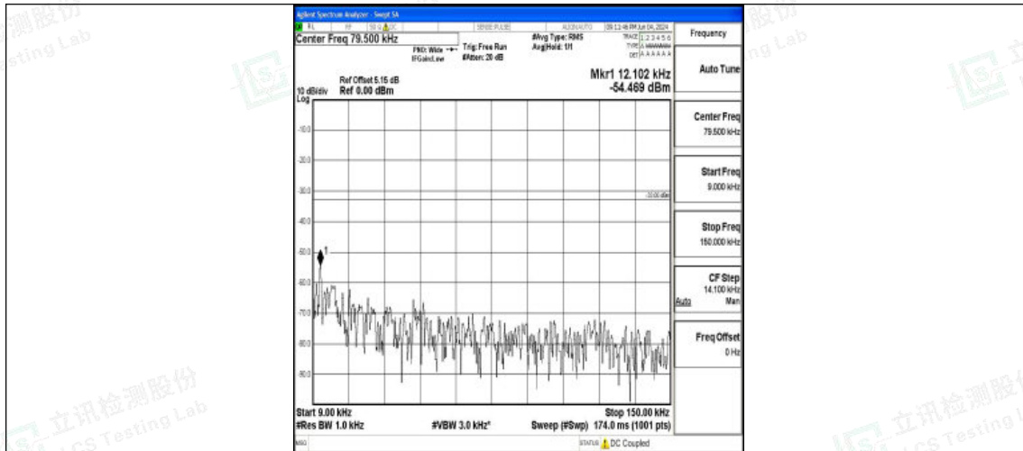
Band71_10MHz_QPSK_133422_1RB#0_0.009~0.15_0.009~0.15
