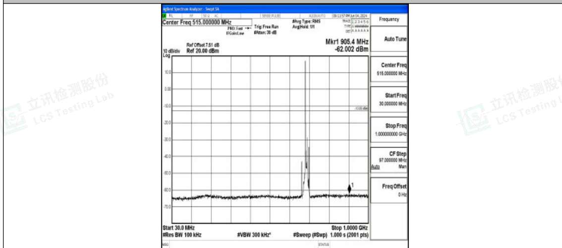
Band71_10MHz_QPSK_133422_1RB#0_30~1000_30~1000
