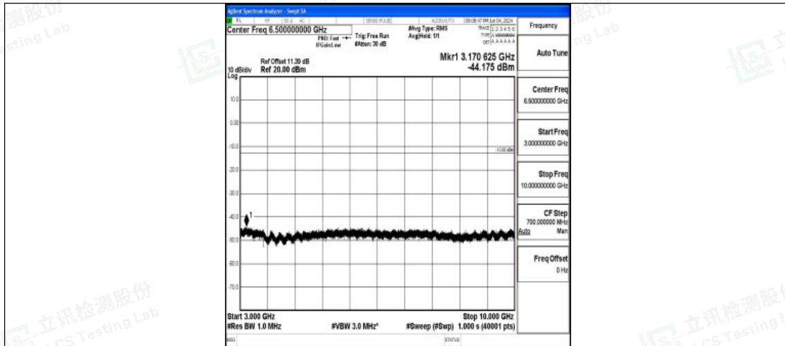
Band71_10MHz_16QAM_133172_1RB#0_3000~10000_3000~10000
