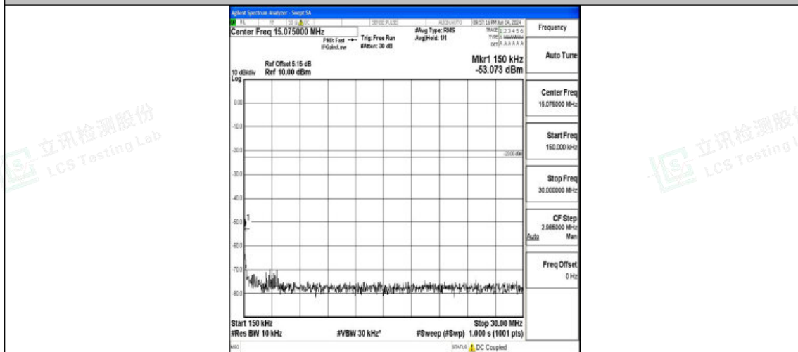
Band71_20MHz_16QAM_133322_1RB#0_0.15~30_0.15~30
