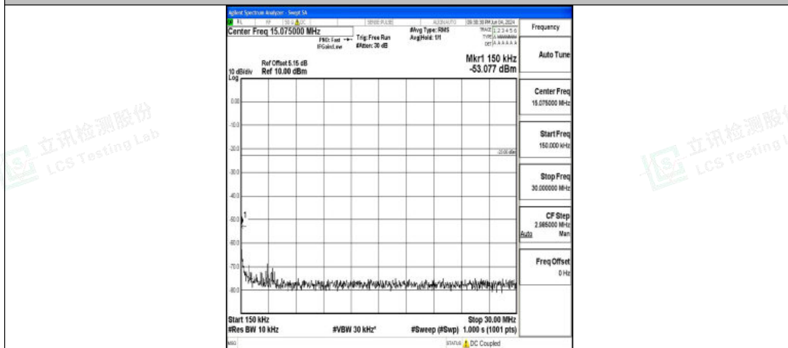
Band71_15MHz_QPSK_133197_1RB#0_0.15~30_0.15~30
