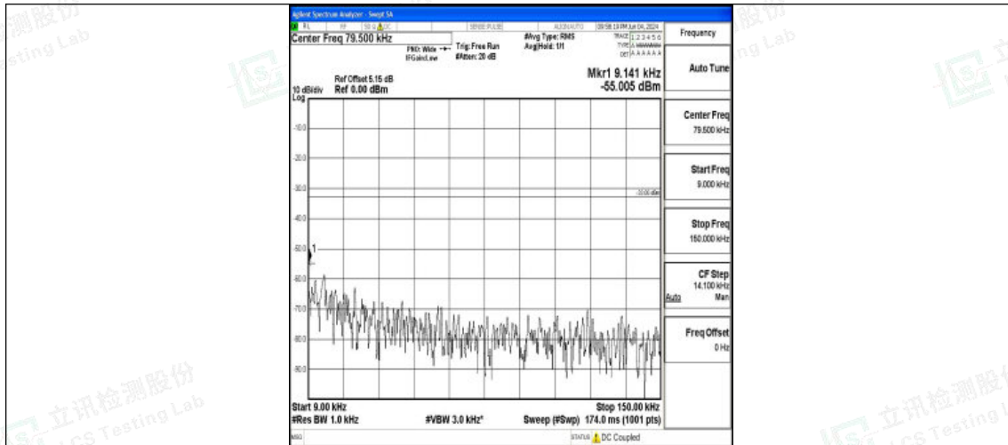
Band71_20MHz_QPSK_133372_1RB#0_0.009~0.15_0.009~0.15
