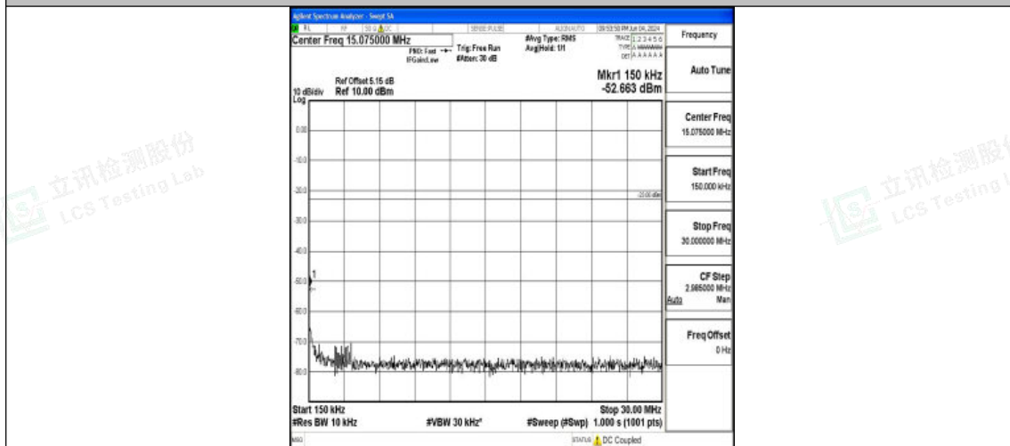
Band71_20MHz_QPSK_133222_1RB#0_0.15~30_0.15~30
