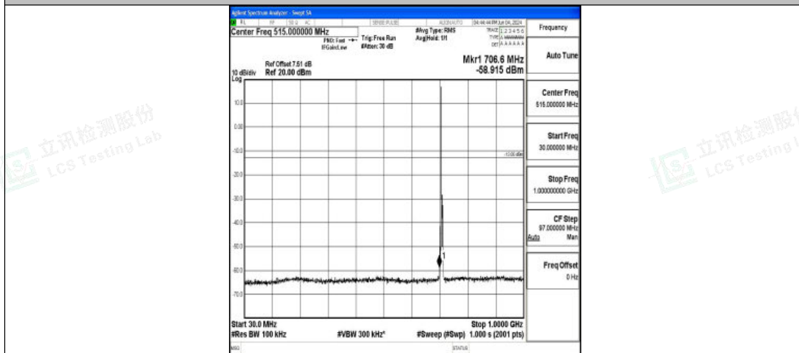
Band12_3MHz_QPSK_23165_1RB#0_30~1000_30~1000
