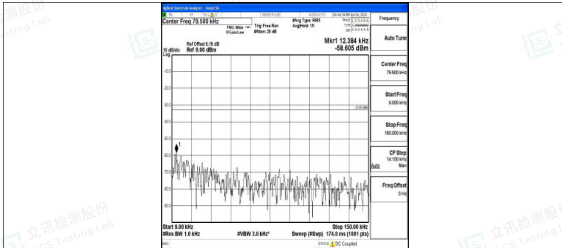
Band12_3MHz_QPSK_23165_1RB#0_0.009~0.15_0.009~0.15
