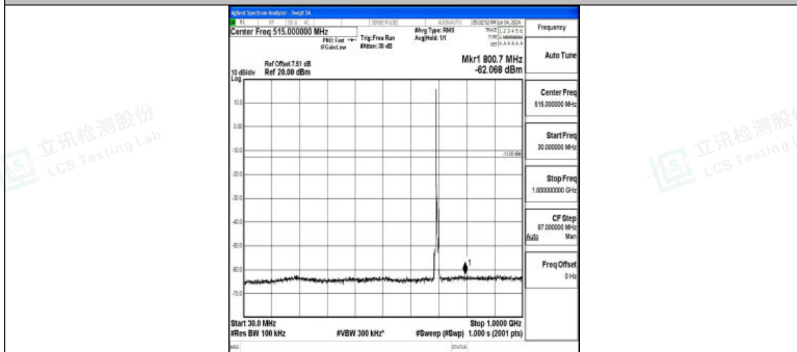
Band12_5MHz_16QAM_23035_1RB#0_30~1000_30~1000
