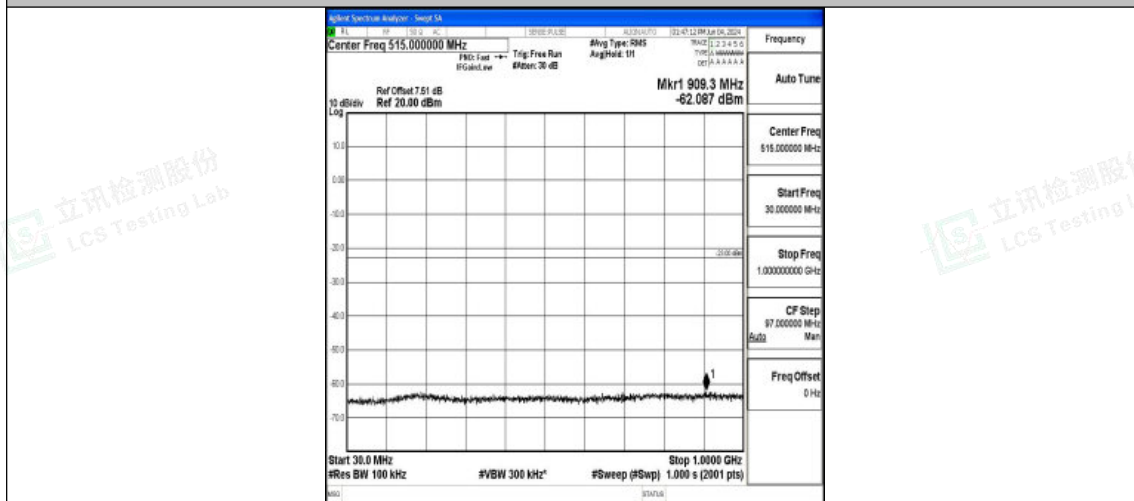
Band4_5MHz_QPSK_20175_1RB#0_30~1000_30~1000
