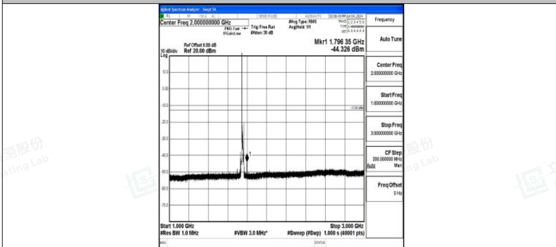
Band4_10MHz_QPSK_20350_1RB#0_1000~3000_1000~3000
