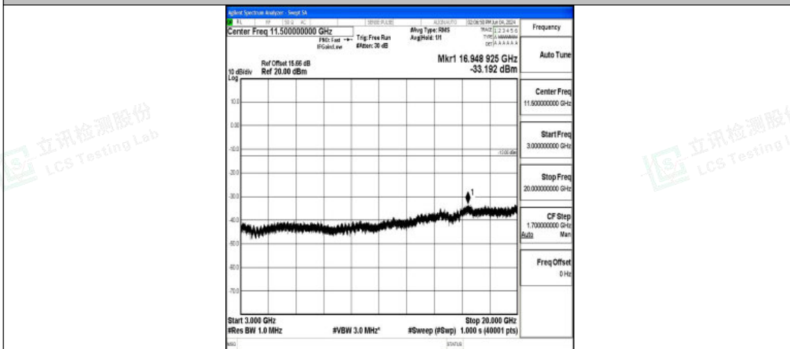
Band4_10MHz_QPSK_20350_1RB#0_3000~20000_3000~20000
